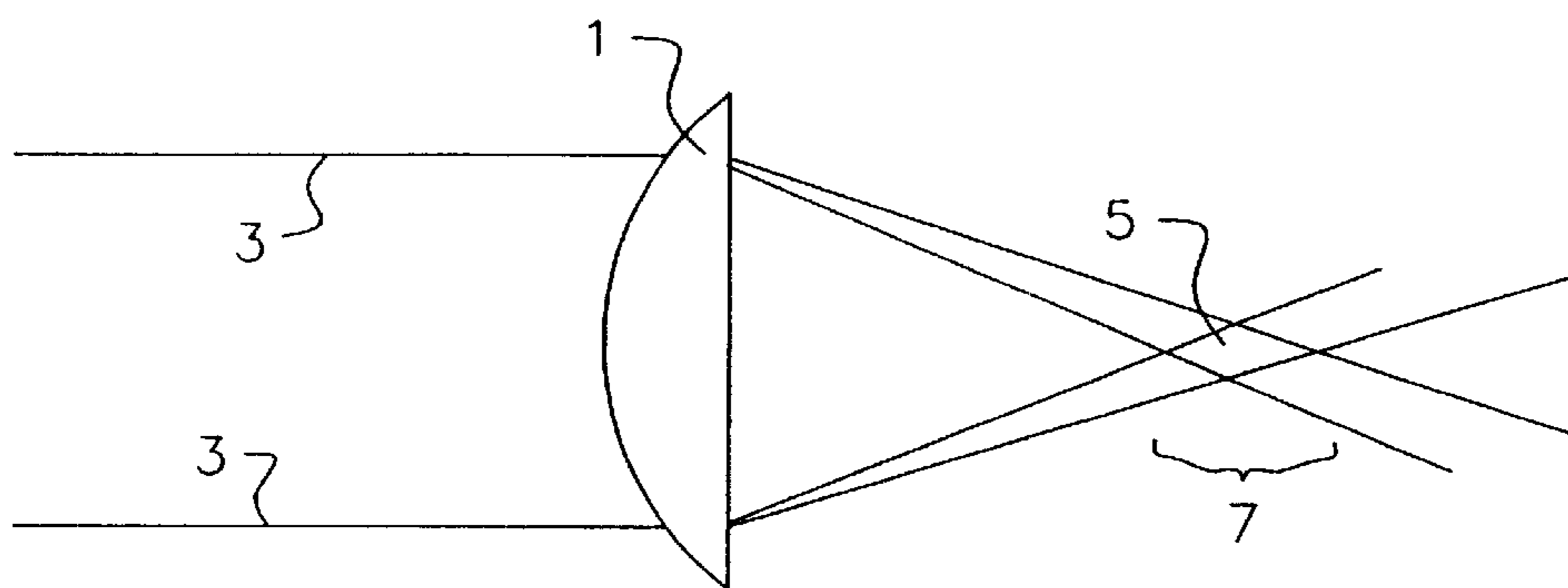
FIG. 1 PRIOR ART
