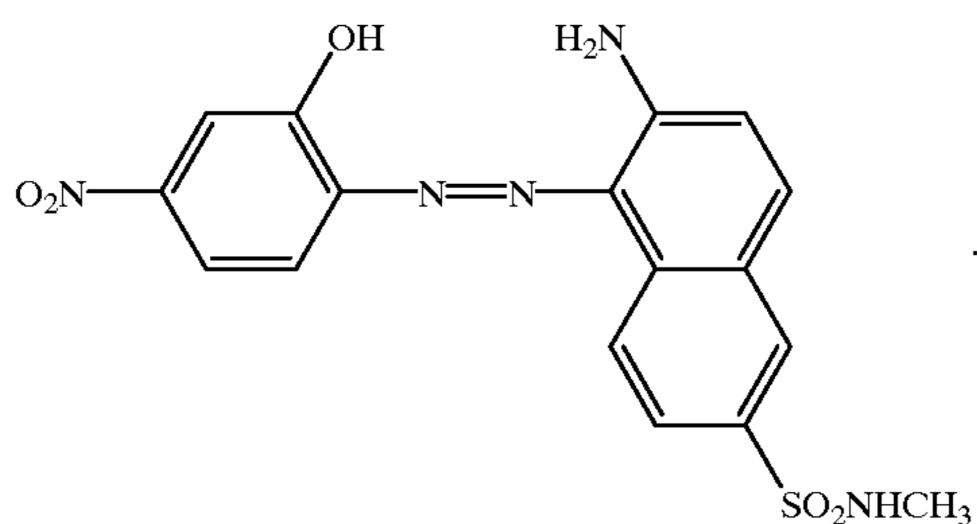
1:2 cobalt complex
