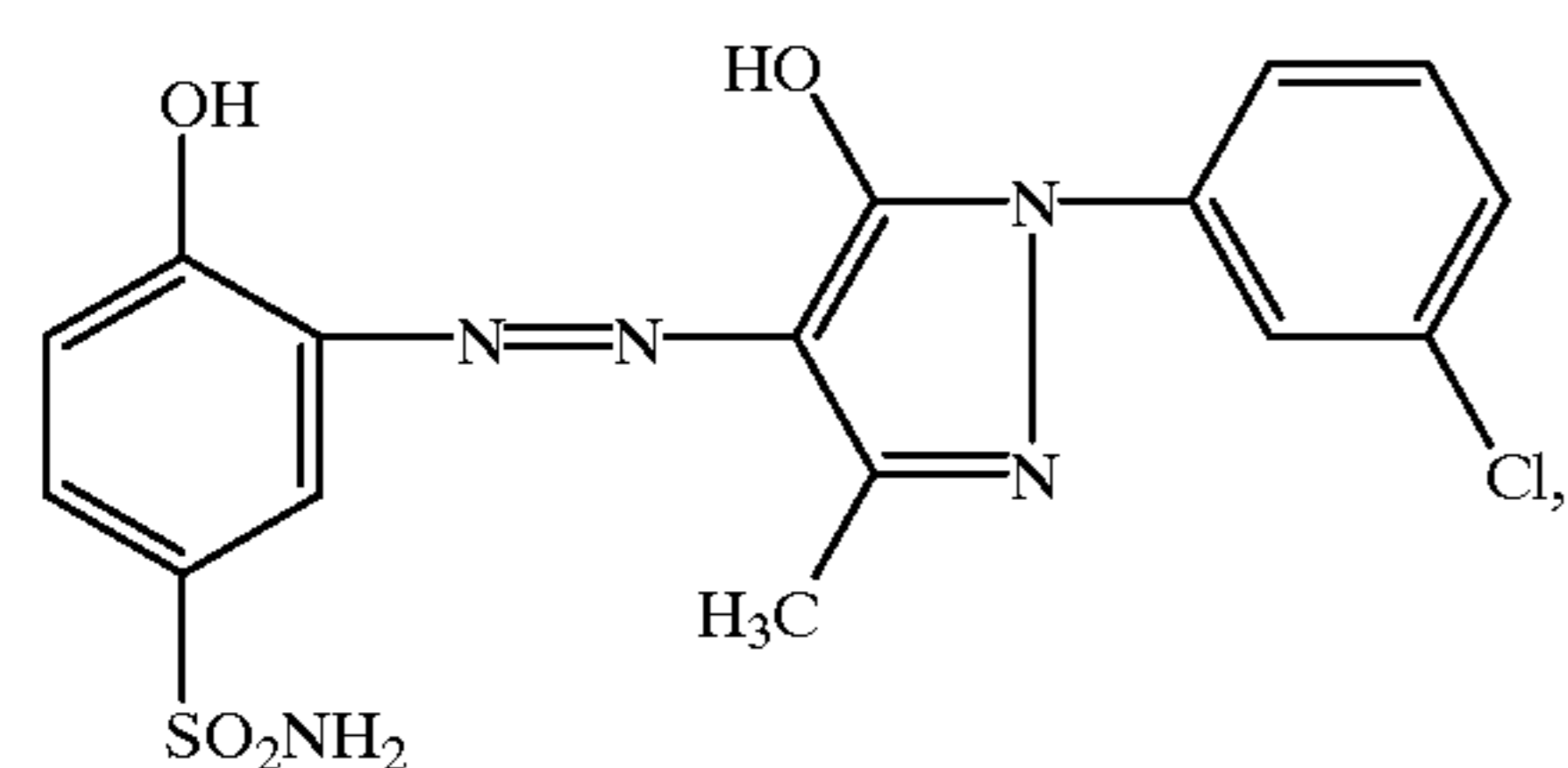
1:2 cobalt complex
