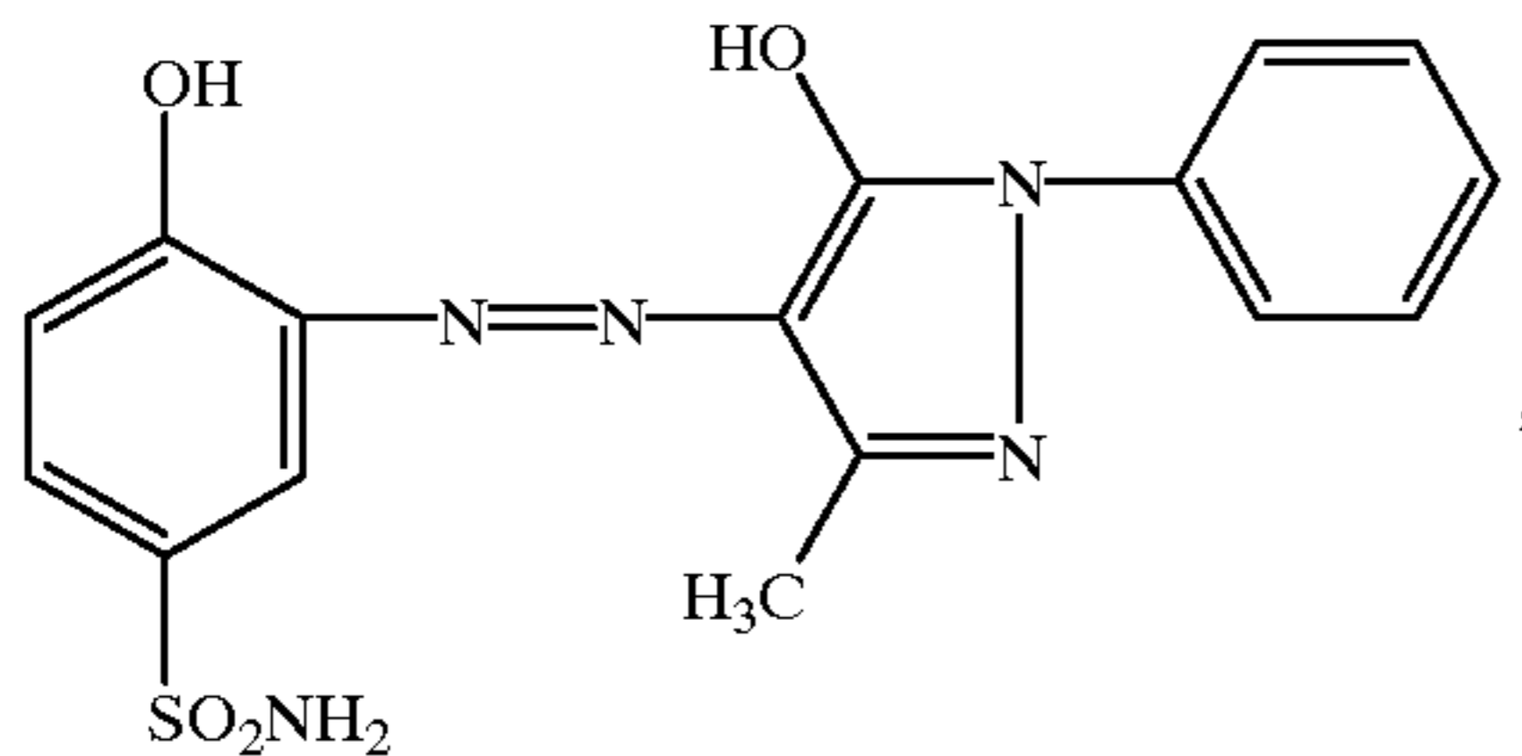
1:2 cobalt complex
