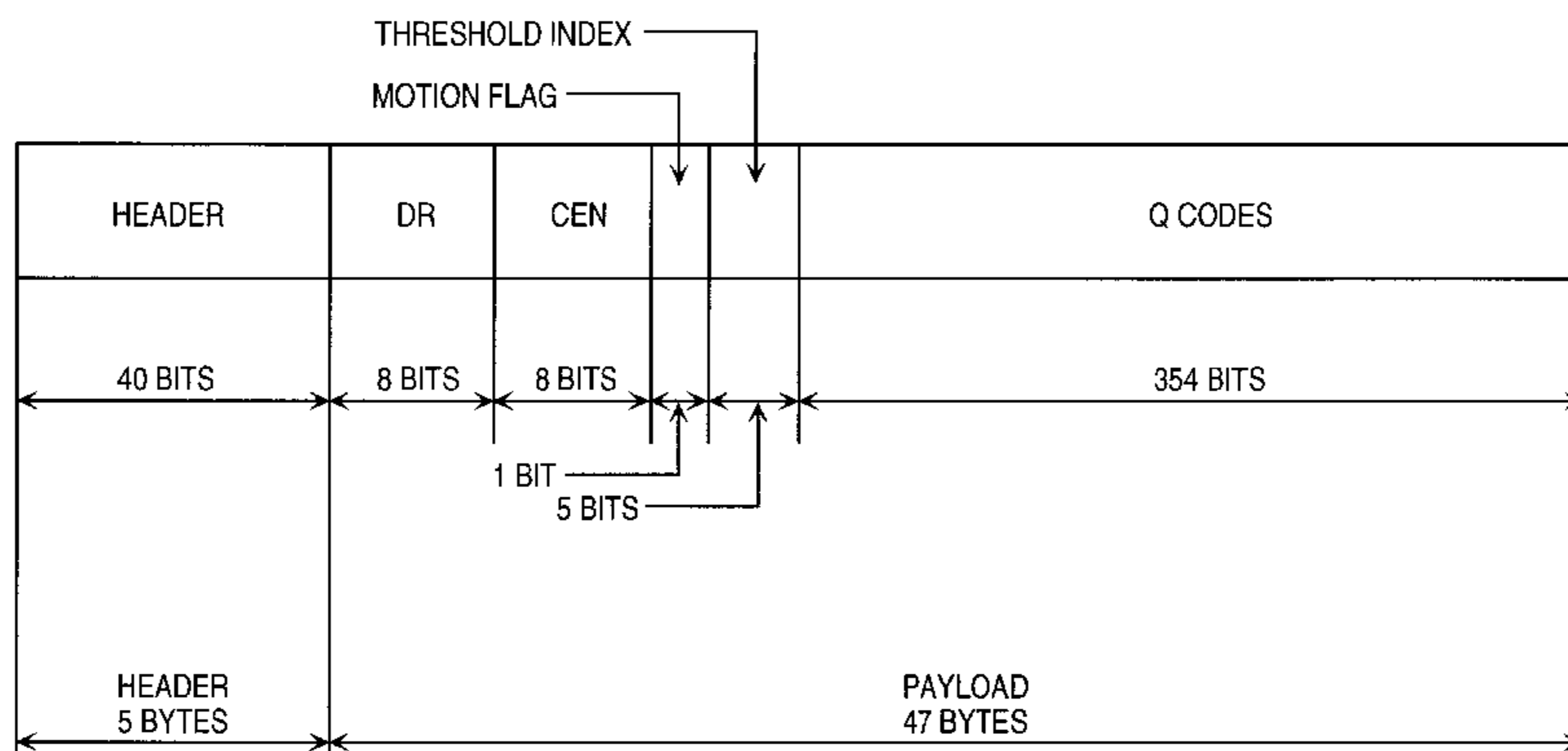
PACKET STRUCTURE 300
