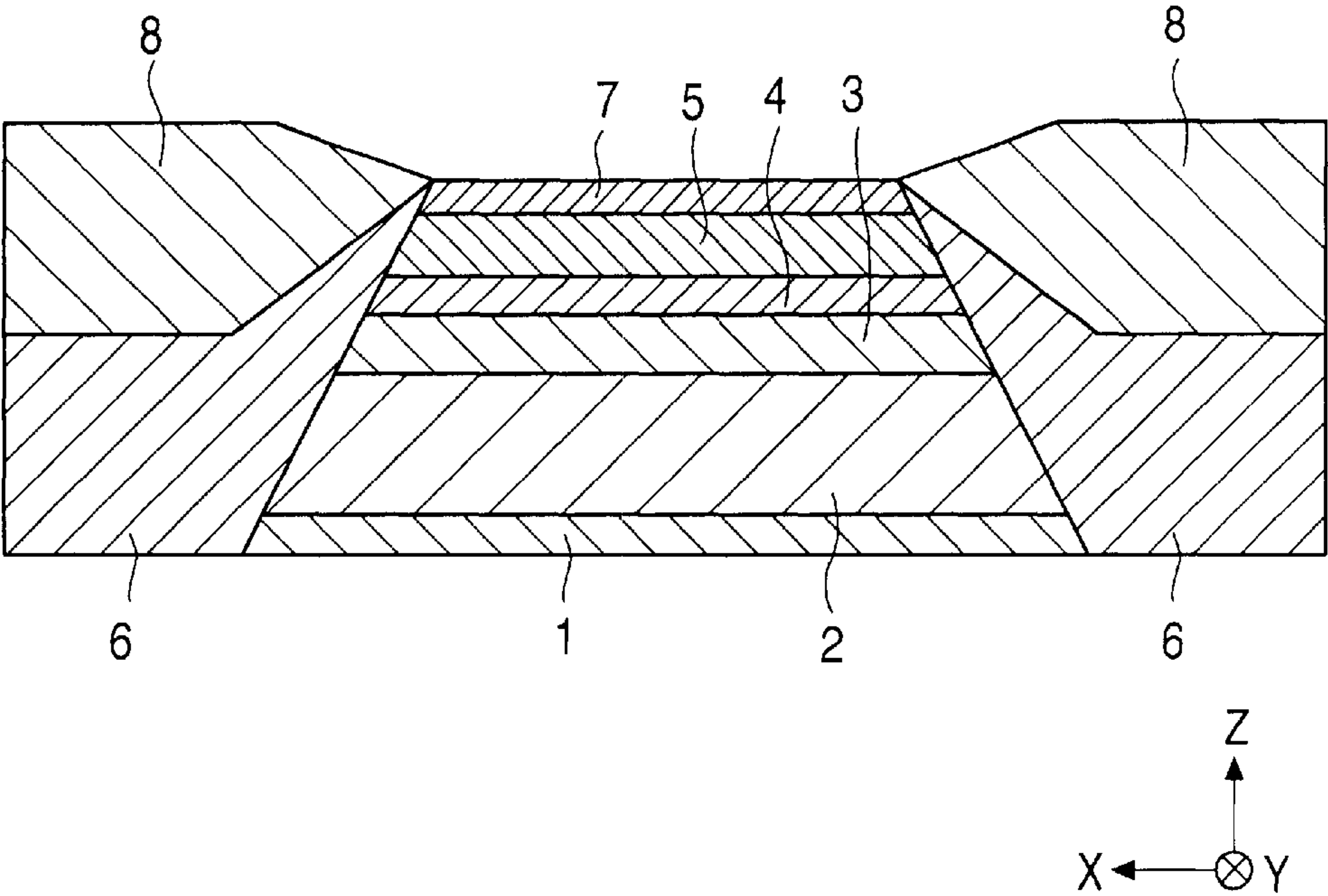
FIG. 28 PRIOR ART
