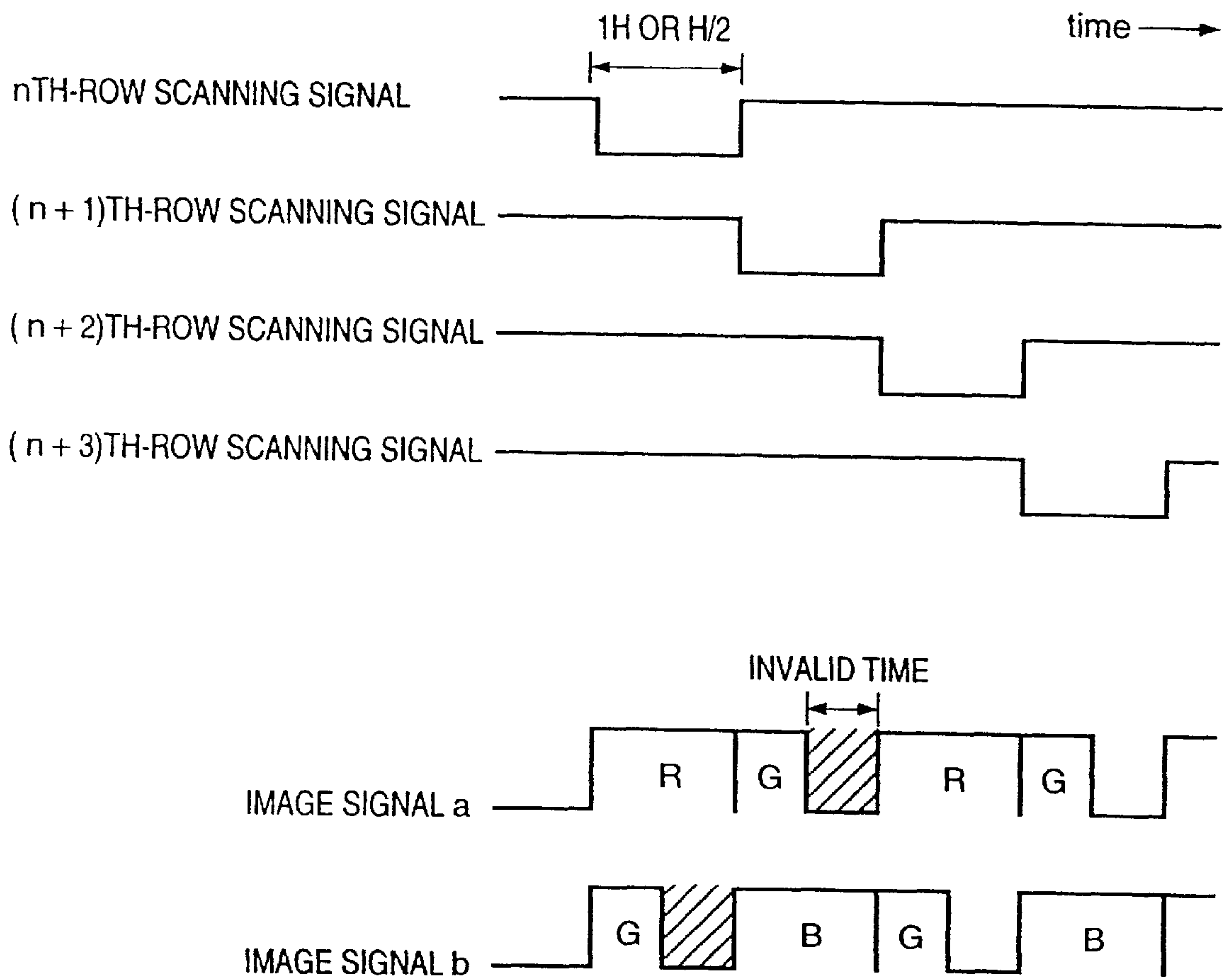
FIG. 6 PRIOR ART
