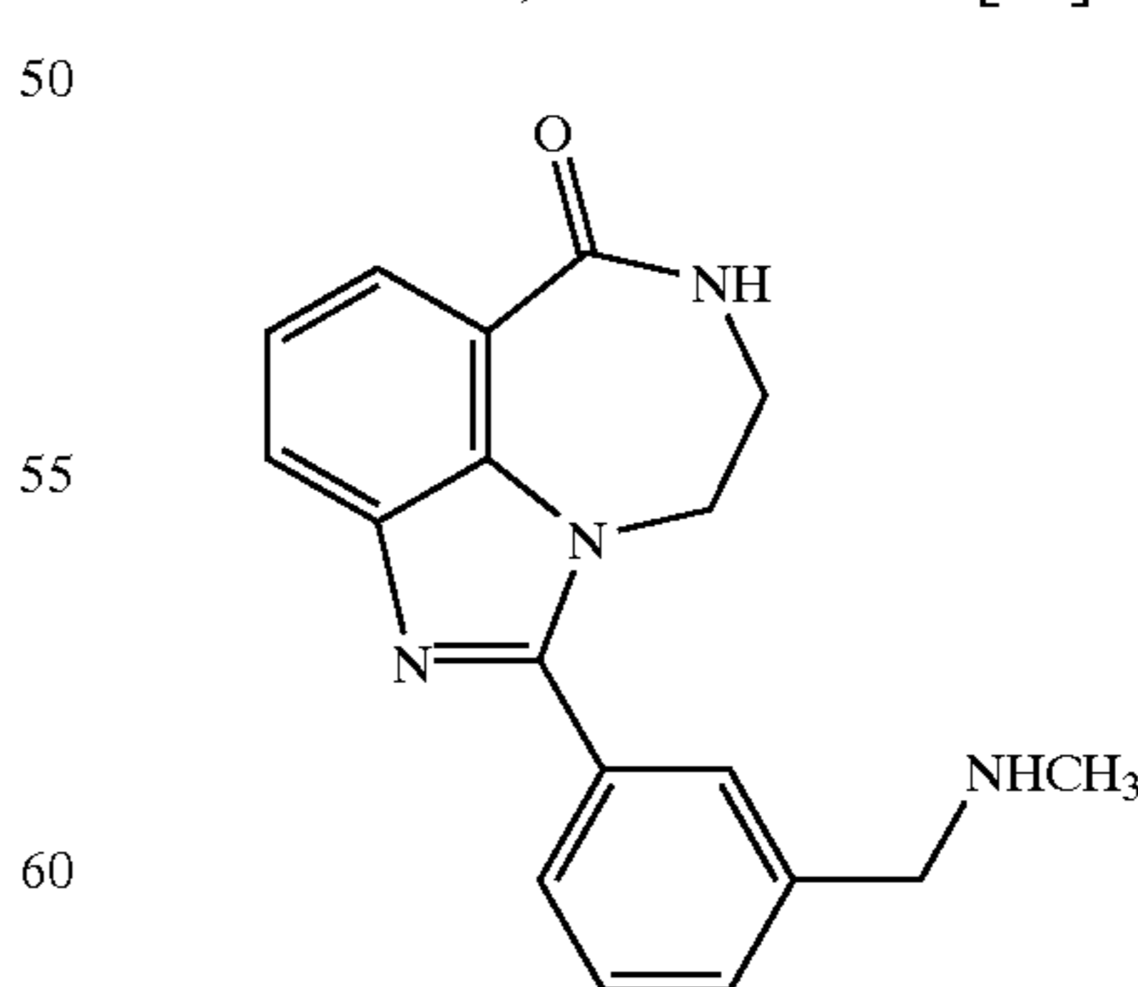
1-(3-Methylaminomethyl-phenyl)-8,9-dihydro-7H-2,7,9a-triaza-benzo[cd]azulen-6-one
