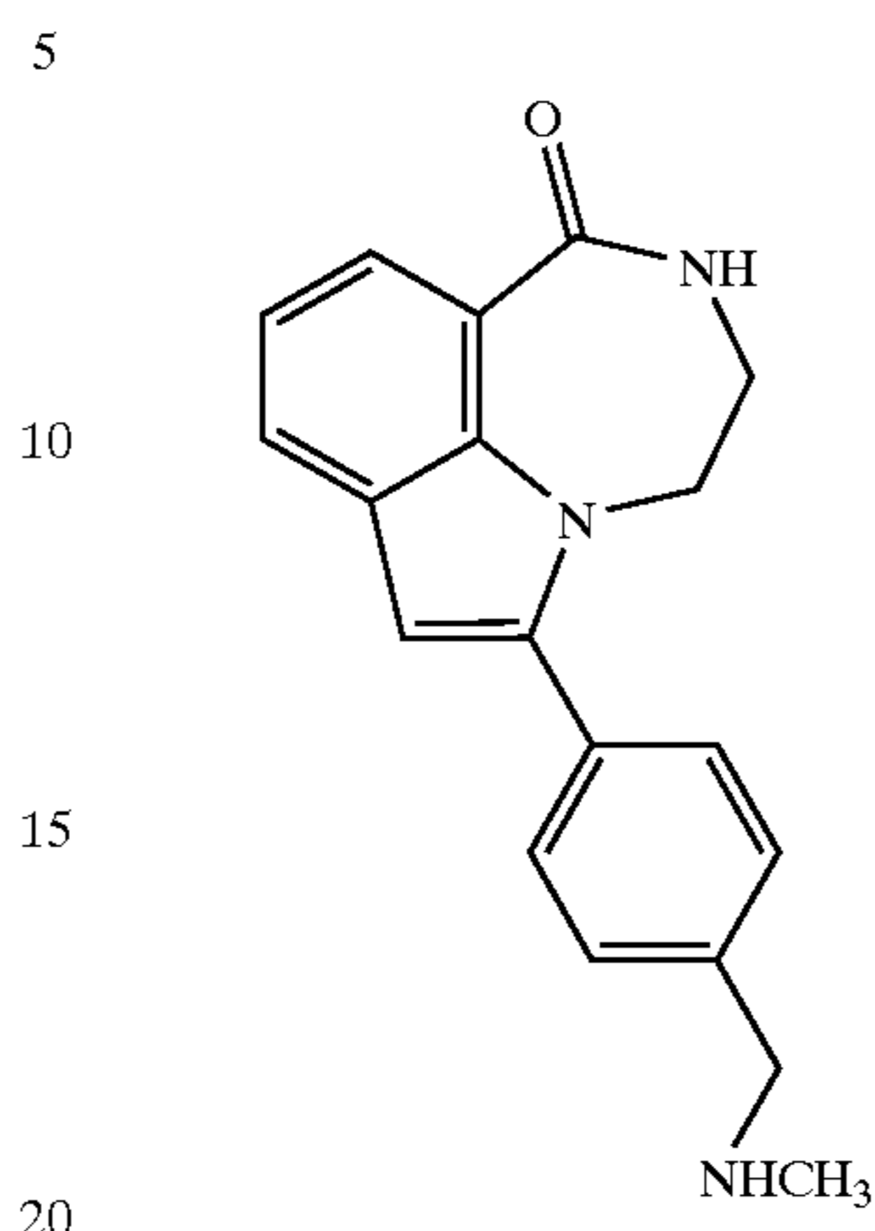
6-(4-Methylaminomethyl-phenyl)-3,4-dihydro-2H-[1,4]diazepino[6,7,1-hi]indol-1-one
