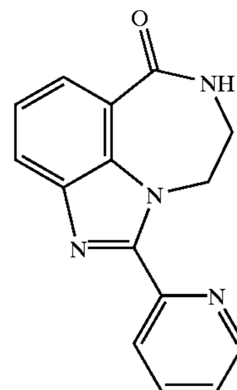
1-Pyridin-2-yl-8,9-dihydro-7H-2,7,9a-triaza-benzo[cd]azulen-6-one
