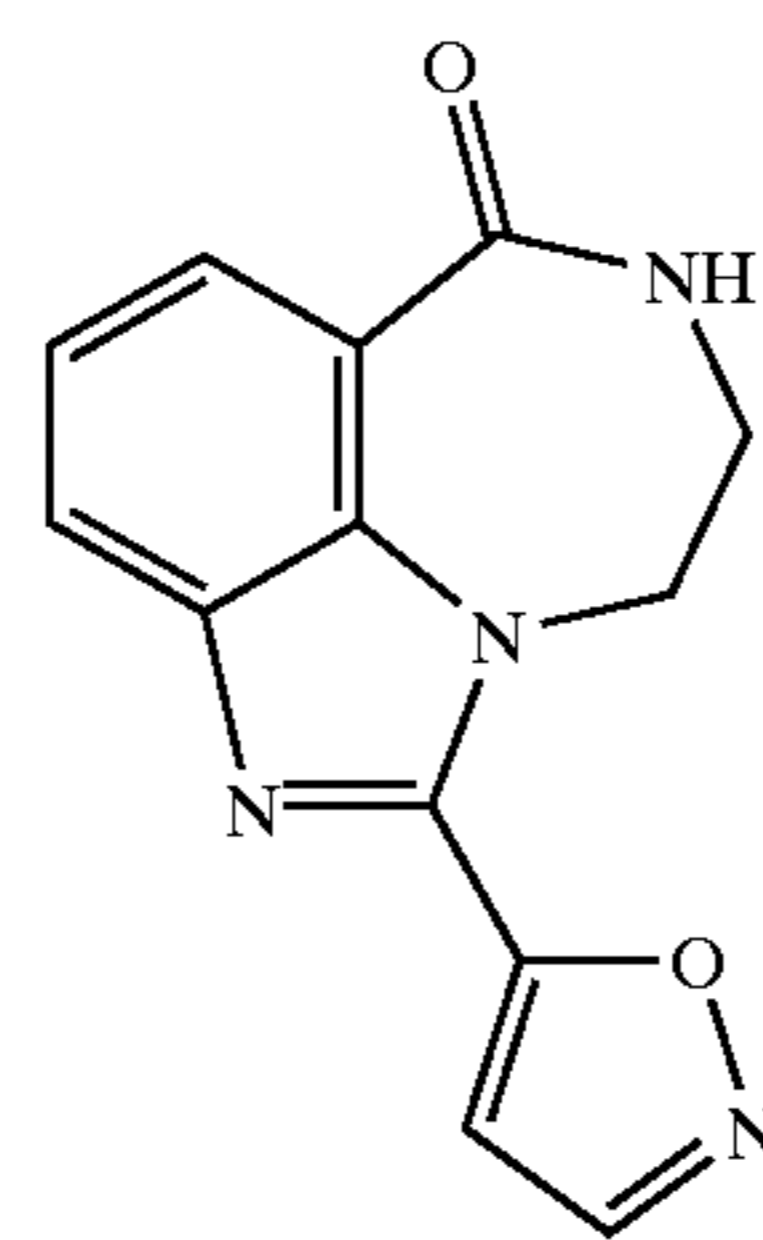
1-Isioxazol-5-yl-8,9-dihydro-7H-2,7,9a-triaza-benzo[cd]azulen-6-one
