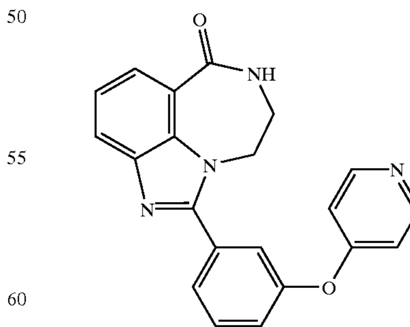
1-[3-(Pyridin-4-yloxy)-phenyl]-8,9-dihydro-7H-2,7,9a-triaza-benzo[cd]azulen-6-one
