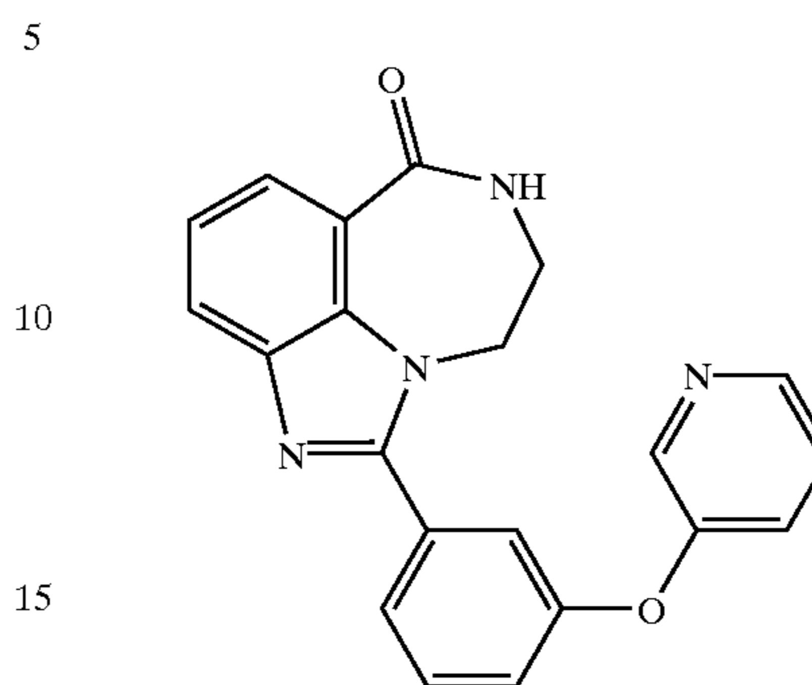
1-[3-(Pyridin-3-yloxy)-phenyl]-8,9-dihydro-7H-2,7,9a-triaza-benzo[cd]azulen-6-one
