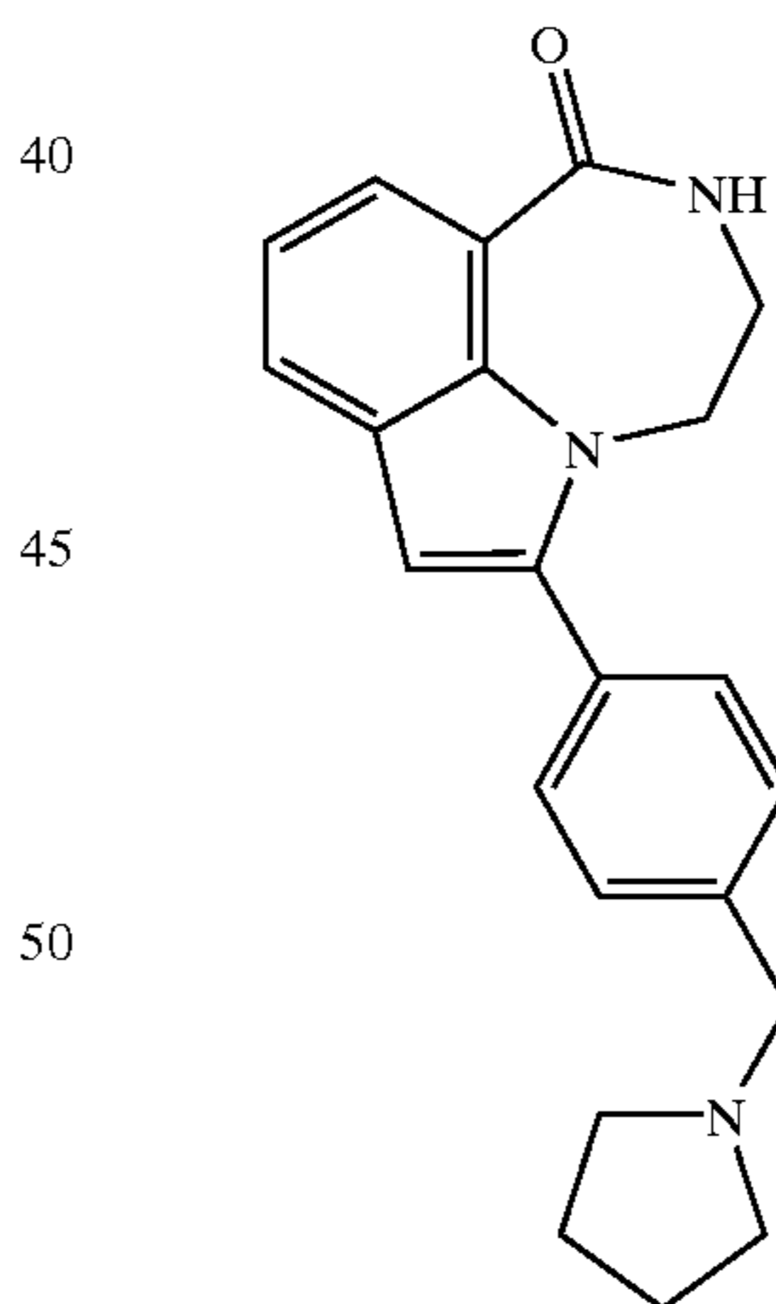
6-(4-Pyrrolidin-1-ylmethyl-phenyl)-3,4-dihydro-2H-[1,4]diazepino[6,7,1-hi]indol-1-one
