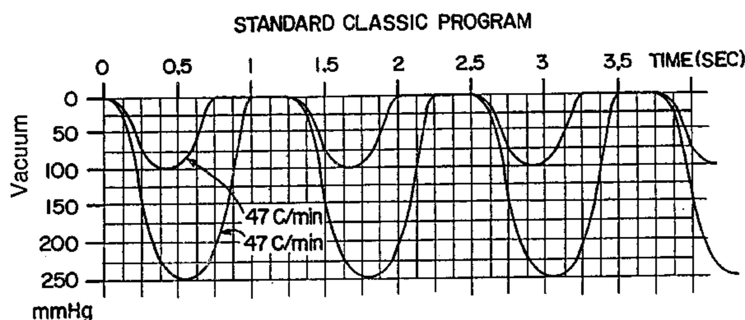
SUCTION CURVES AND CYCLES EQUAL TO CLASSIC VACUUM RANGE: 100 - 250mmHg CYCLES: 47/min (NOT ADJUSTABLE)
