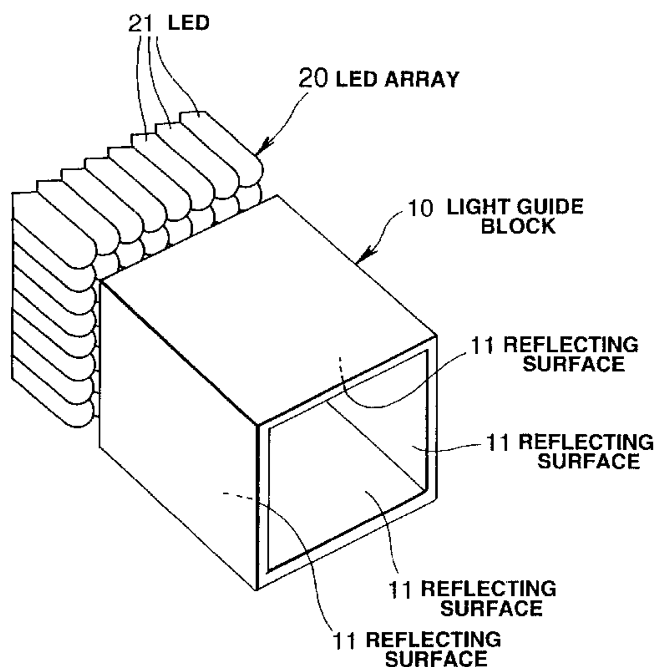
100 LIGHT SOURCE DEVICE
