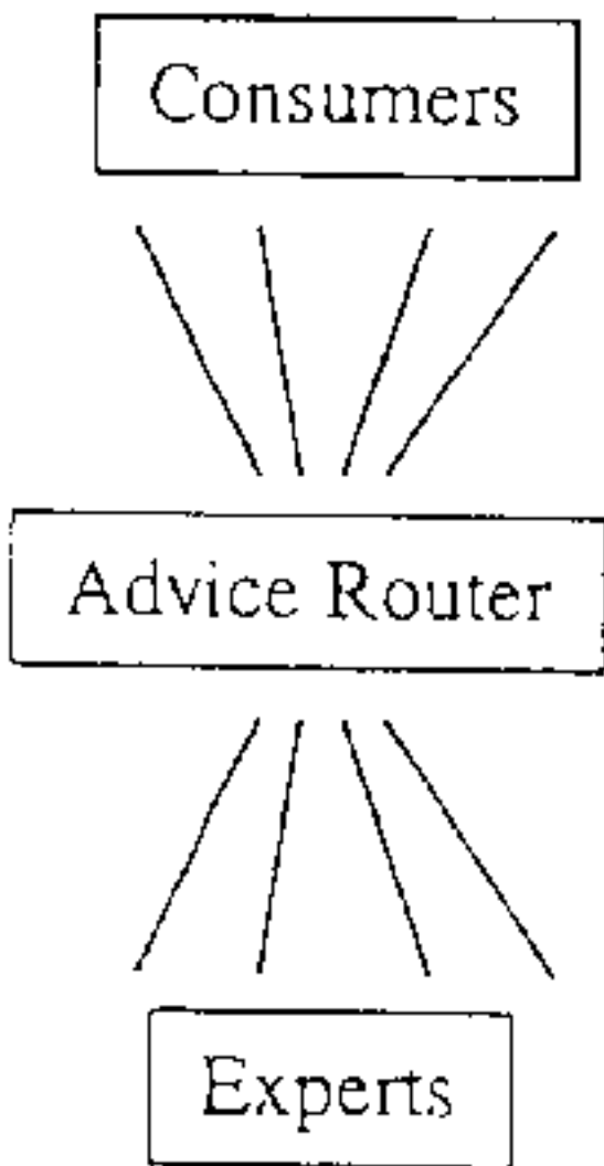
Information Flow:
