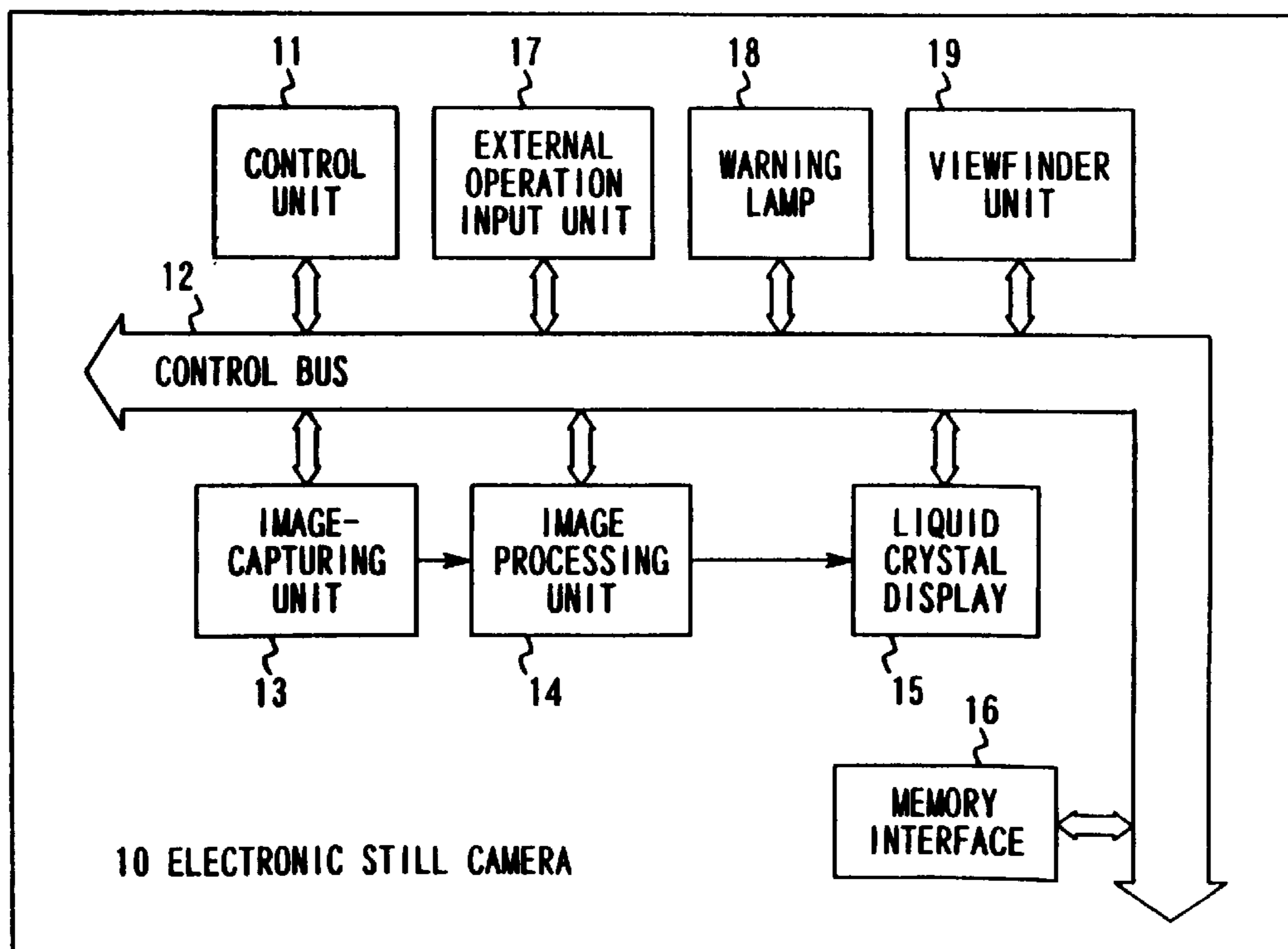
FUNCTIONAL BLOCK DIAGRAM OF ELECTRONIC STILL CAMERA
