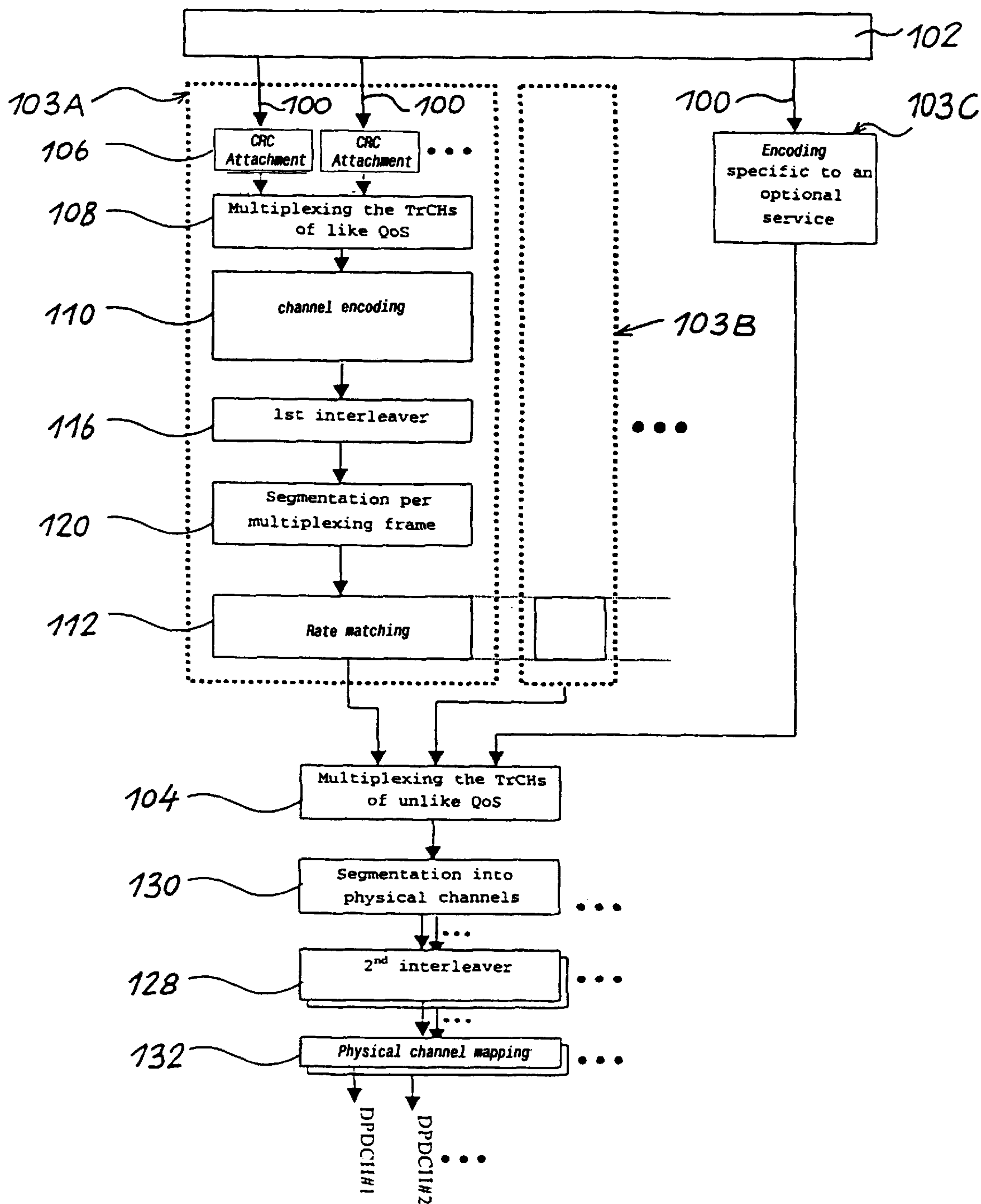
FIG. 2 PRIOR ART
