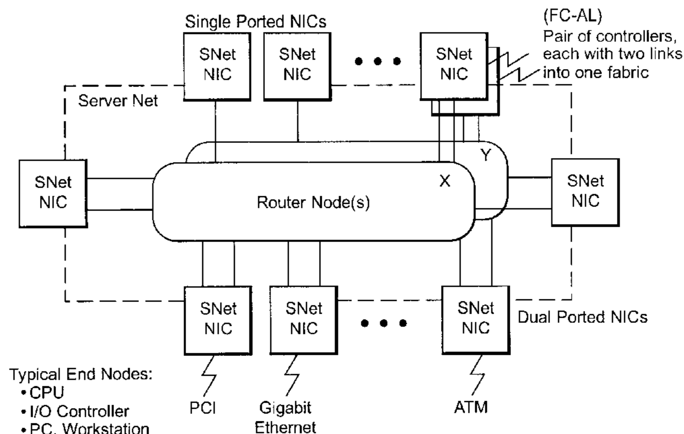
Fault Tolerant ServerNet II System Area Network
