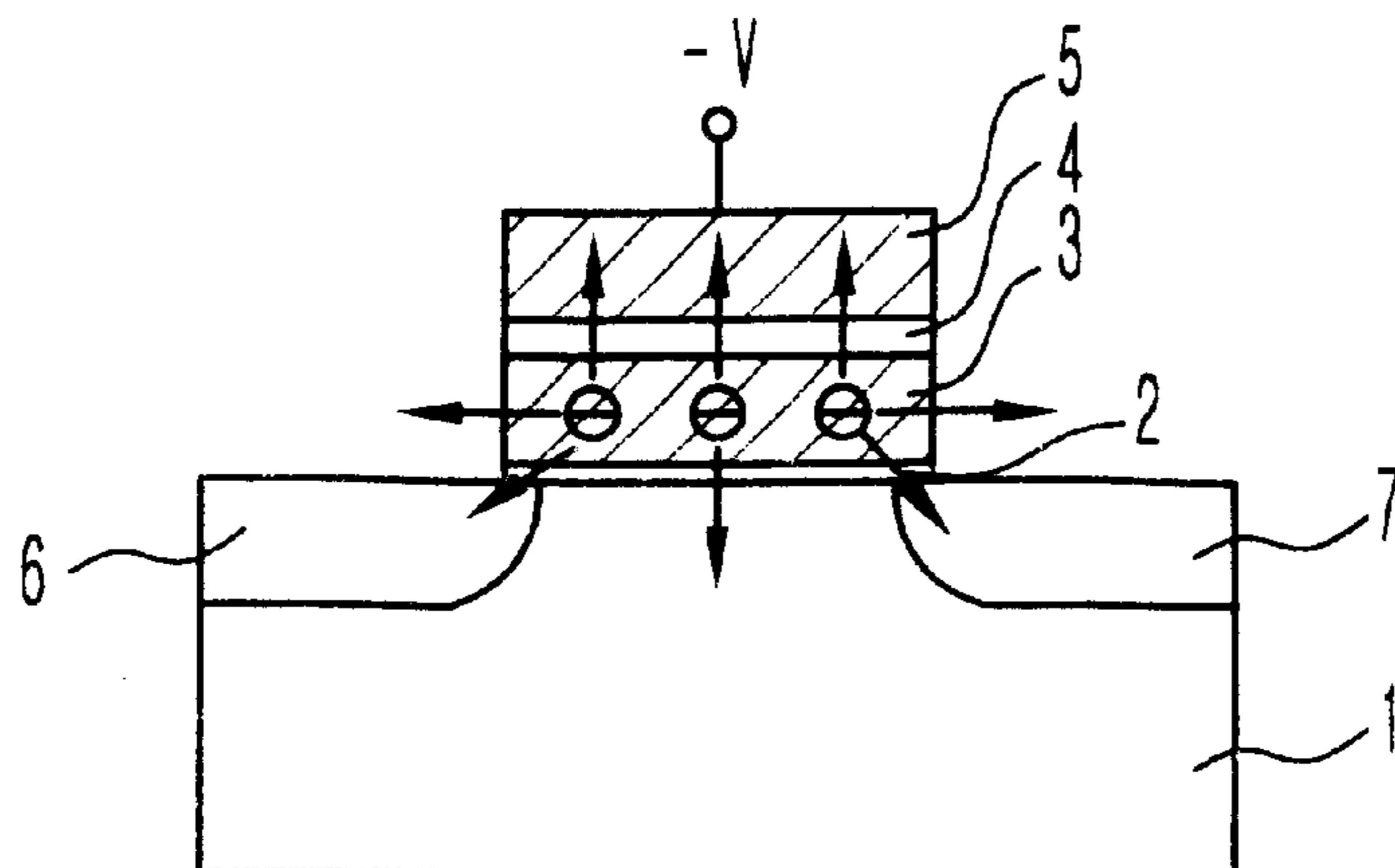
FIG. 4 (PRIOR ART)
