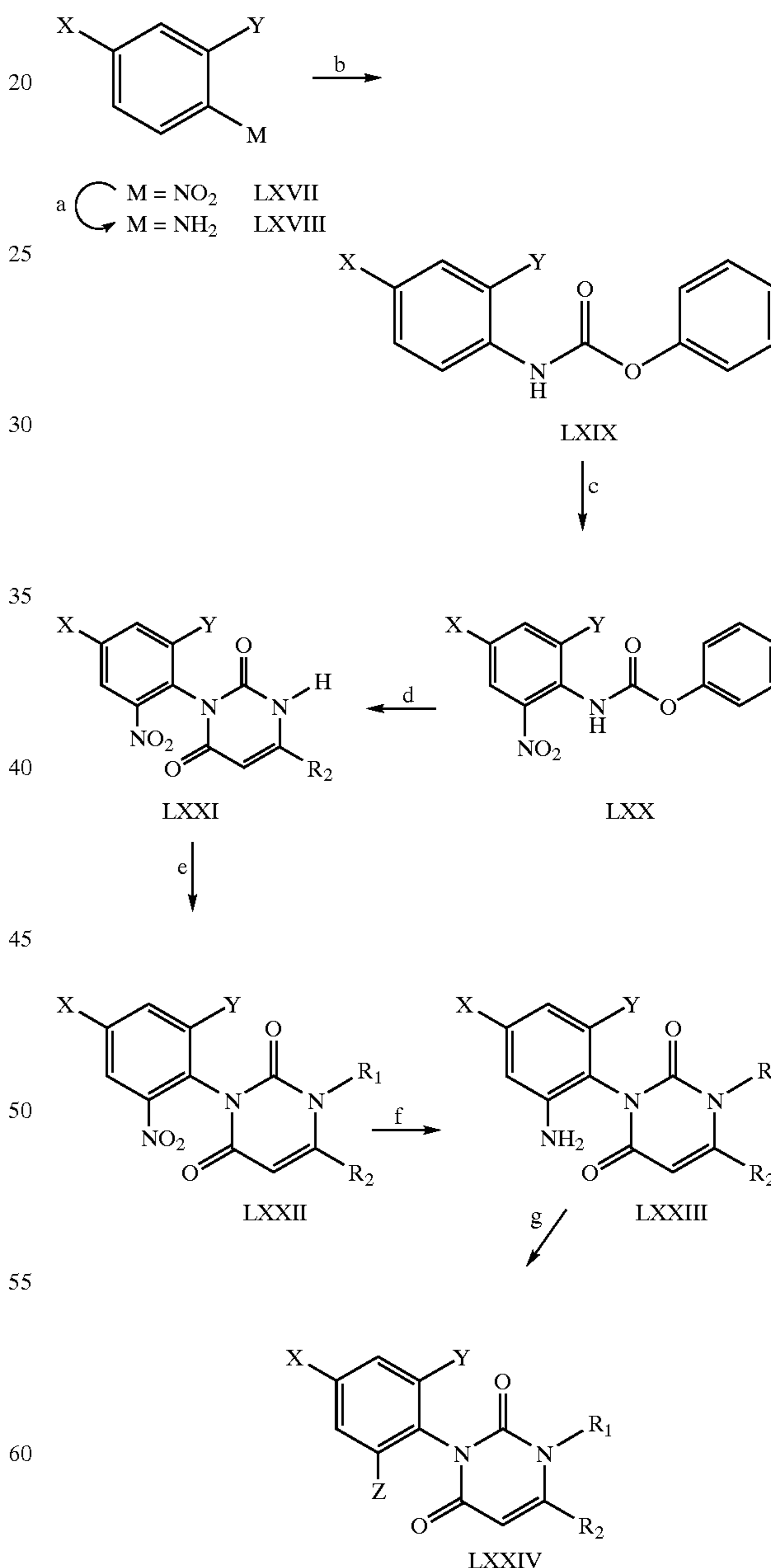
SCHEME 14
