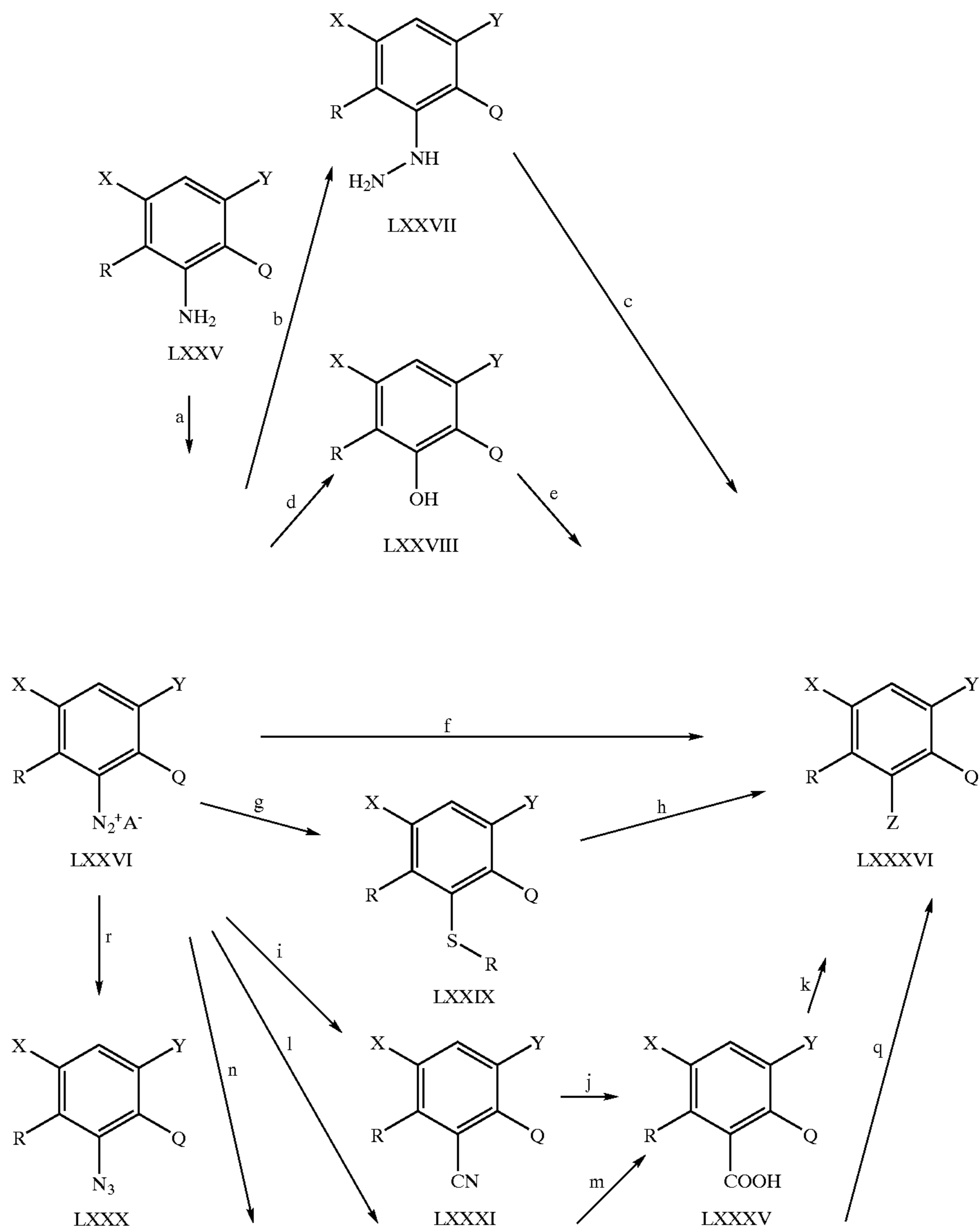
SCHEME 15
