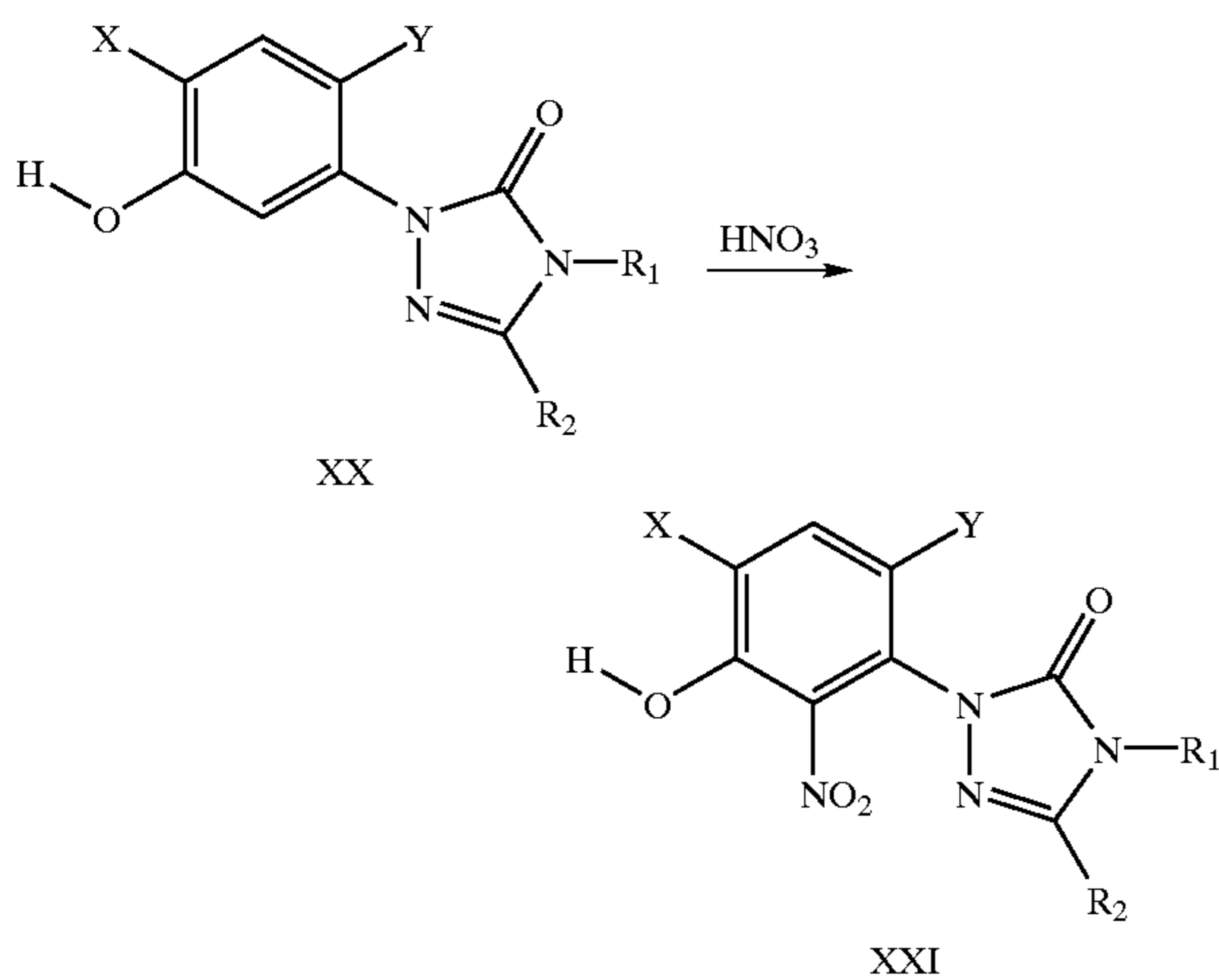
SCHEME 5
