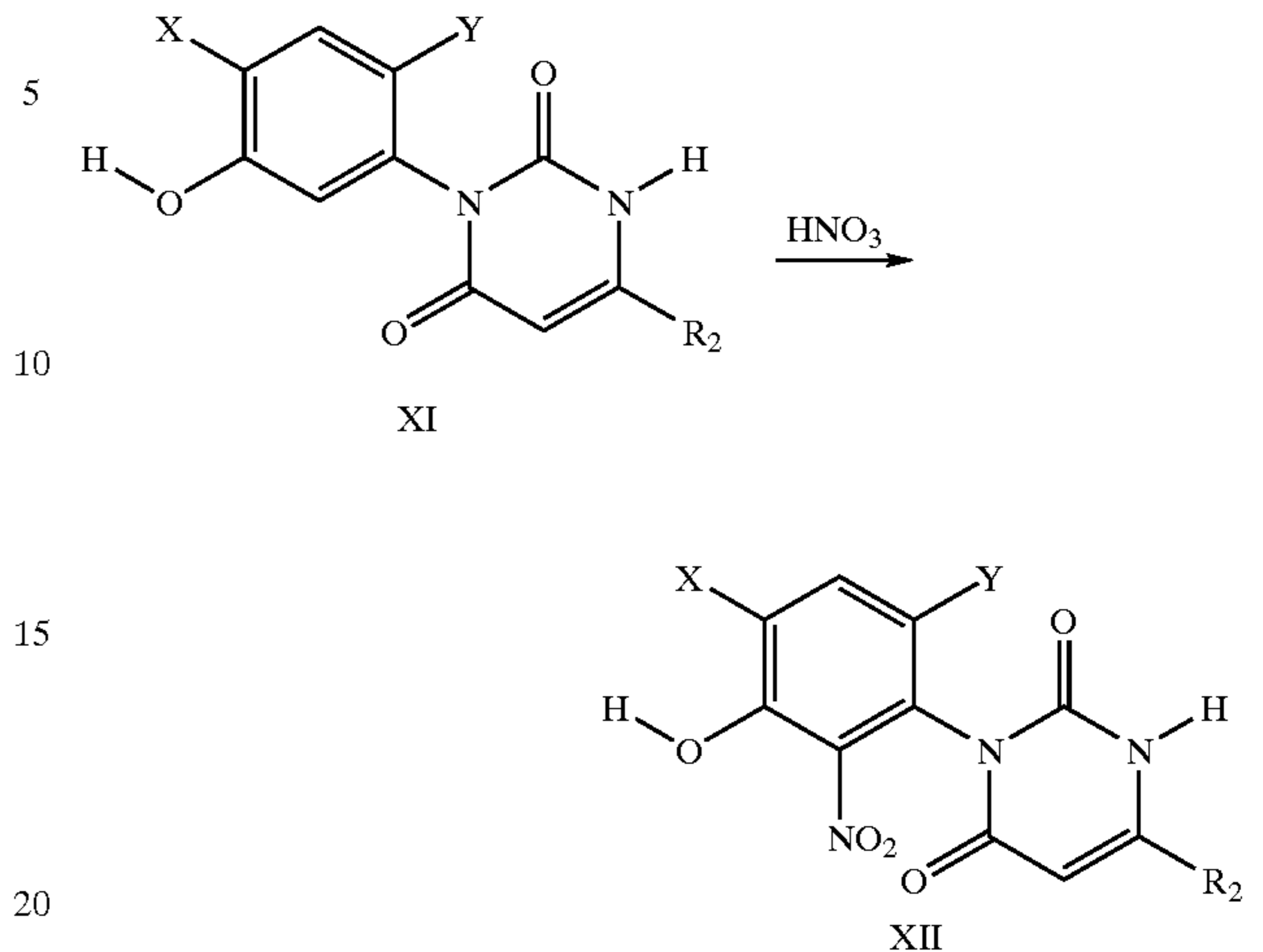
SCHEME 2
