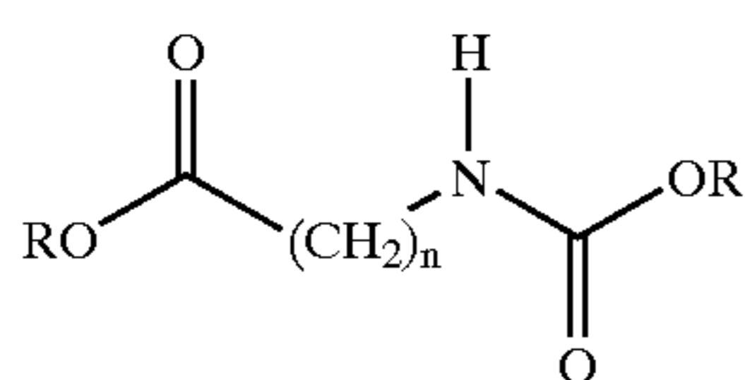
Compound A (n = 5, R = methyl) Compound B (n = 11, R = butyl)
