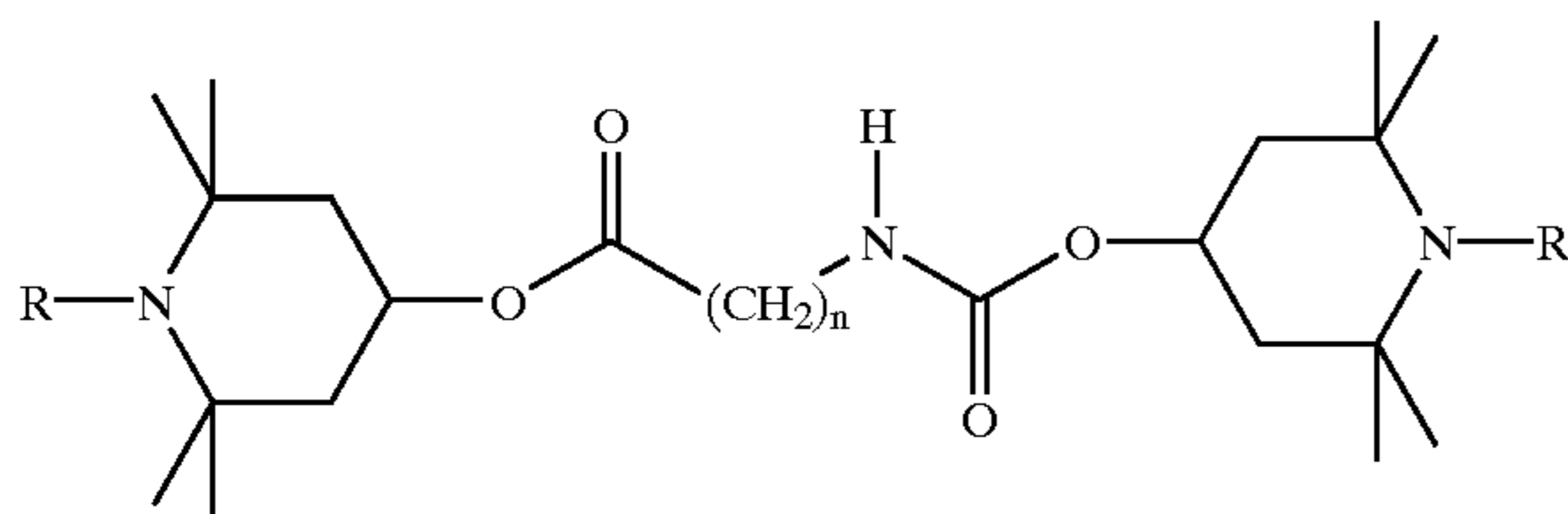
Compound I (n = 5, R = hydrogen) Compound II (n = 5, R = methyl) Compound III (n = 11, R = hydrogen) Compound IV (n = 11, R = methyl)
