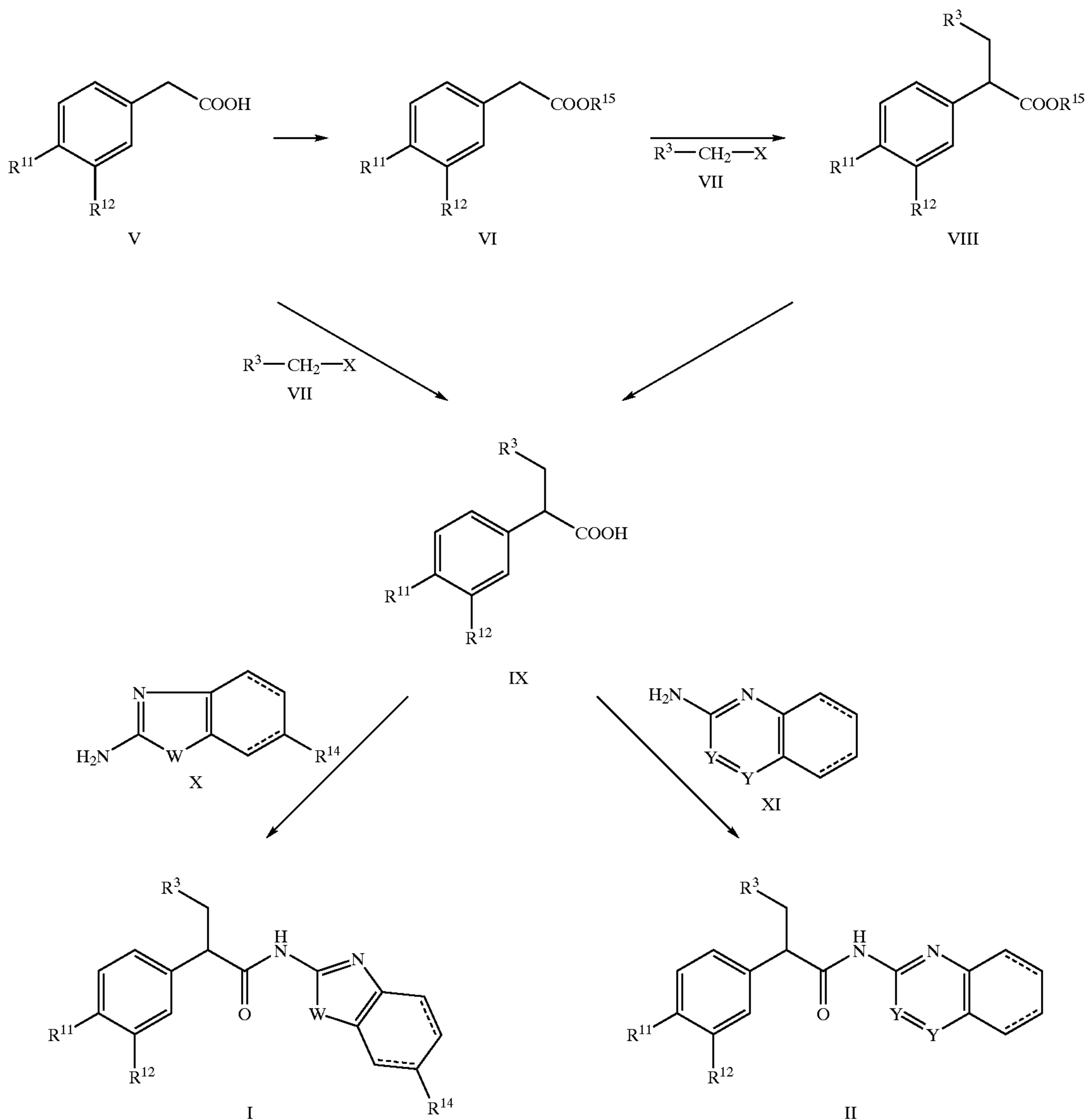
Reaction Scheme
