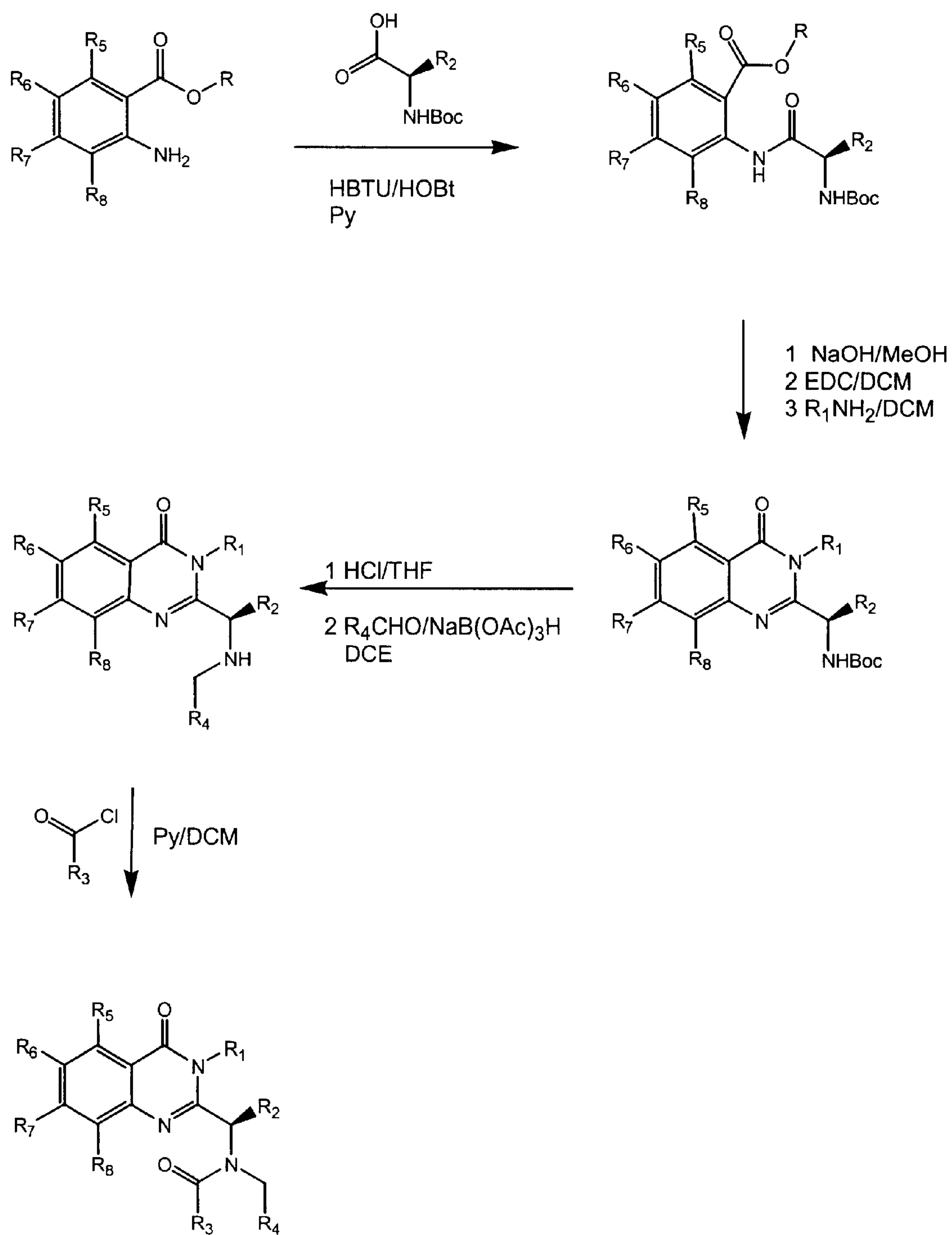
Figure 4: Asymmetric Synthesis
