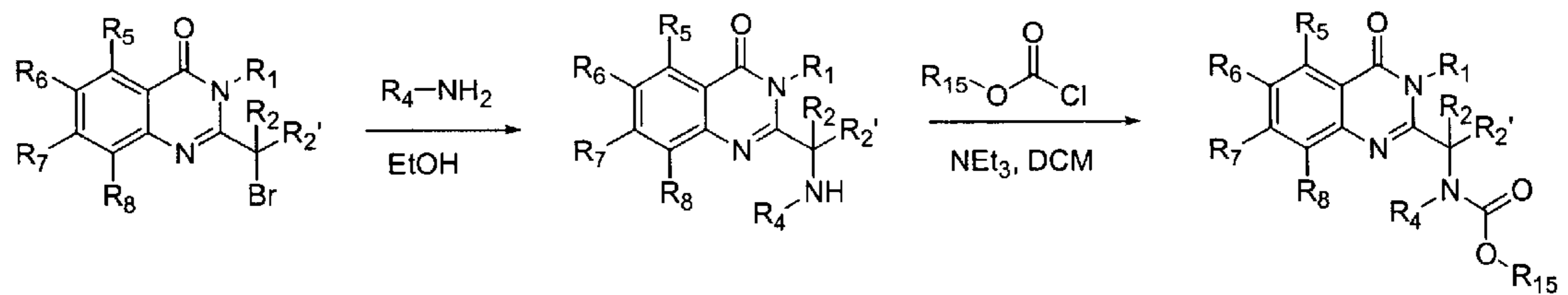
Figure 5c: Urea Synthesis
