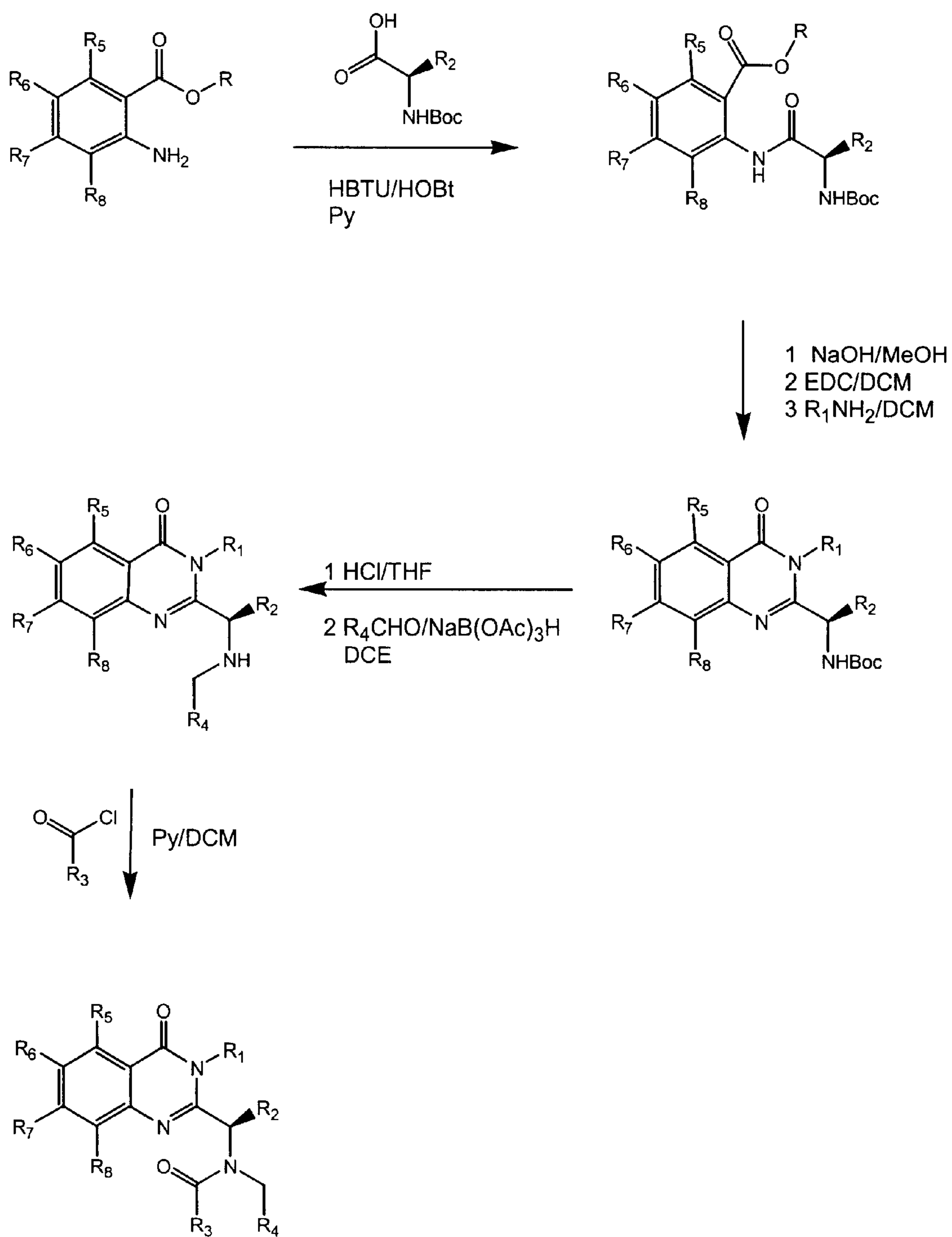
Figure 4: Asymmetric Synthesis
