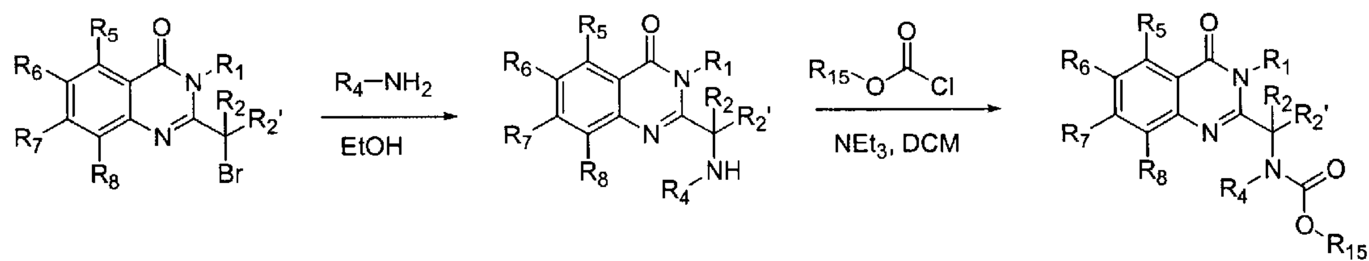
Figure 5c: Urea Synthesis
