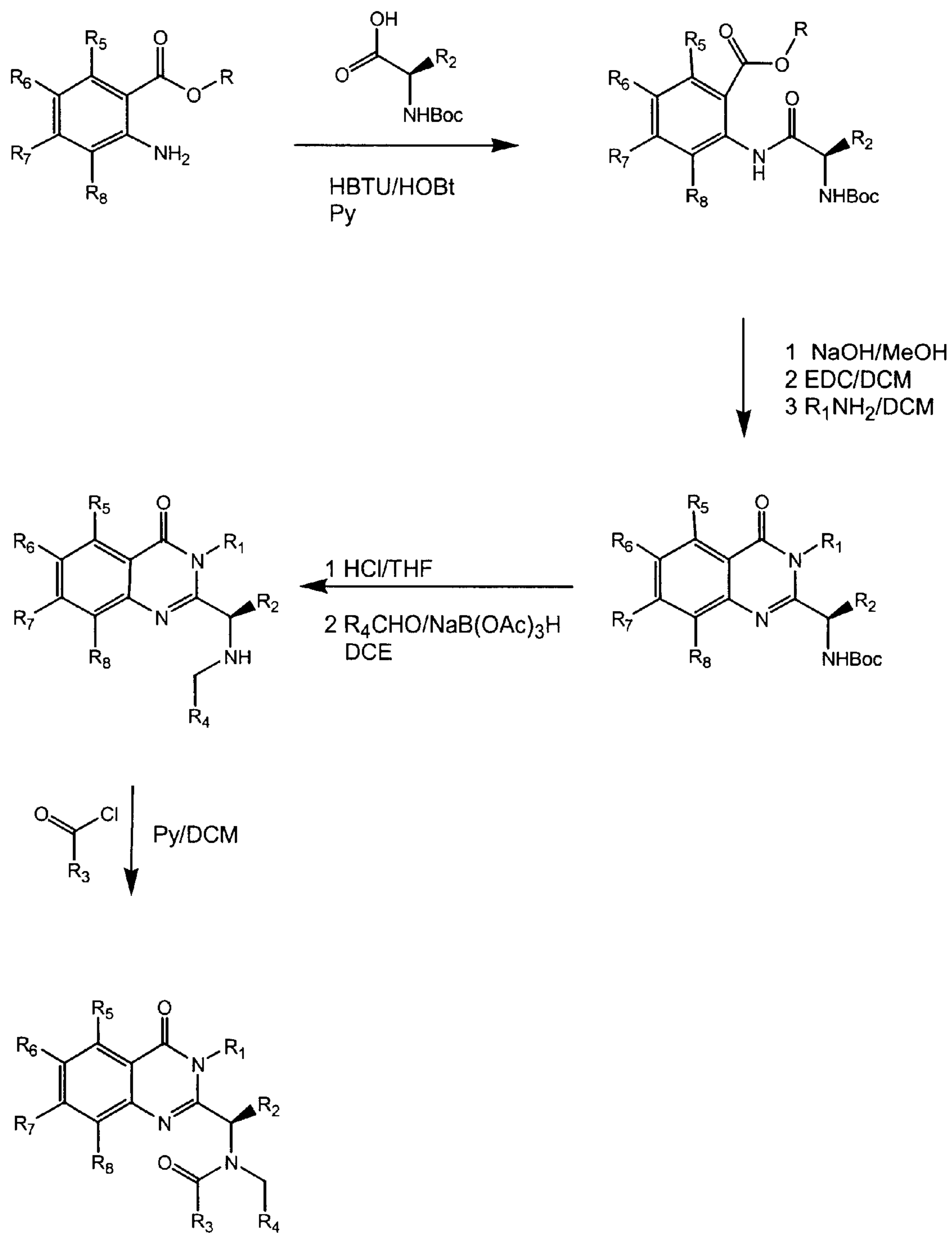
Figure 4: Asymmetric Synthesis
