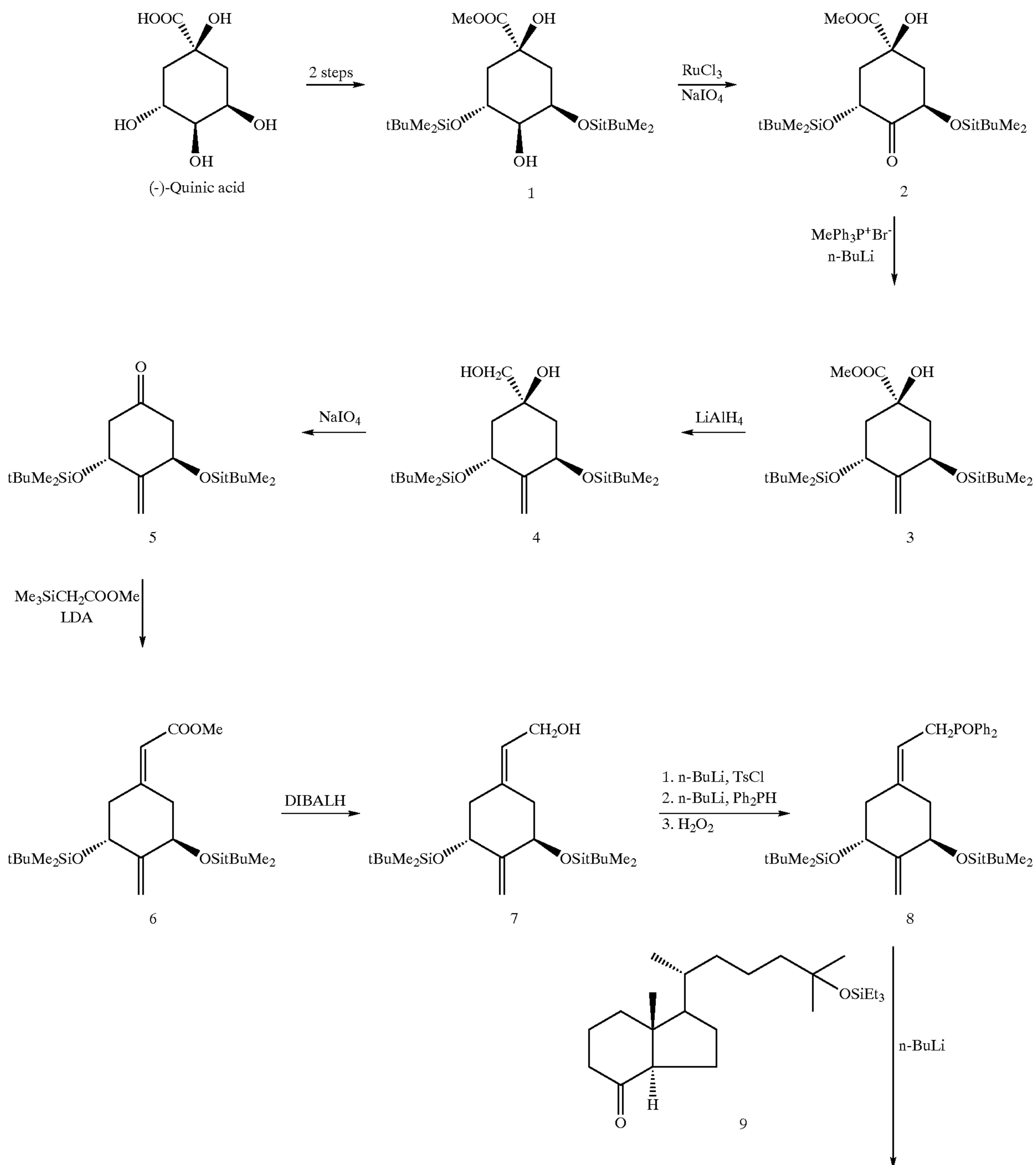
SCHEME I
