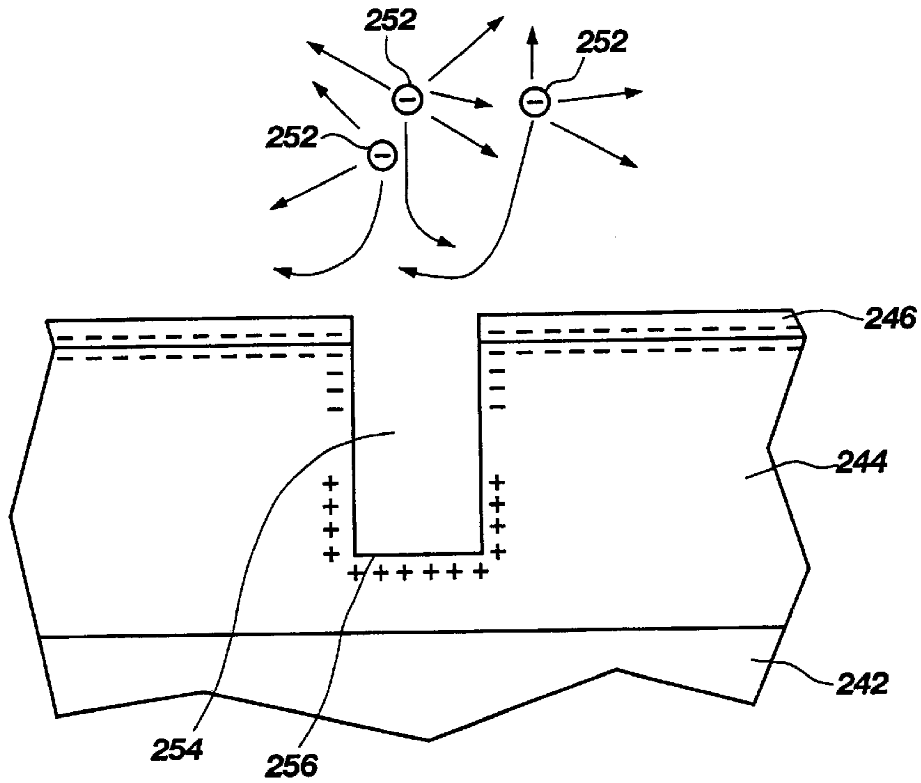
Fig. 8 (PRIOR ART)
