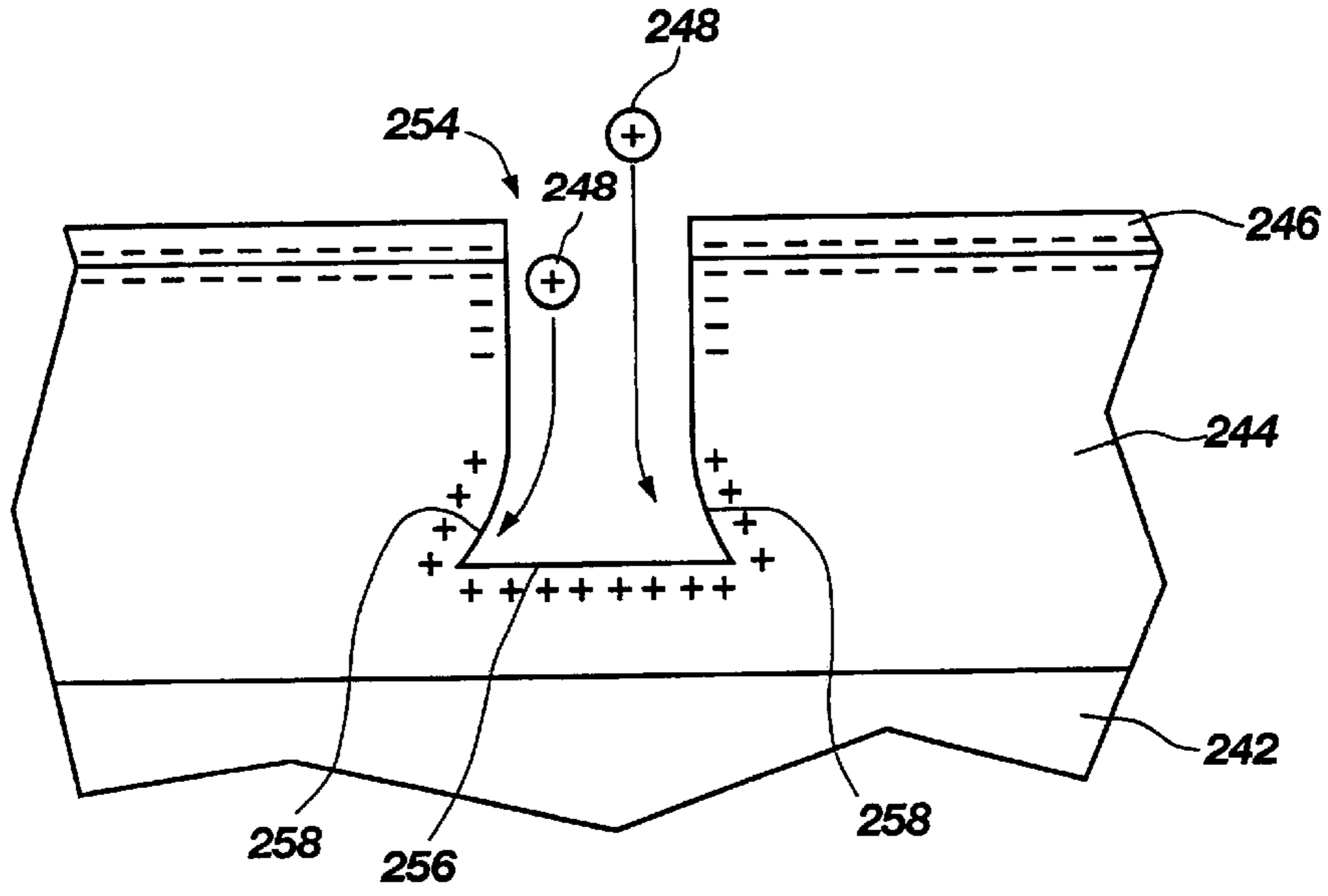
Fig. 7 (PRIOR ART)
