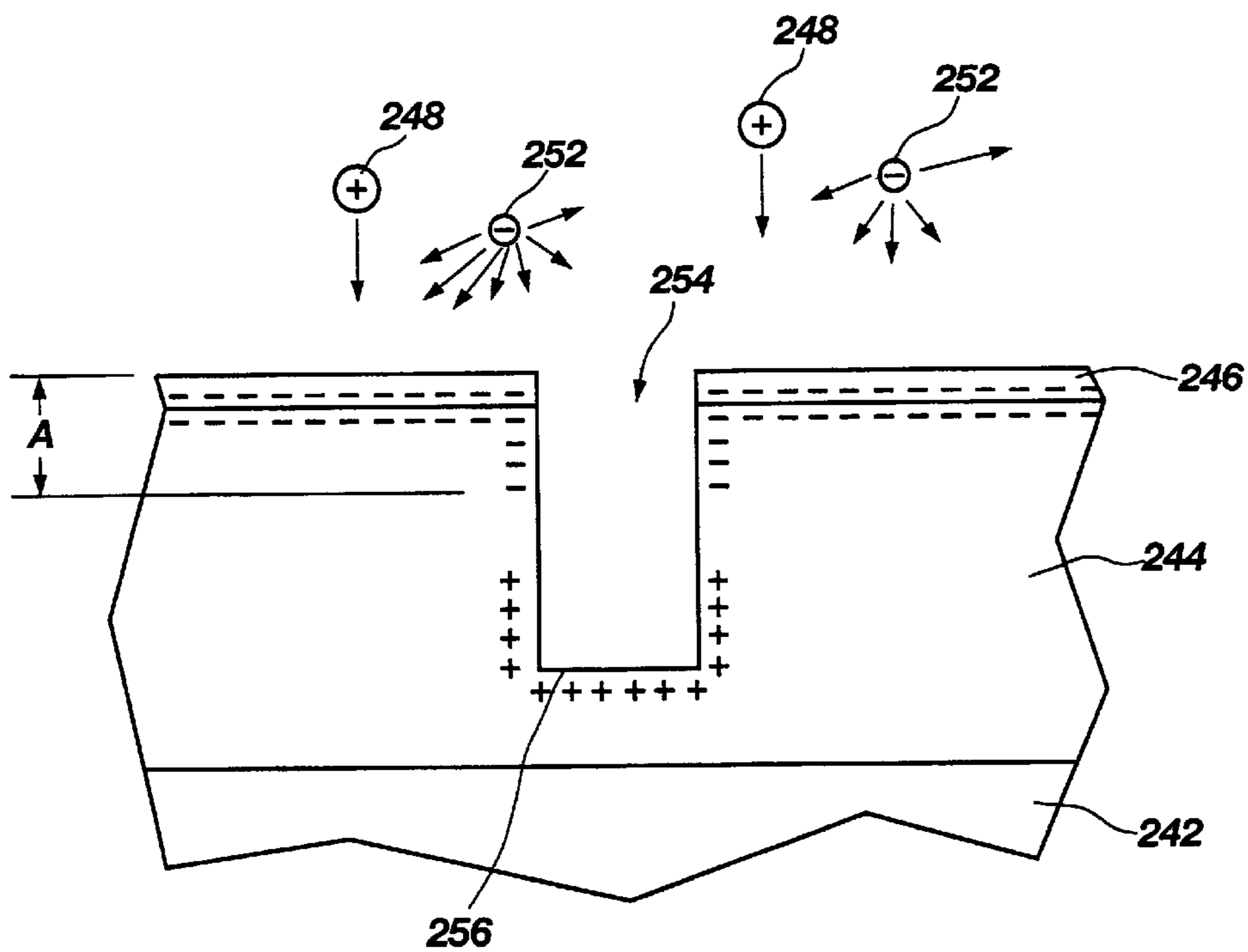
Fig. 6 (PRIOR ART)
