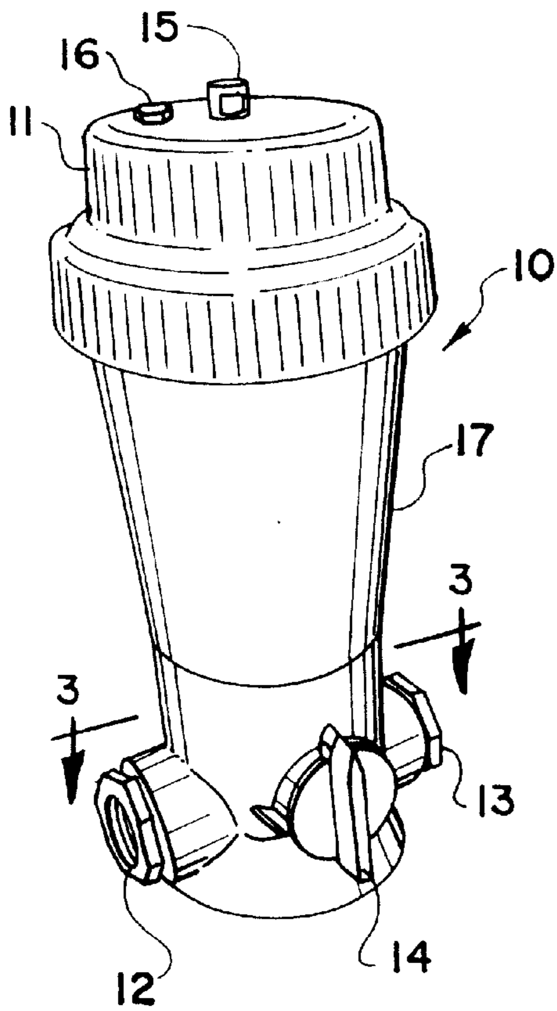
Fig. 2 PRIOR ART
