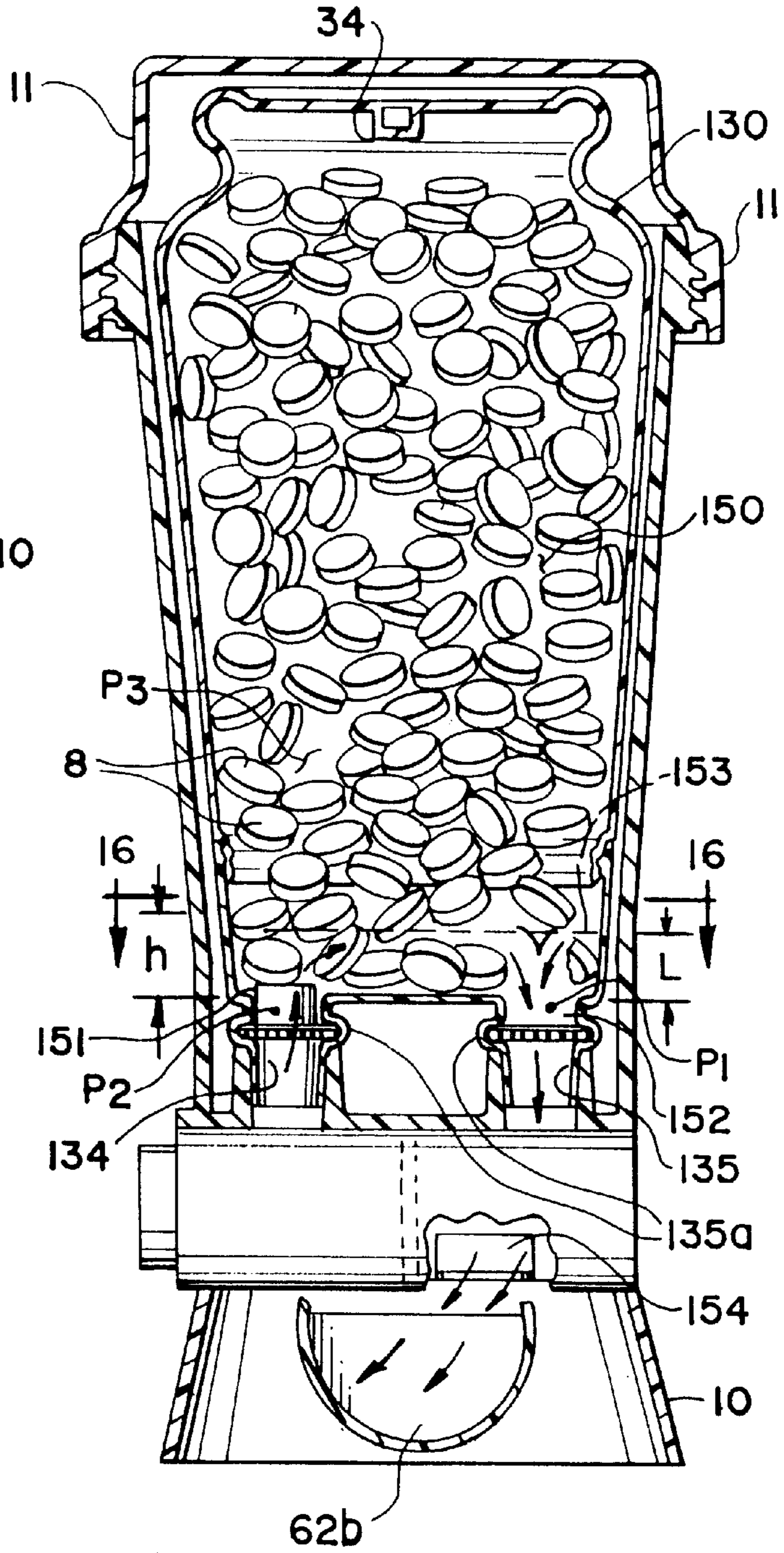
Fig. 1 PRIOR ART
