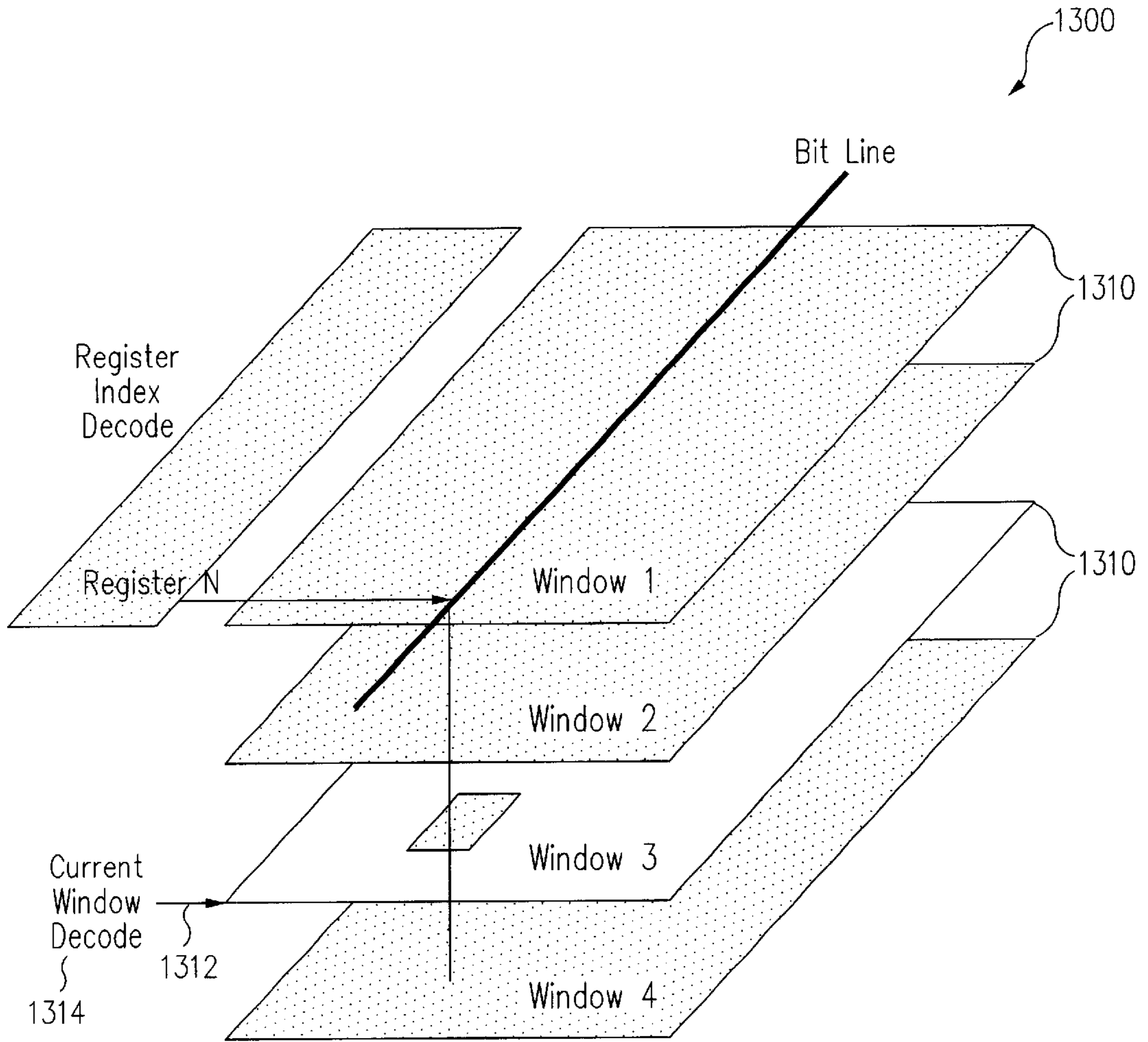
A Three Dimensional Register File
