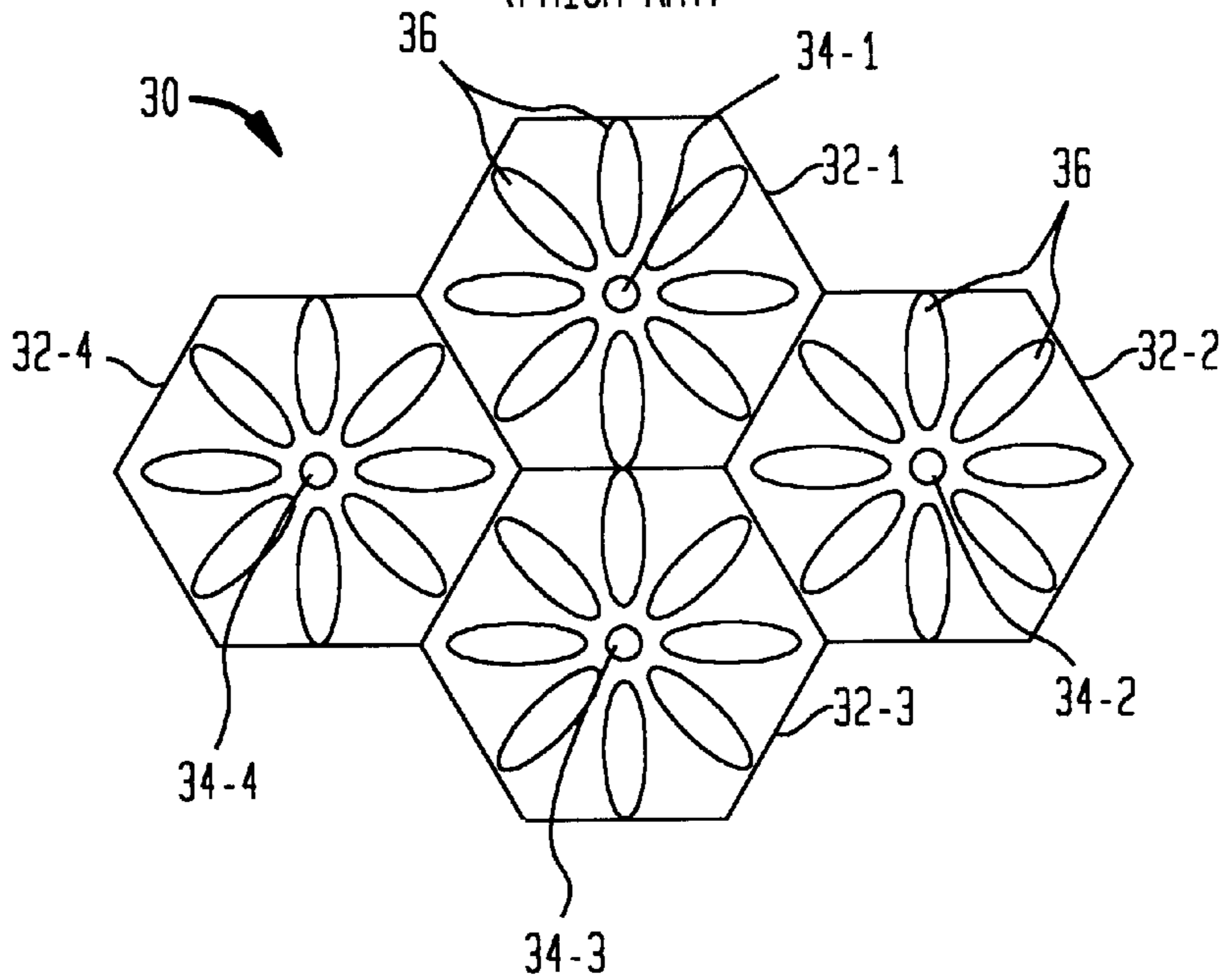
FIG. 3 (PRIOR ART)
