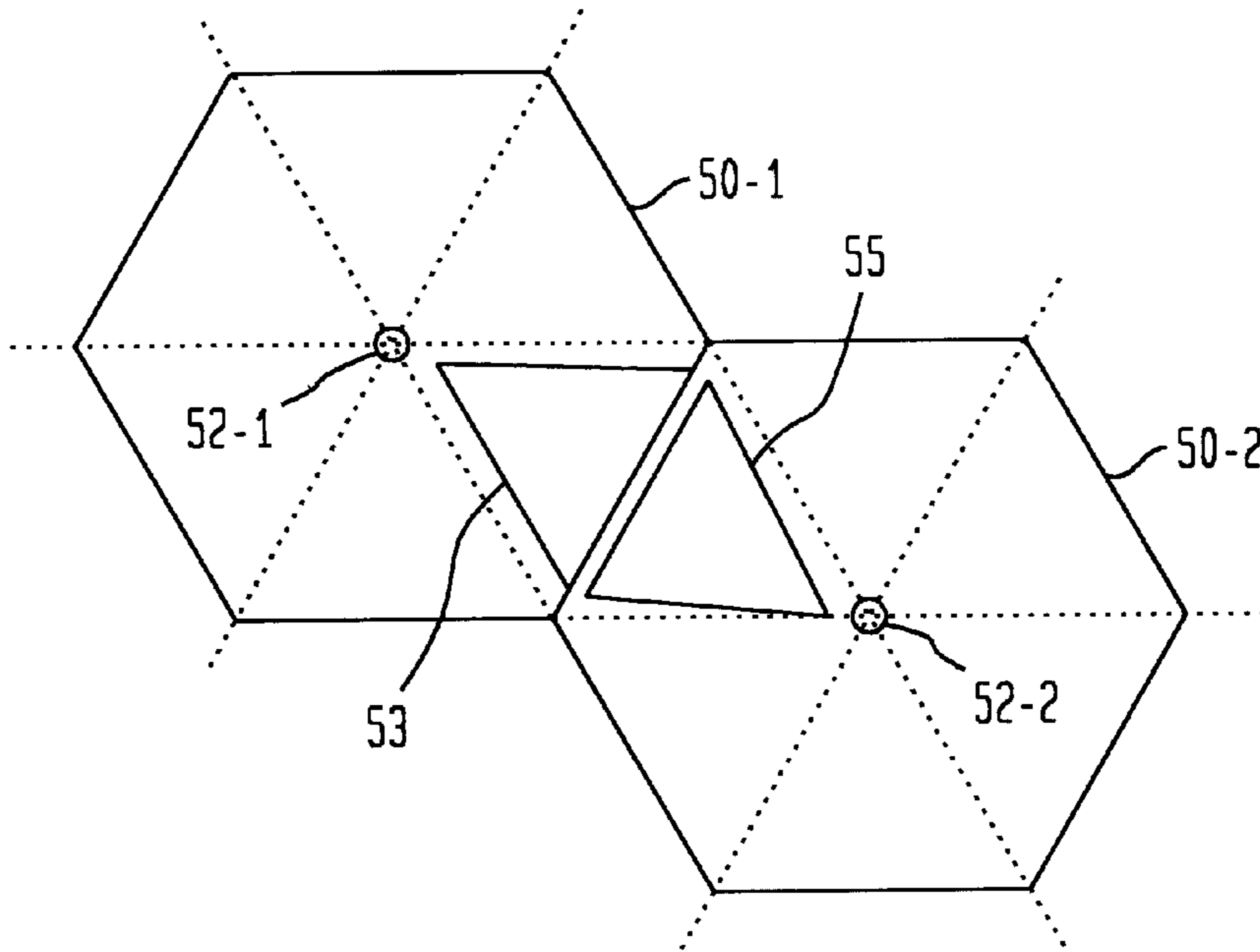
FIG. 5 (PRIOR ART)
