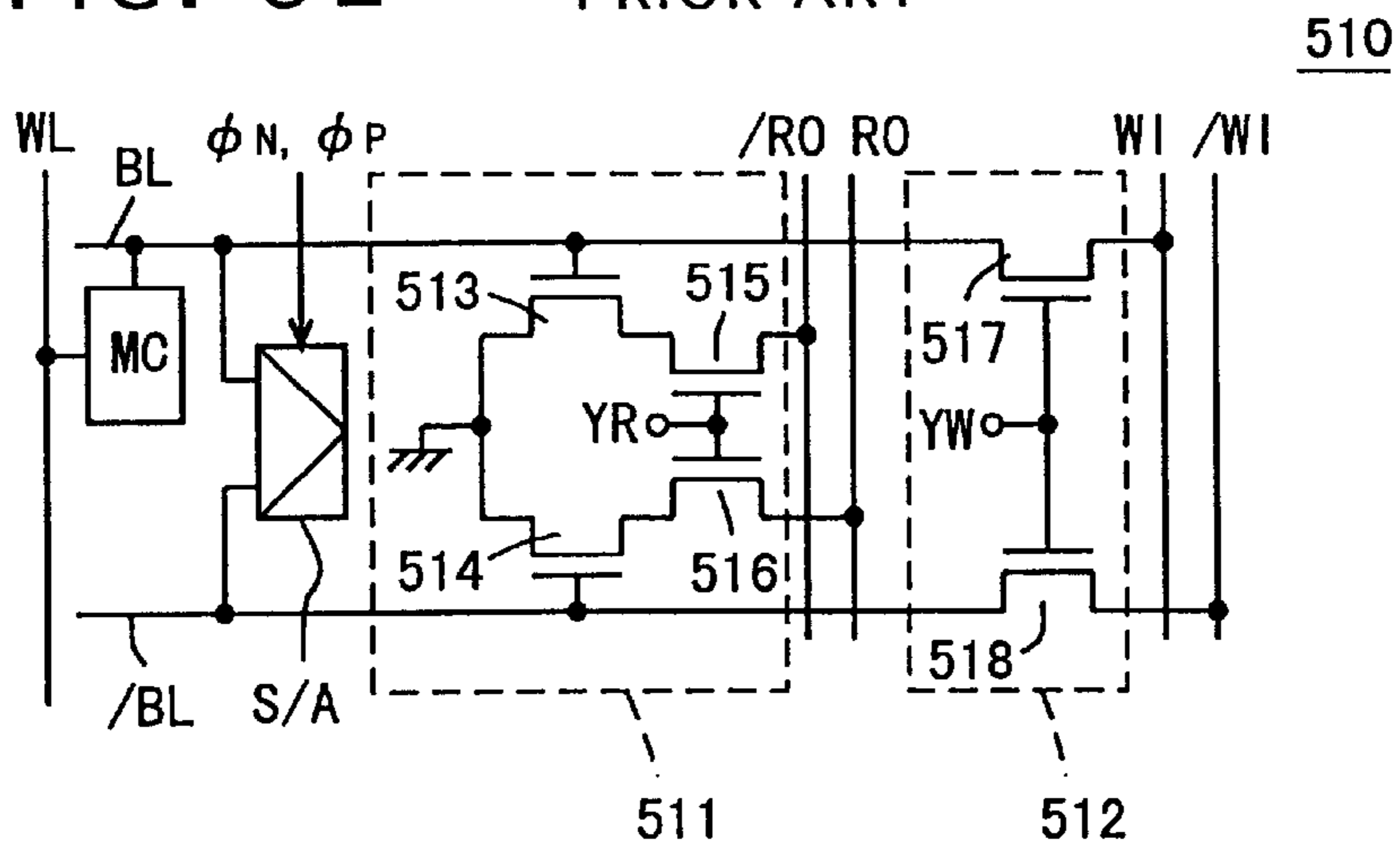
FIG. 32 PRIOR ART
