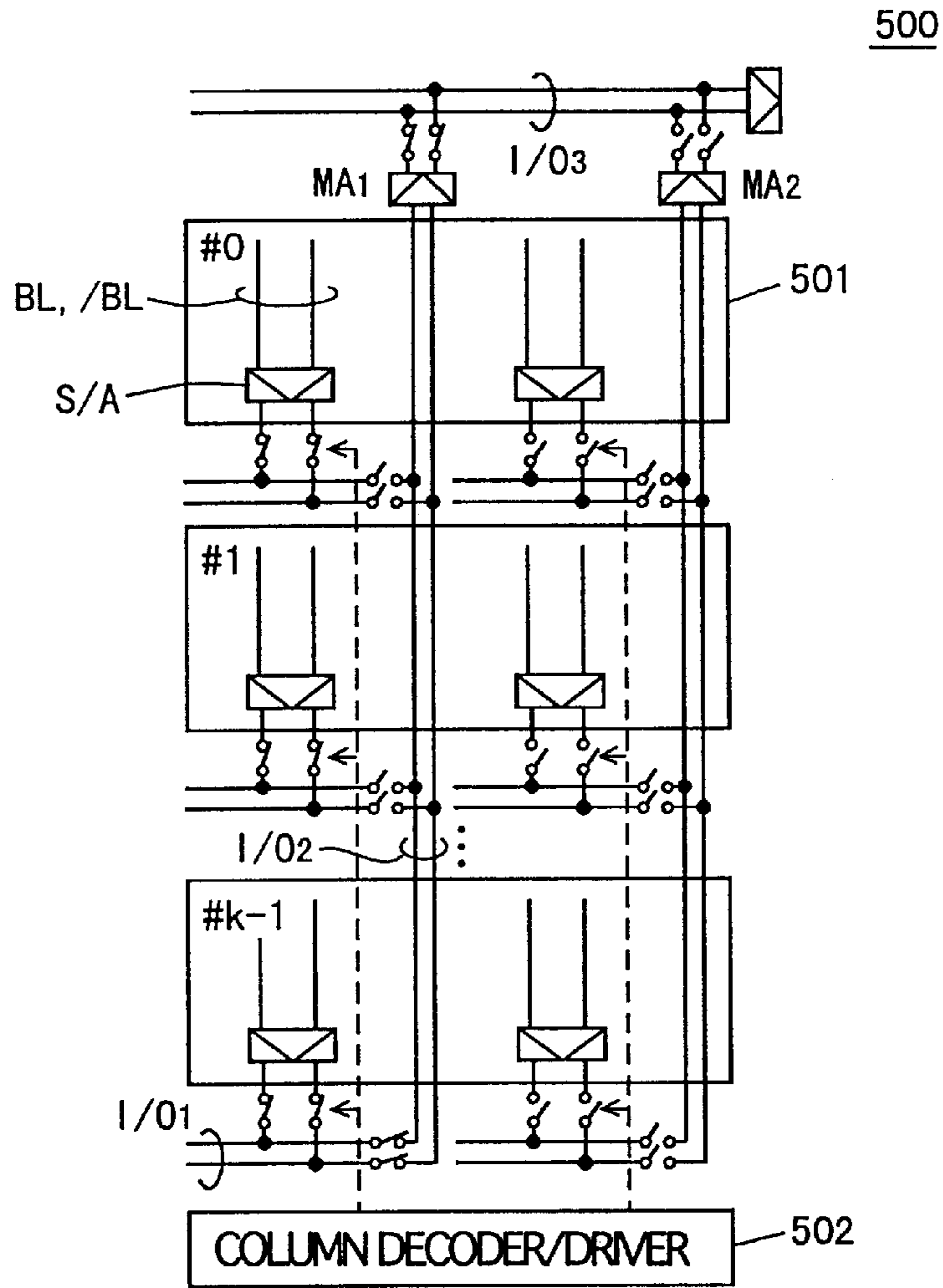
FIG. 31 PRIOR ART
