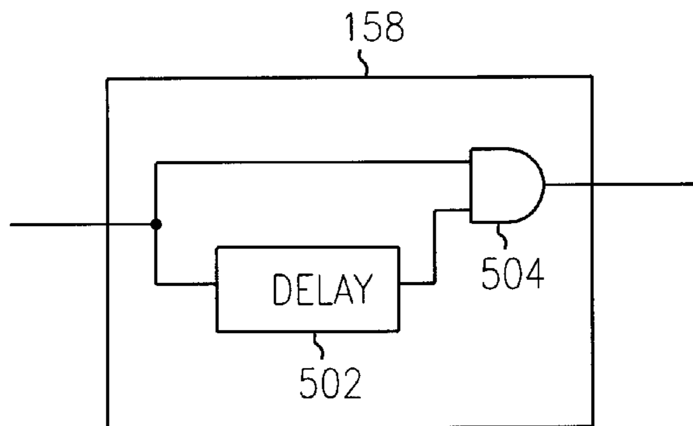
FIG. 6 (PRIOR ART)
