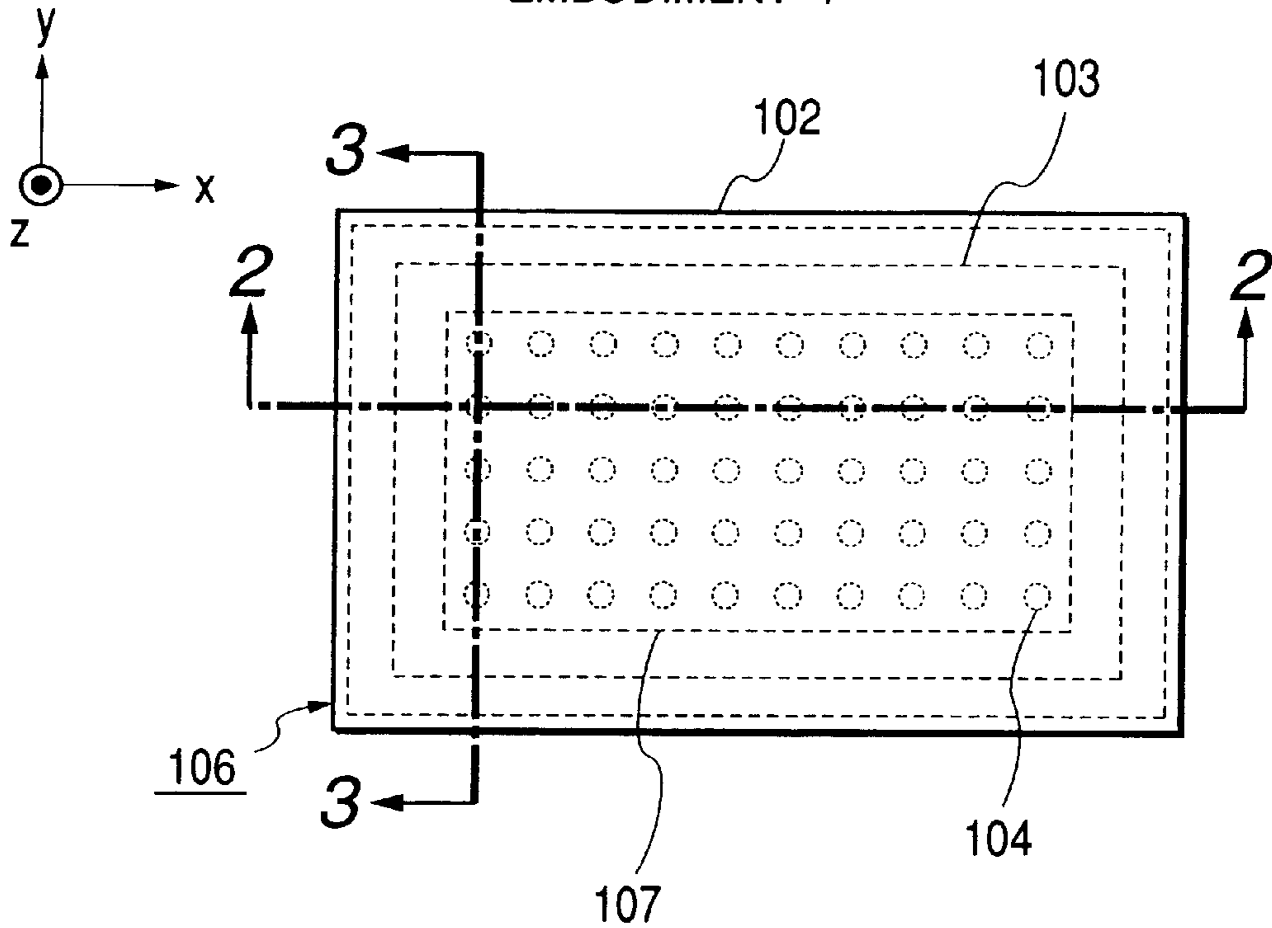
FRONT VIEW OF VACUUM CHAMBER EMBODIMENT 1
