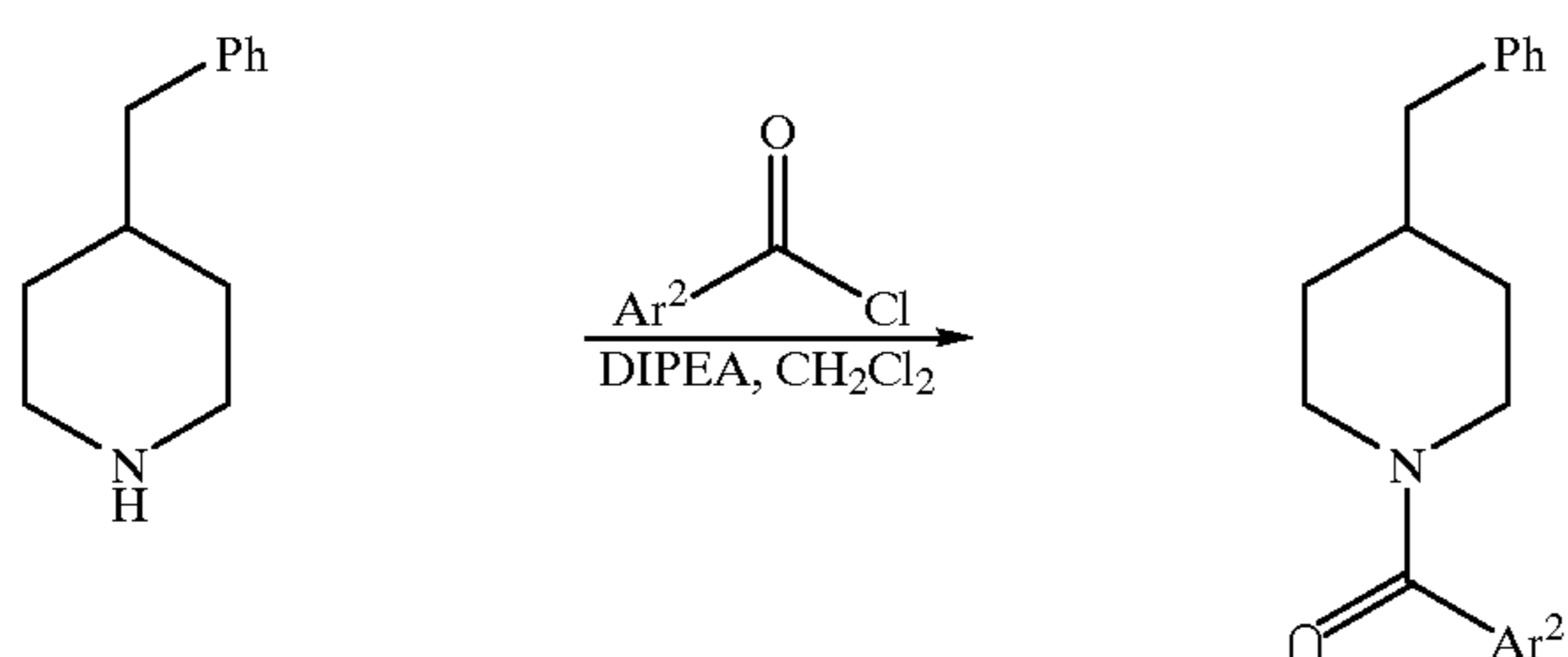
Reaction Scheme 1
