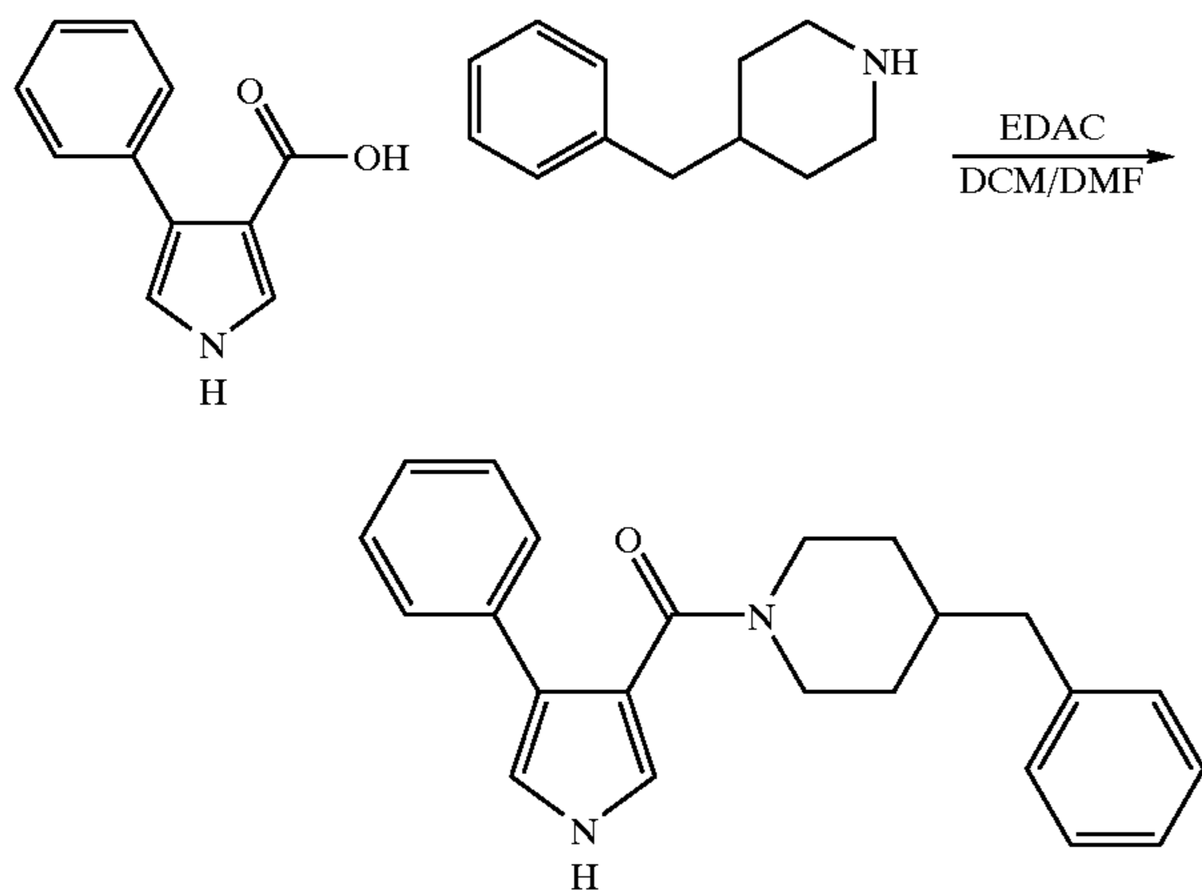
Reaction Scheme 5
