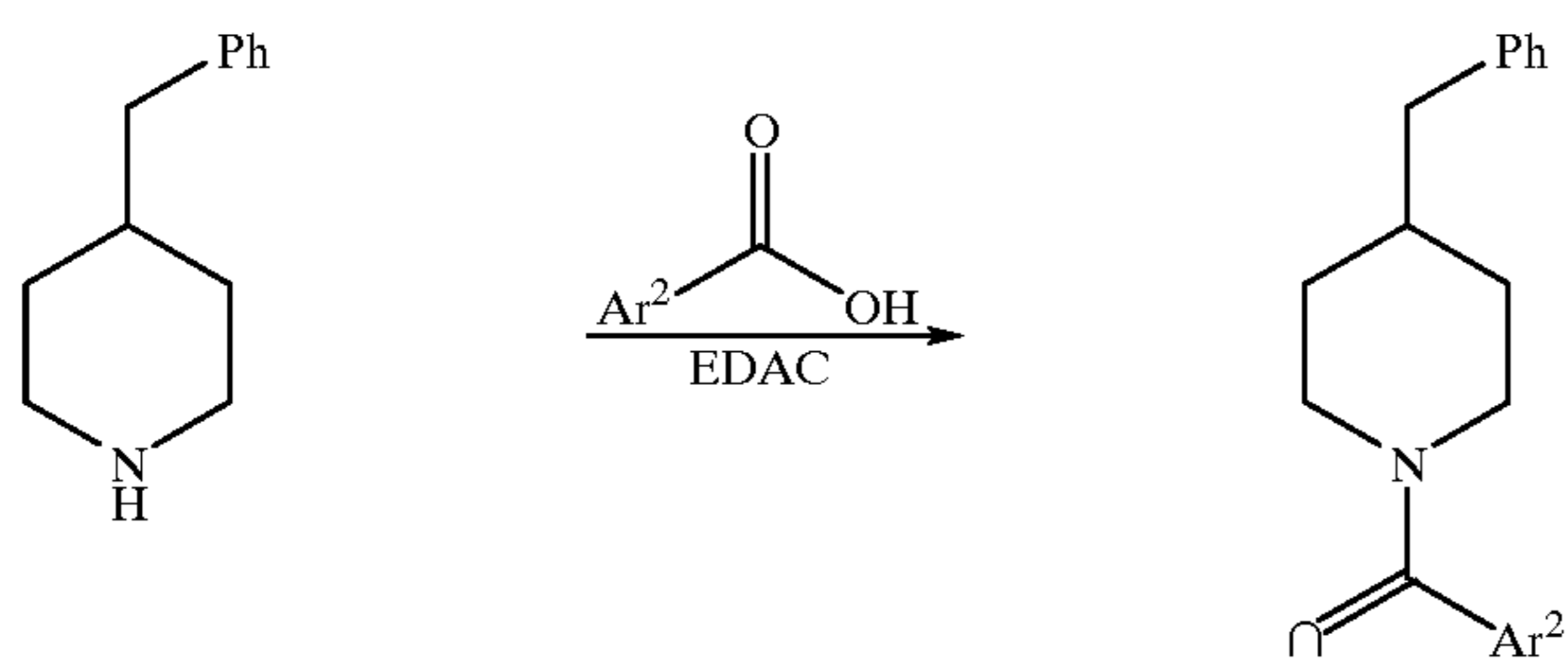
Reaction Scheme 2
