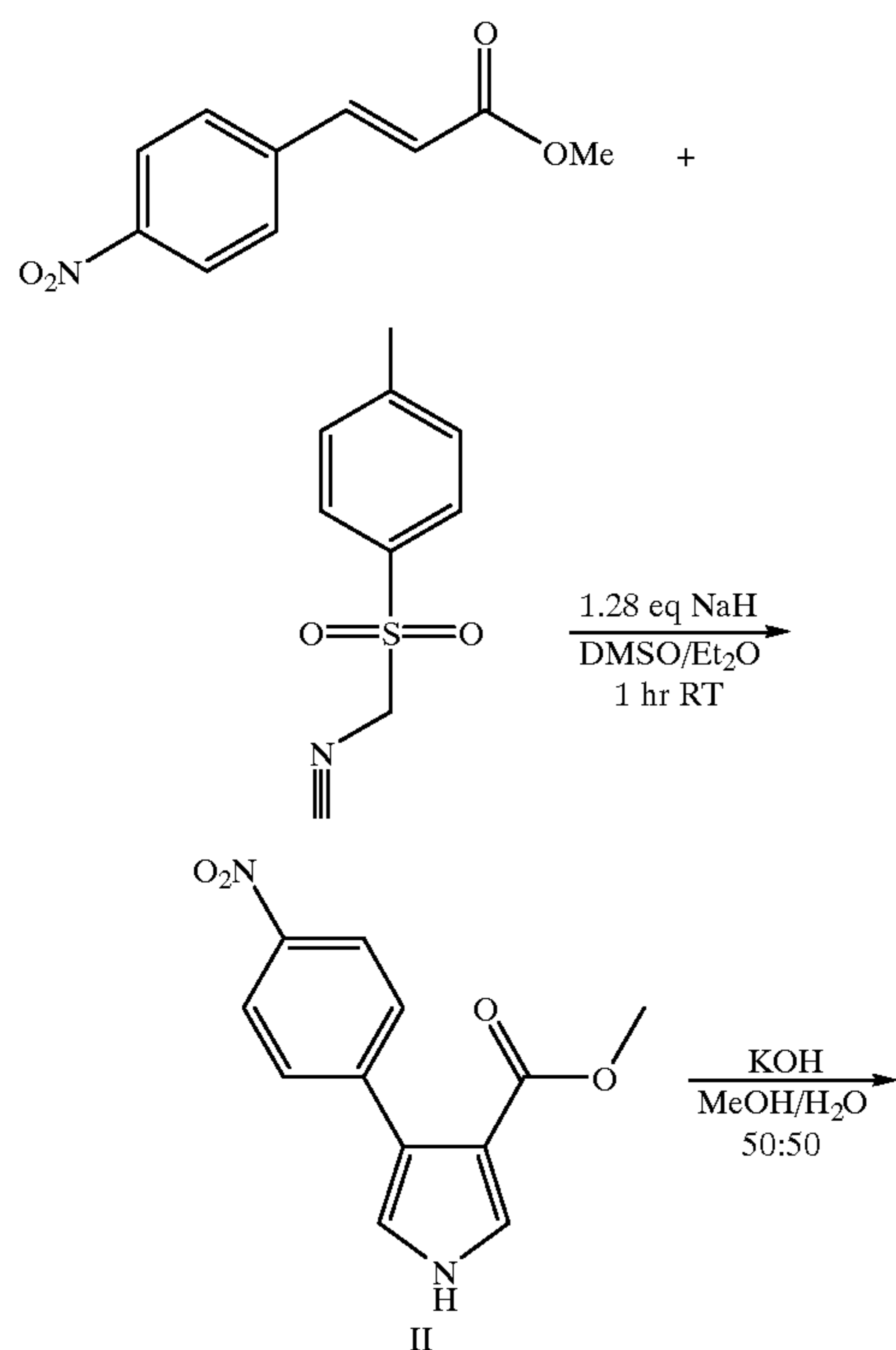
Reaction Scheme 6
