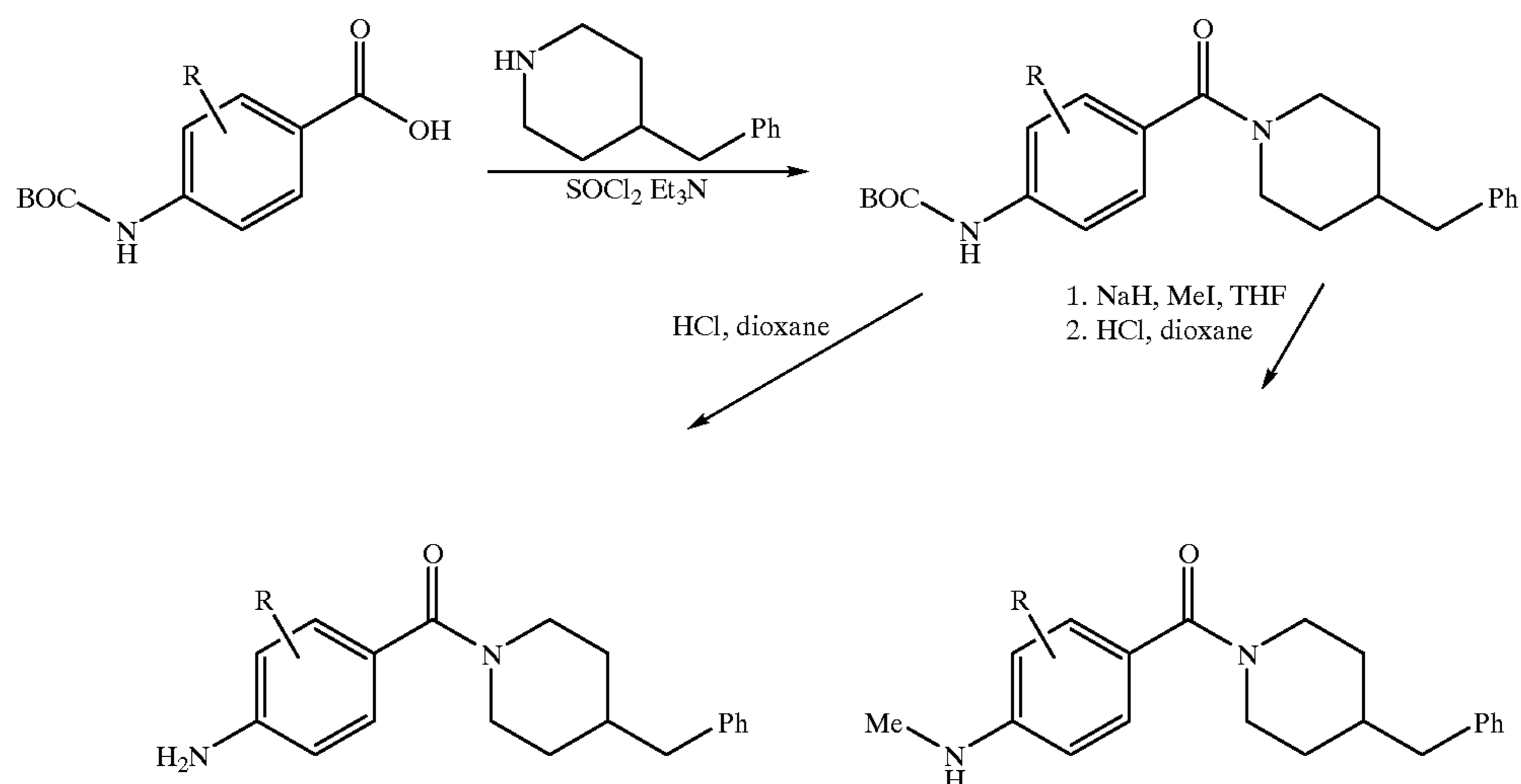
Reaction Scheme 3
