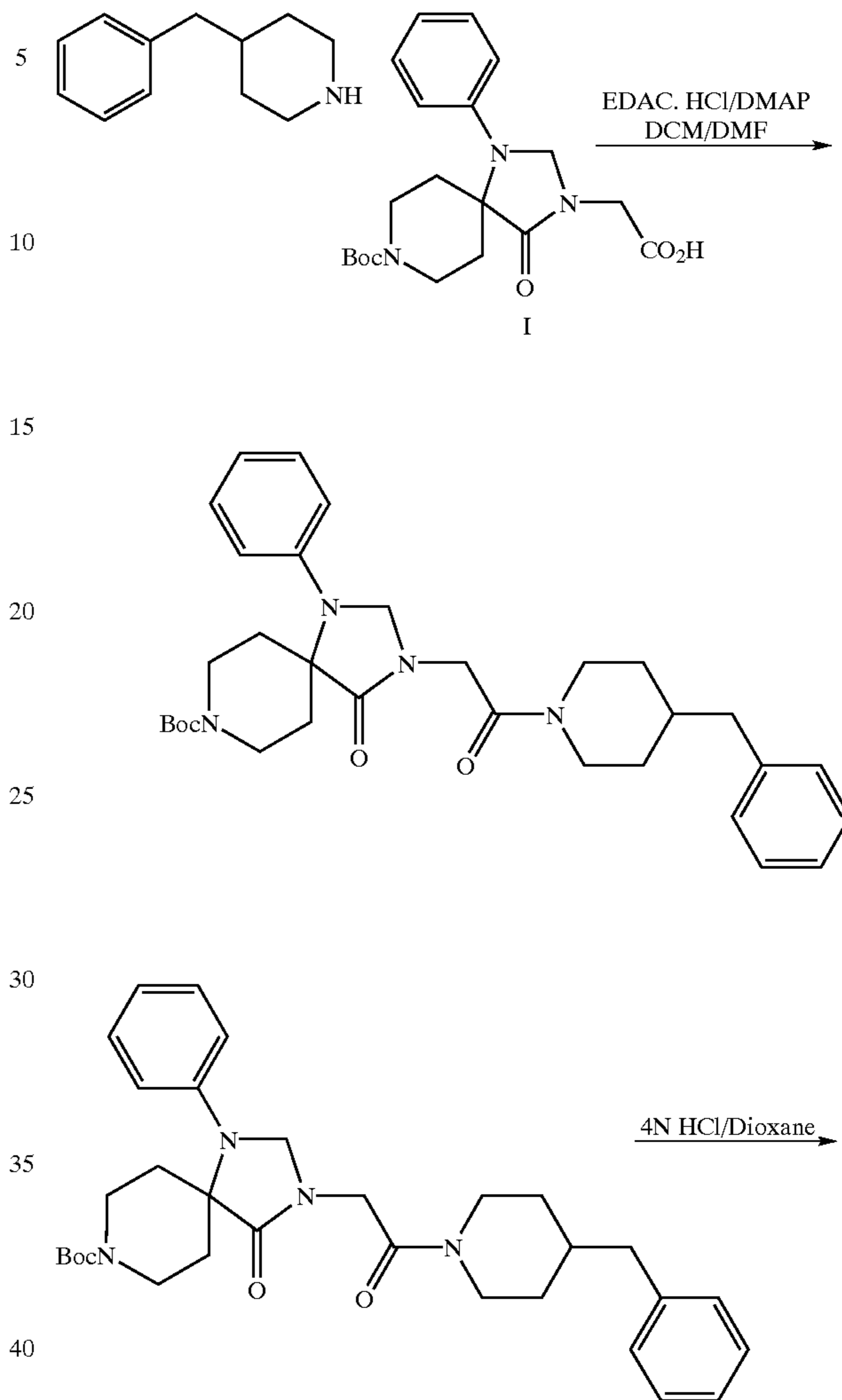
Reaction Scheme 4
