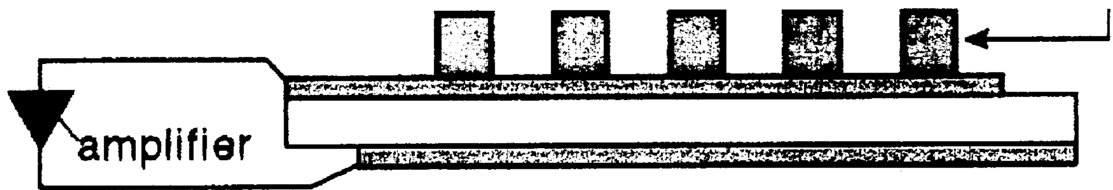
Figure 13. Model of a carbon electrode with immobilized cholinesterase enzyme.
