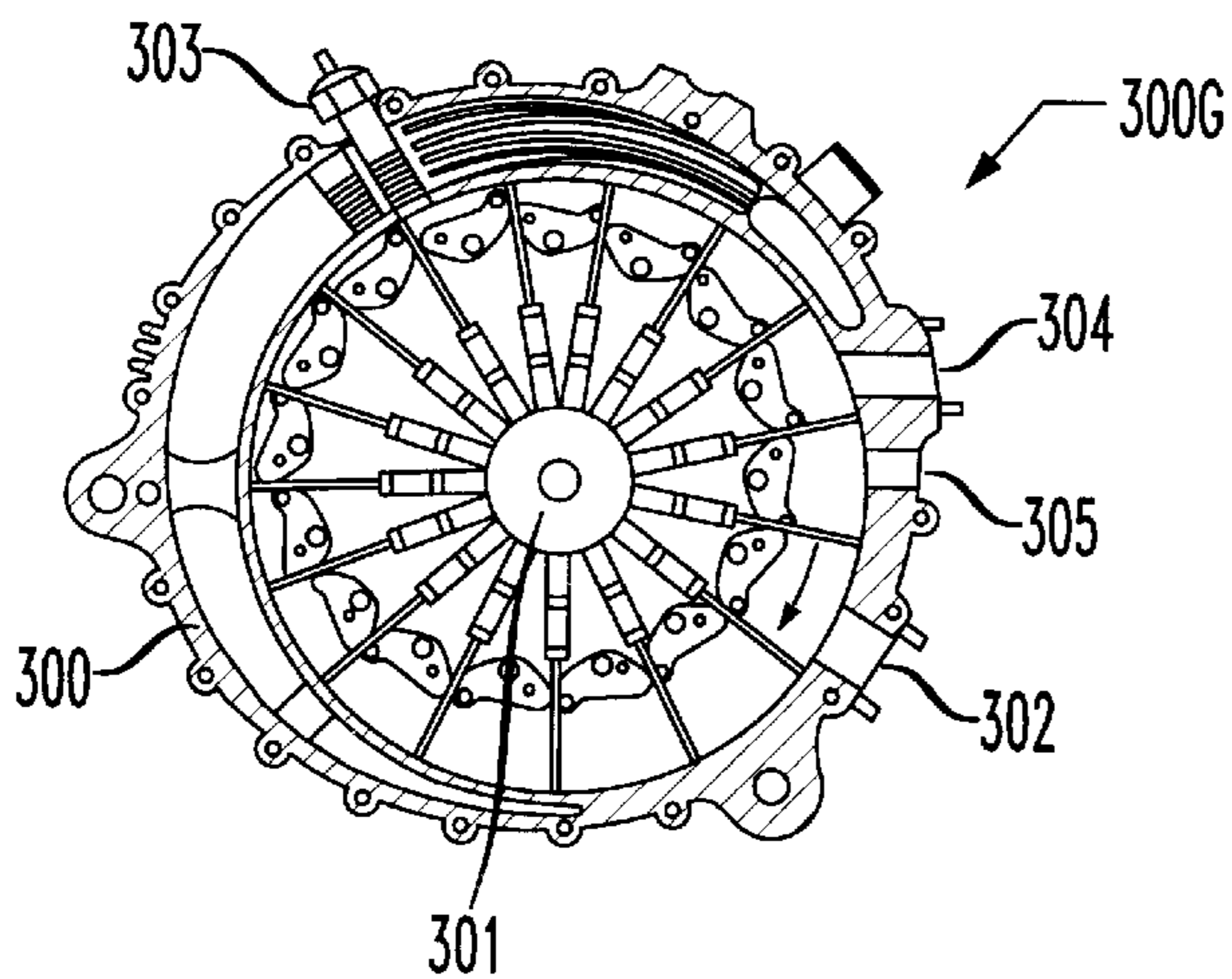
FIG. 18 (PRIOR ART)
