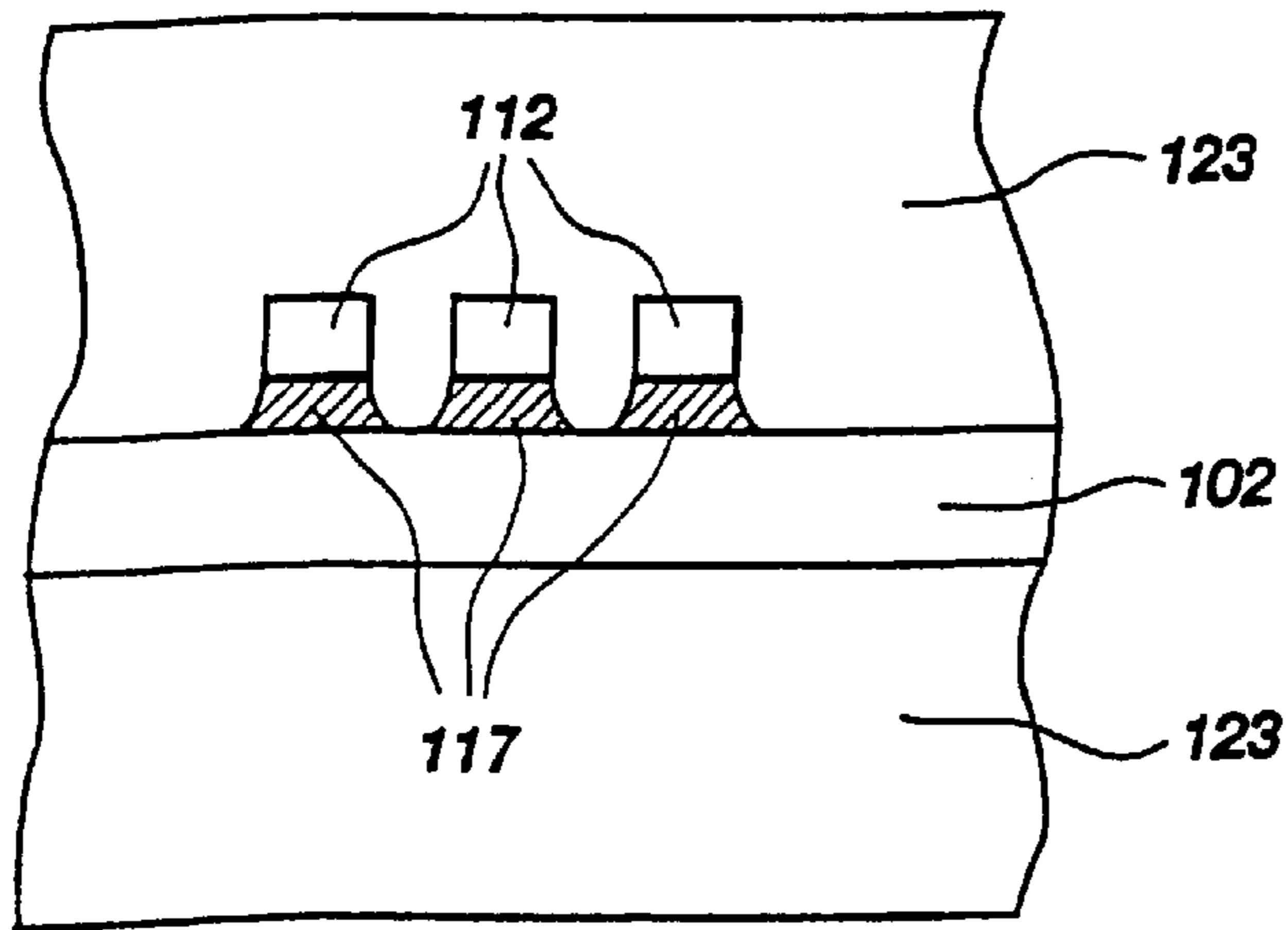
SECTION 10-10
