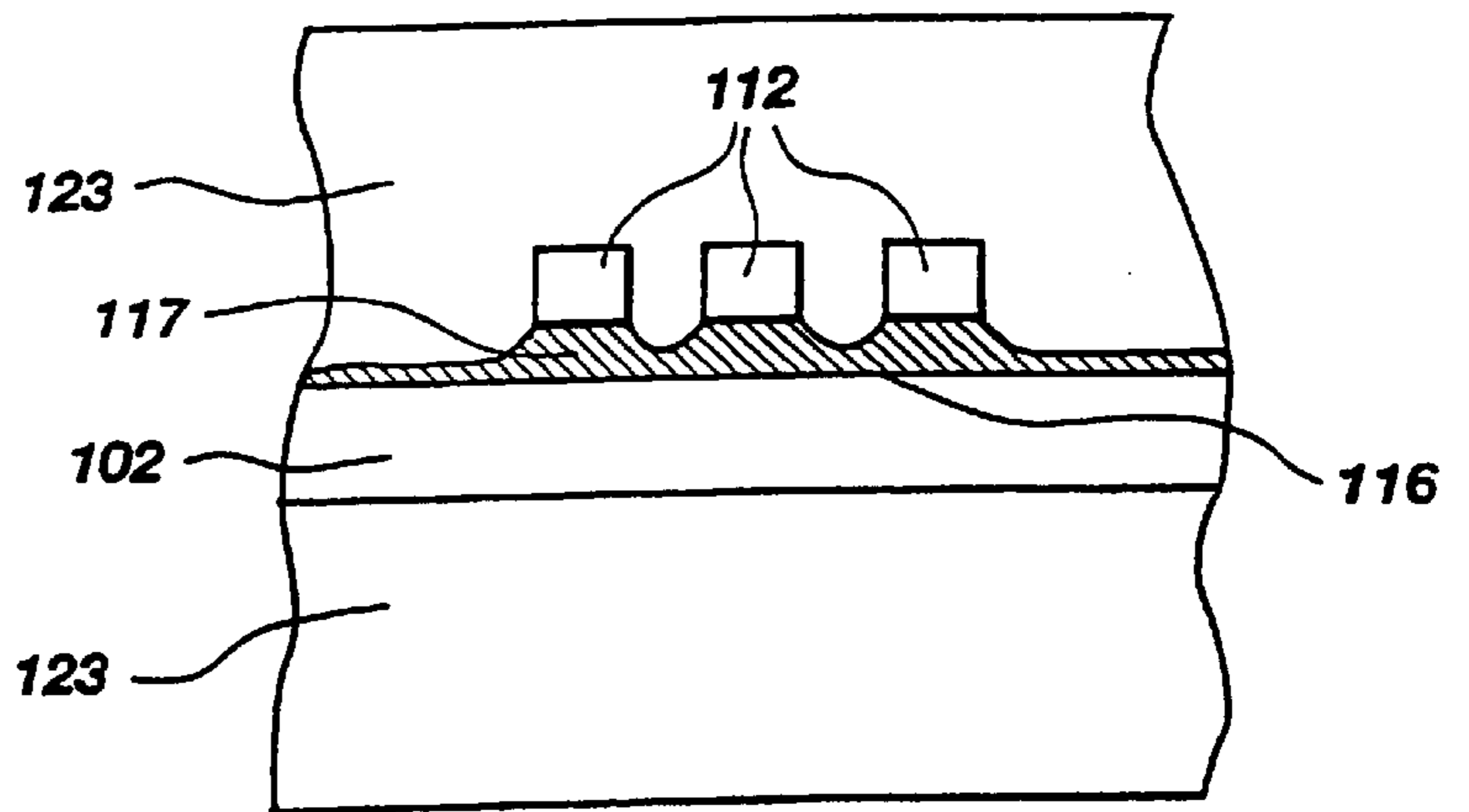
SECTION 10-10
