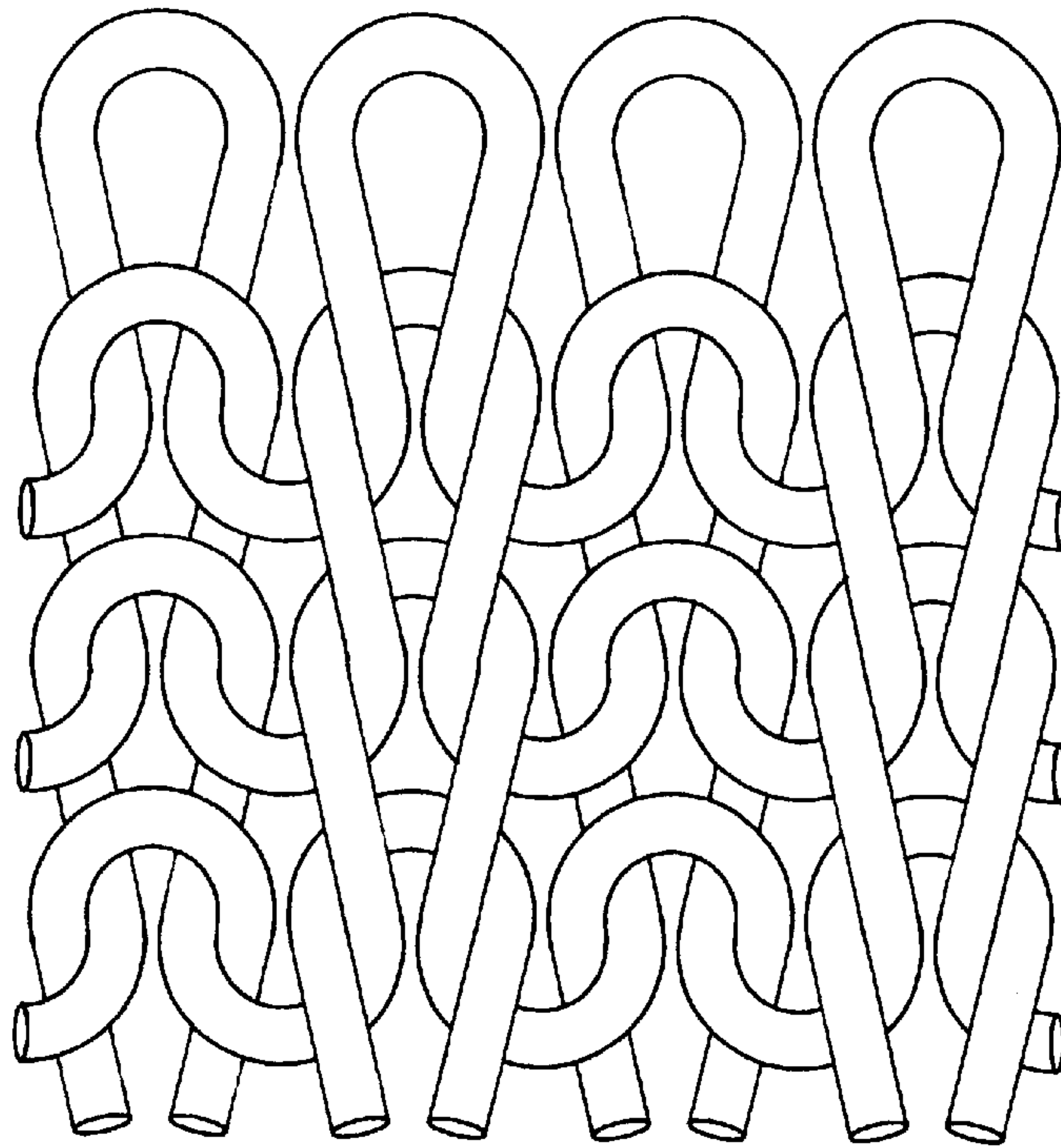
Rib Structure
