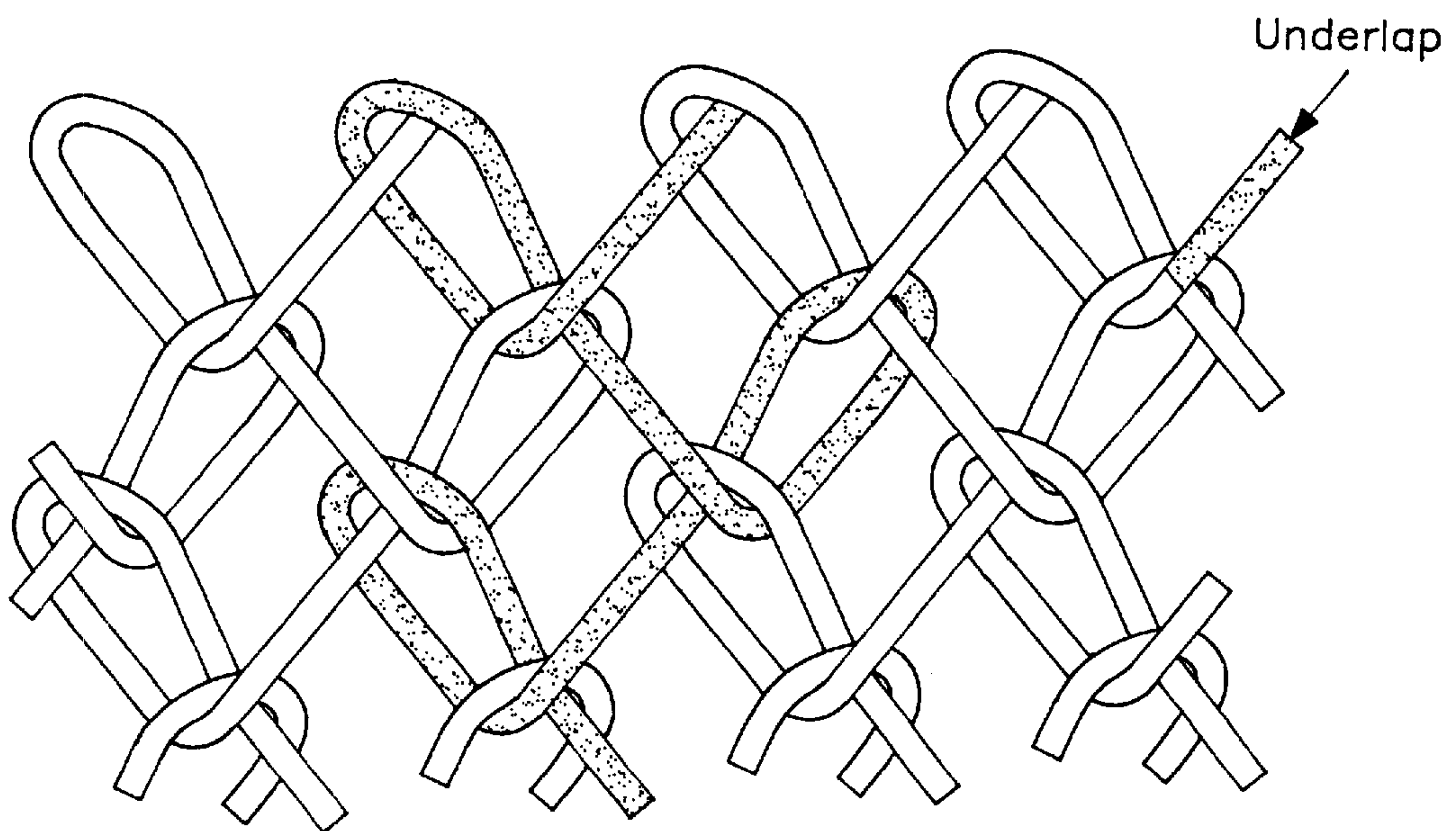
Tricot warp knitted Structure
