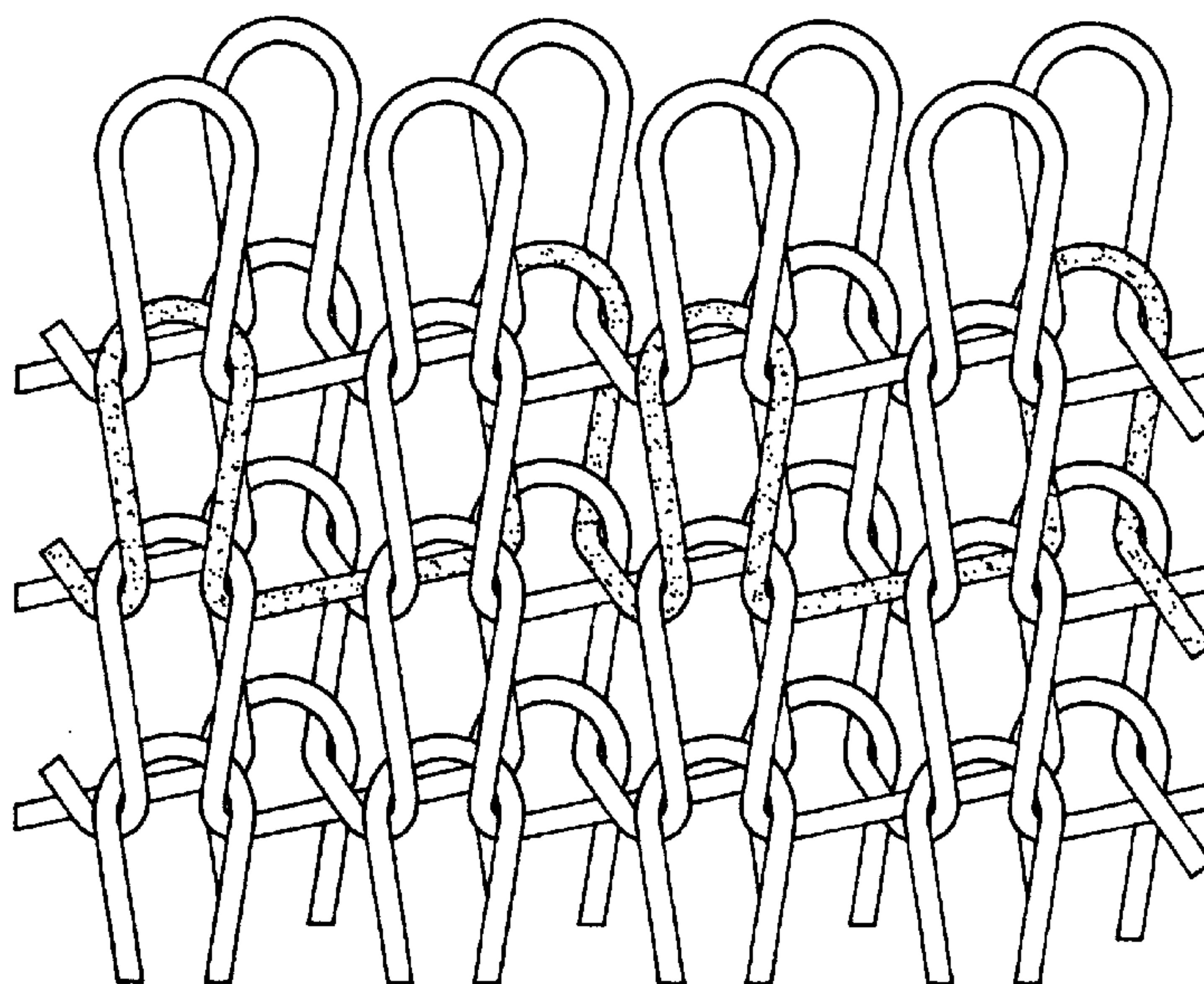
Interlocking Structure
