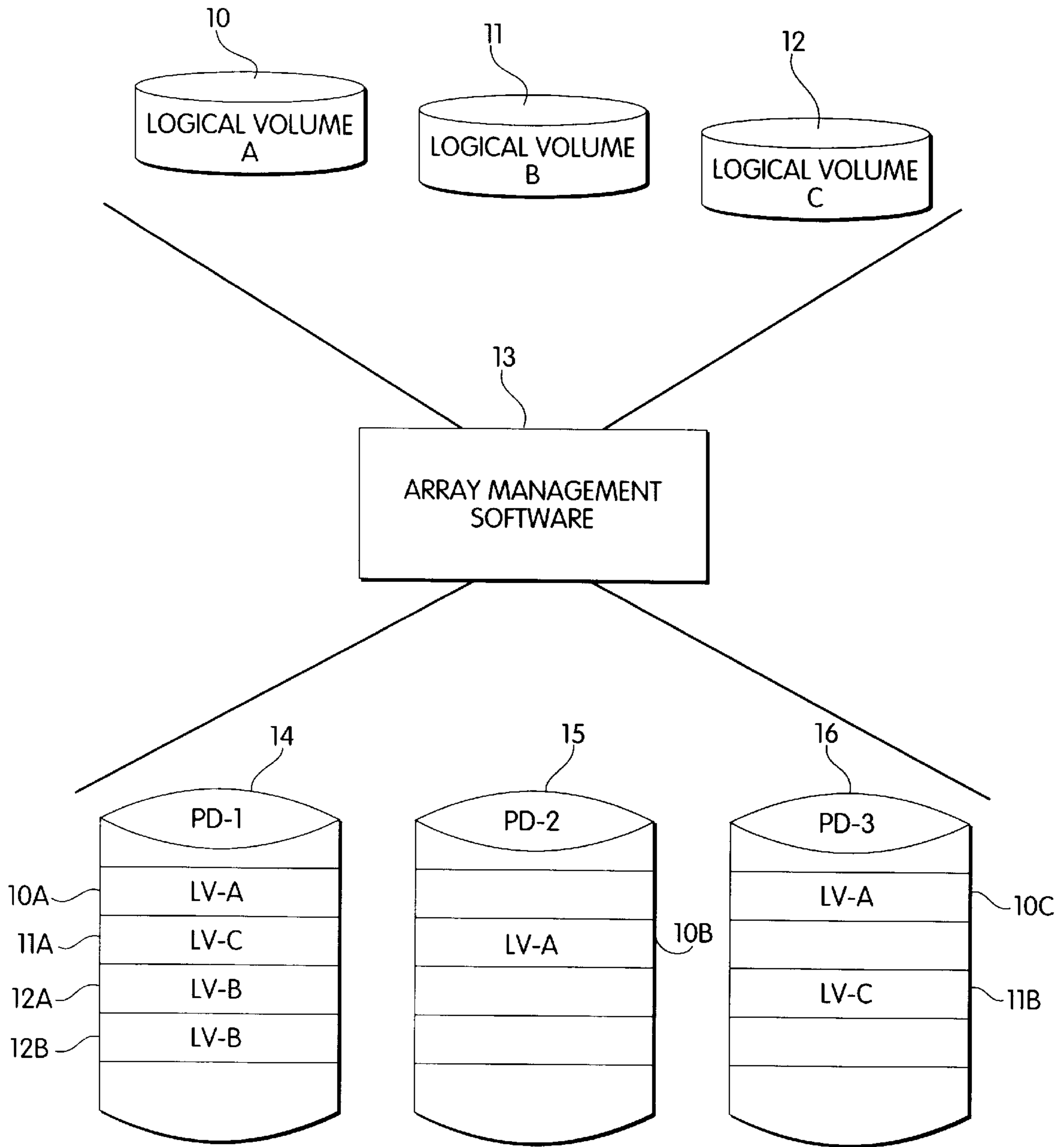
Fig. 1 (PRIOR ART)
