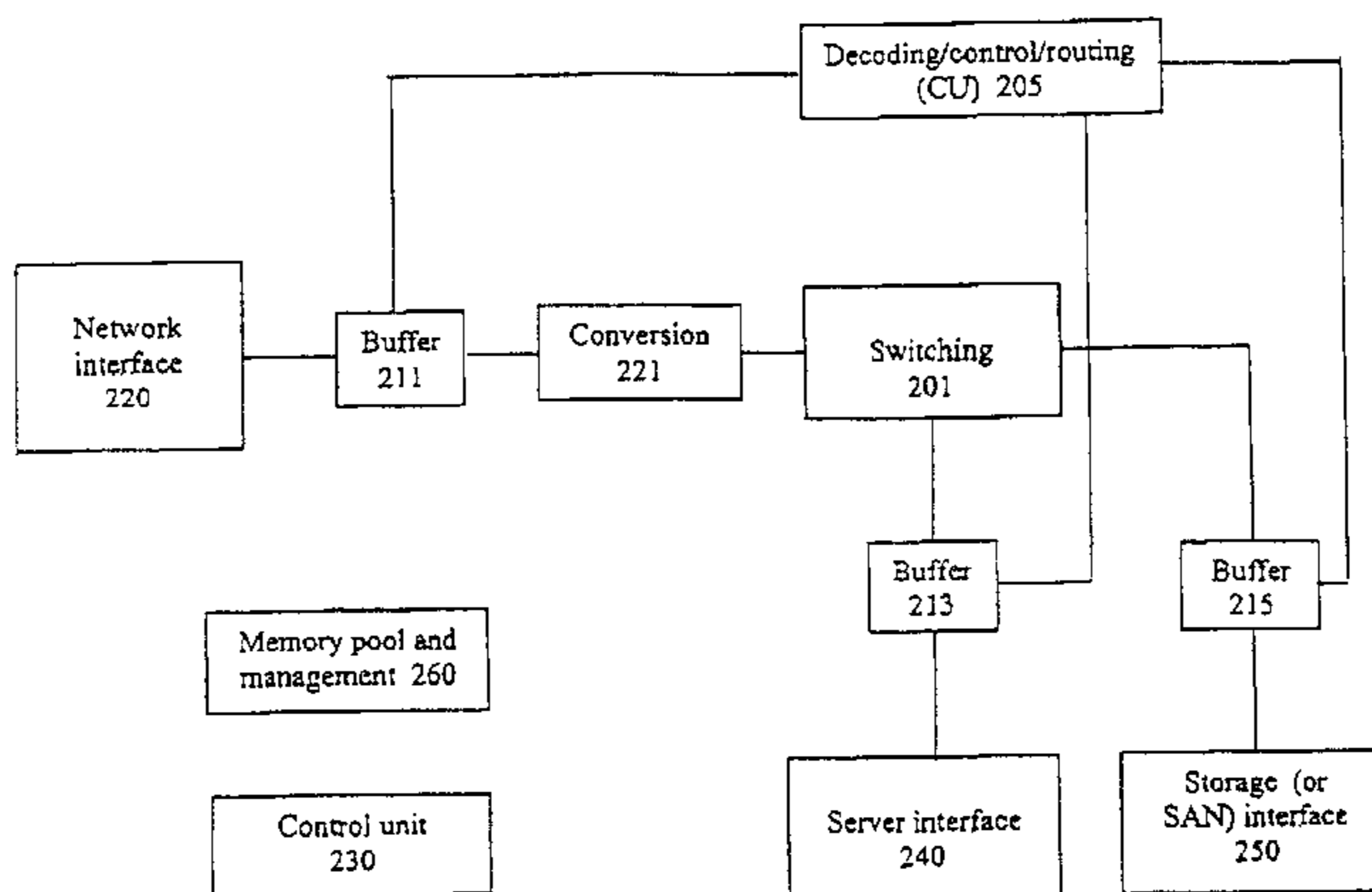
Block Function Diagram
