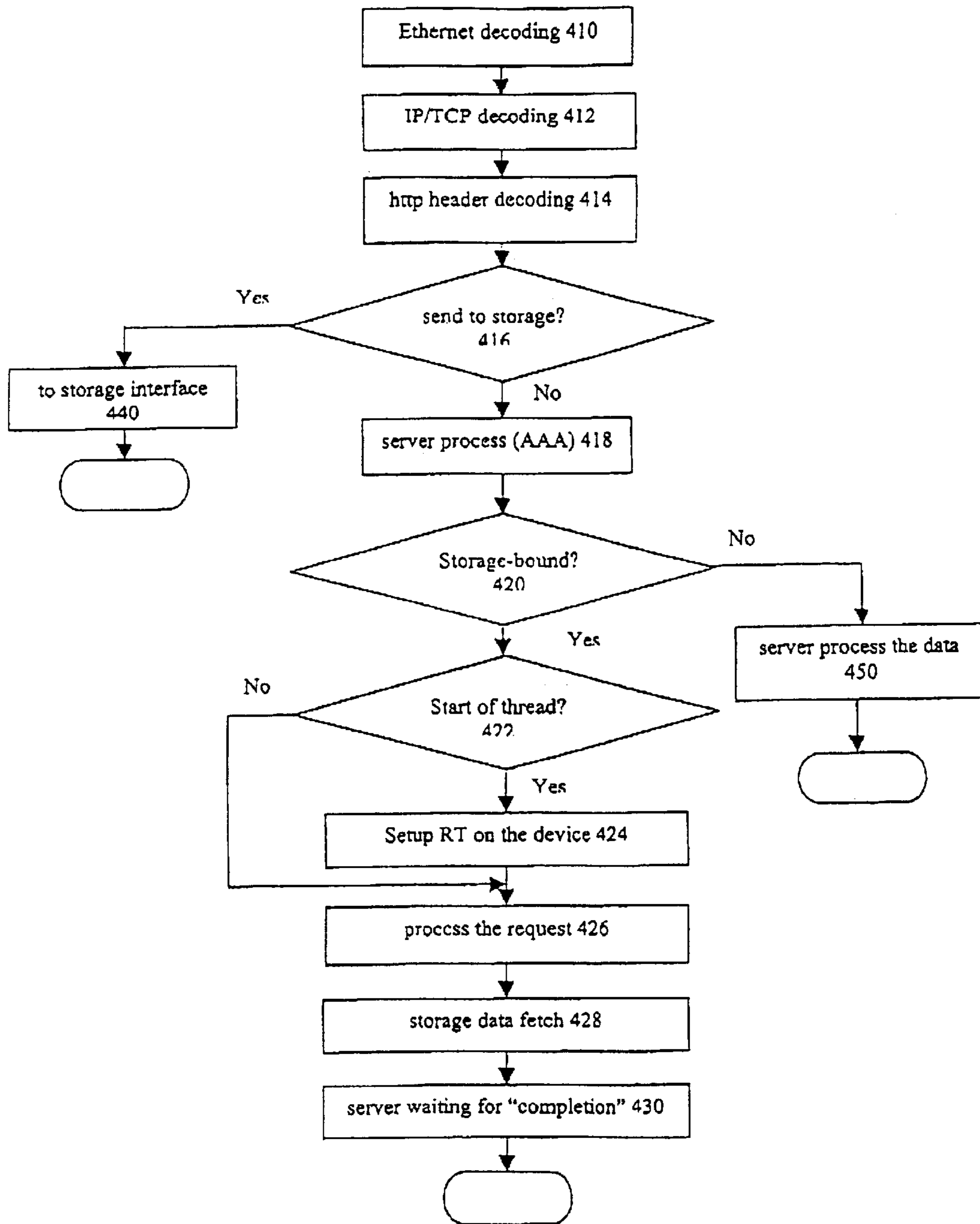
Figure 11 Traffic Flow from Network to Storage and Server
