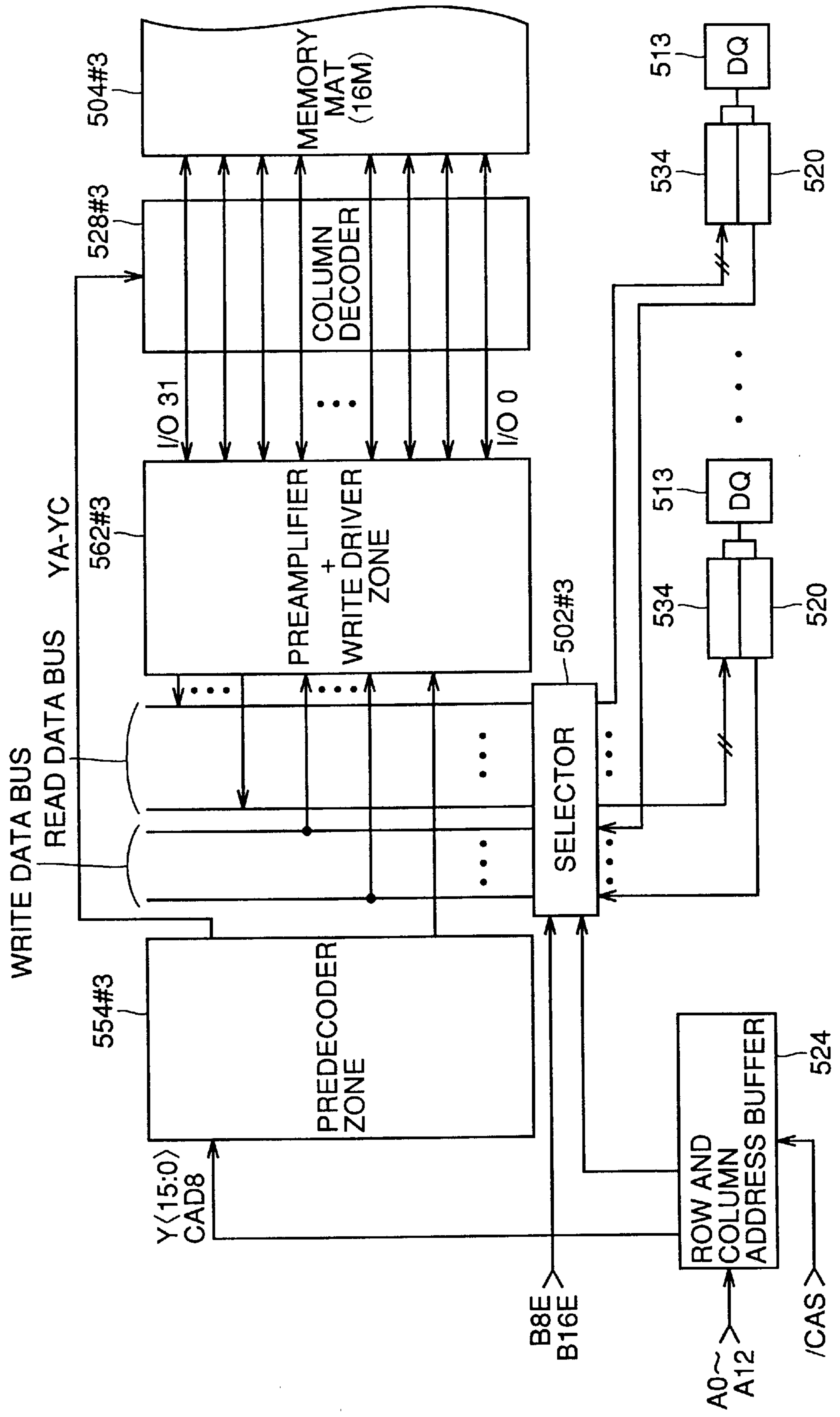
FIG. 30 PRIOR ART
