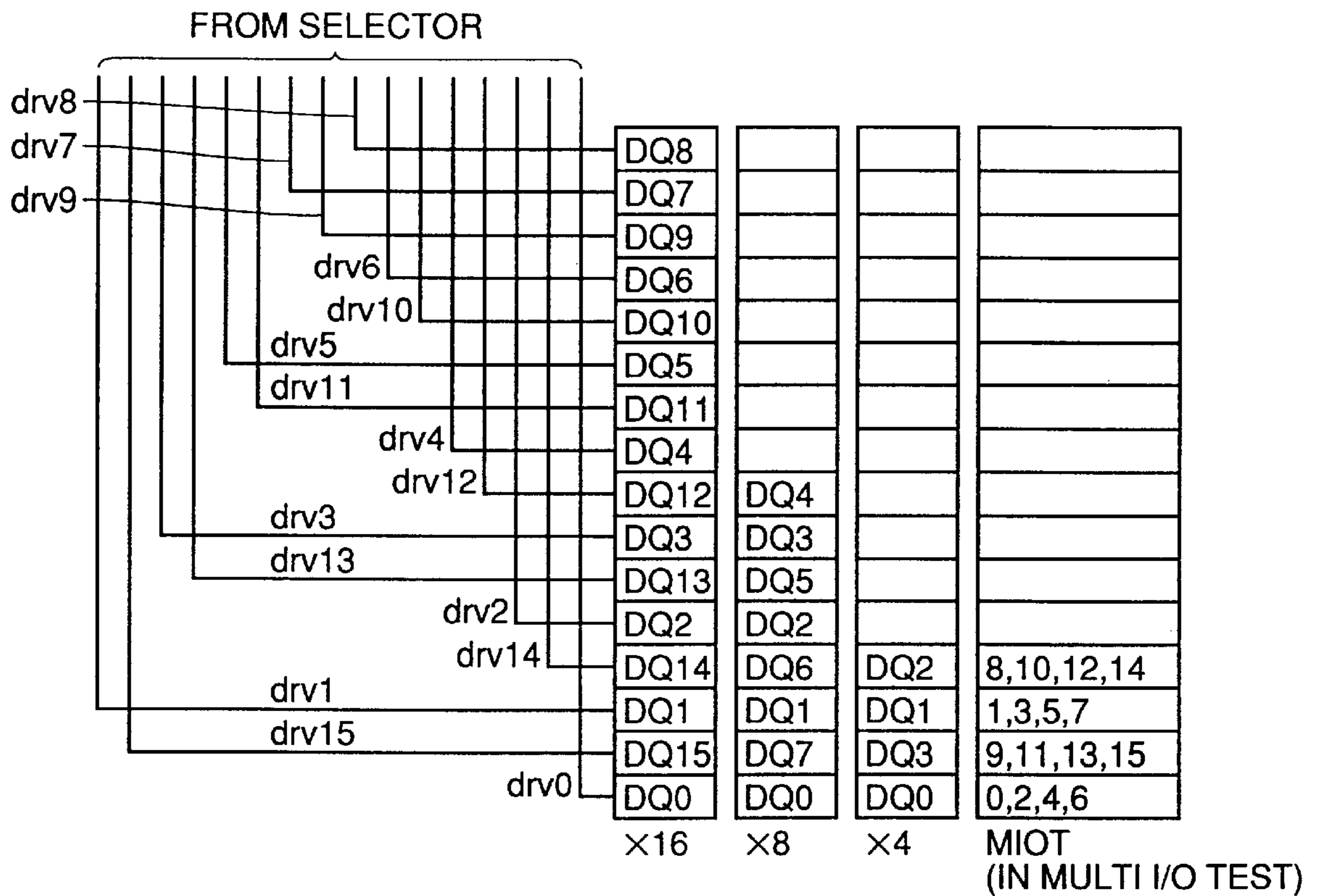
FIG.29 PRIOR ART
