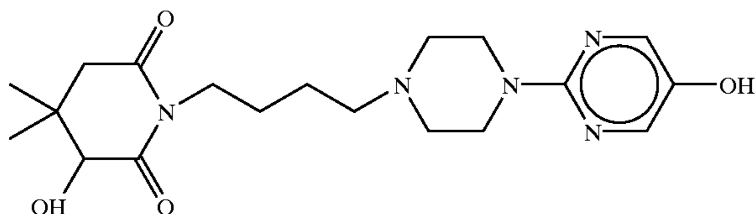
3,5-dihydroxy gepirone
