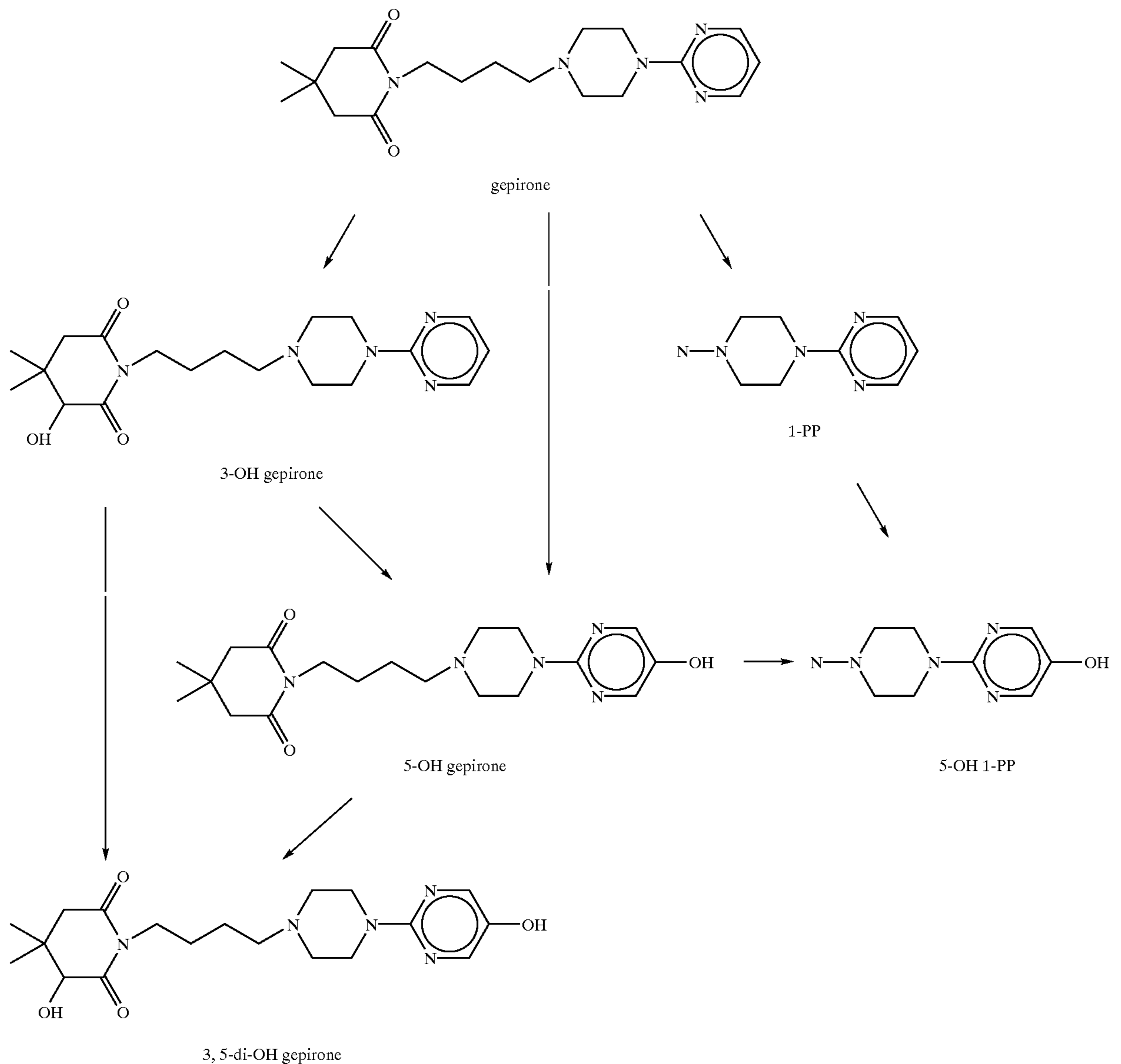
Scheme 1: Proposed Metabolic Scheme of Gepirone in Rats
