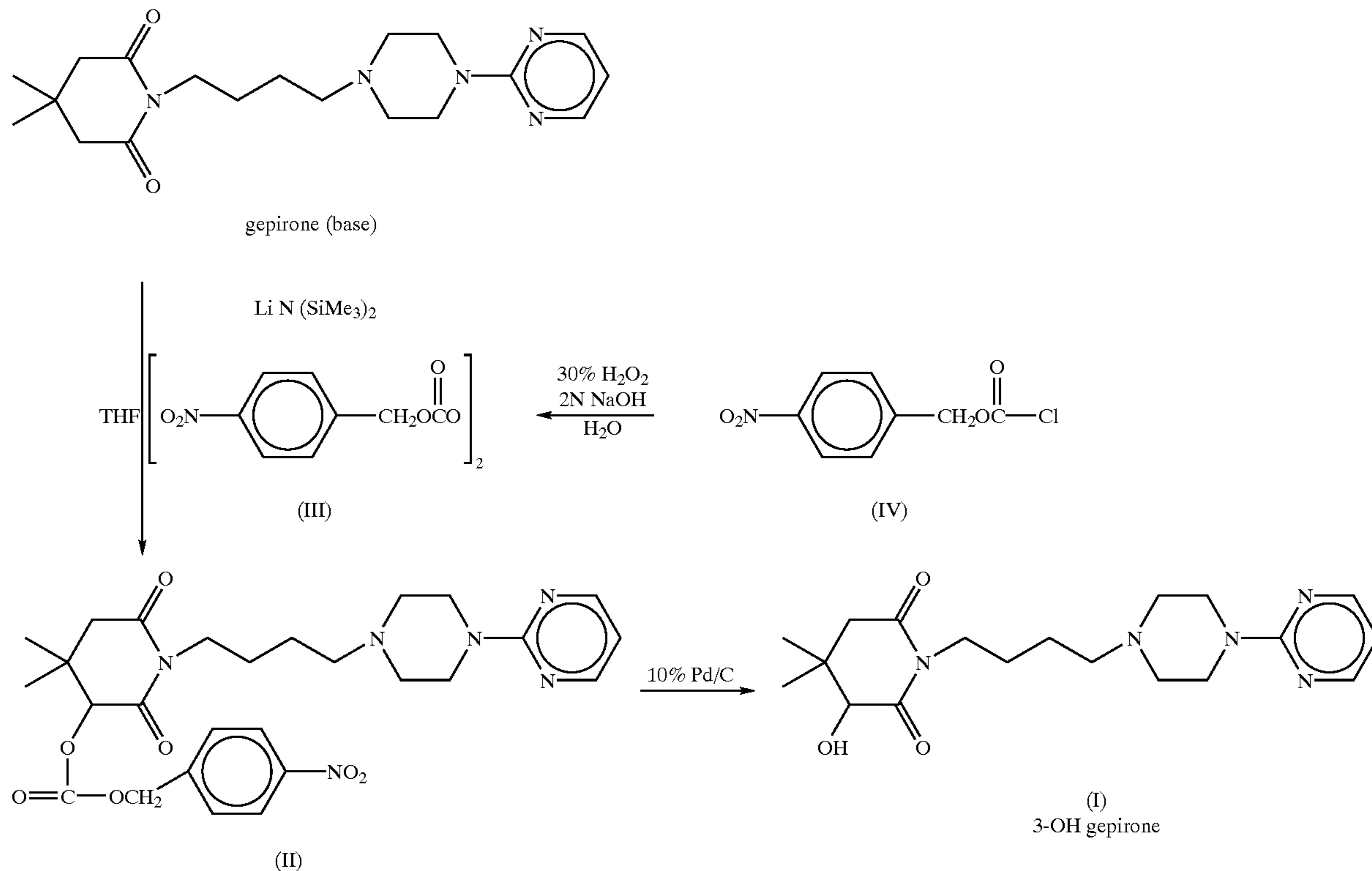
Scheme 2: Preparation of 3-OH Gepirone
