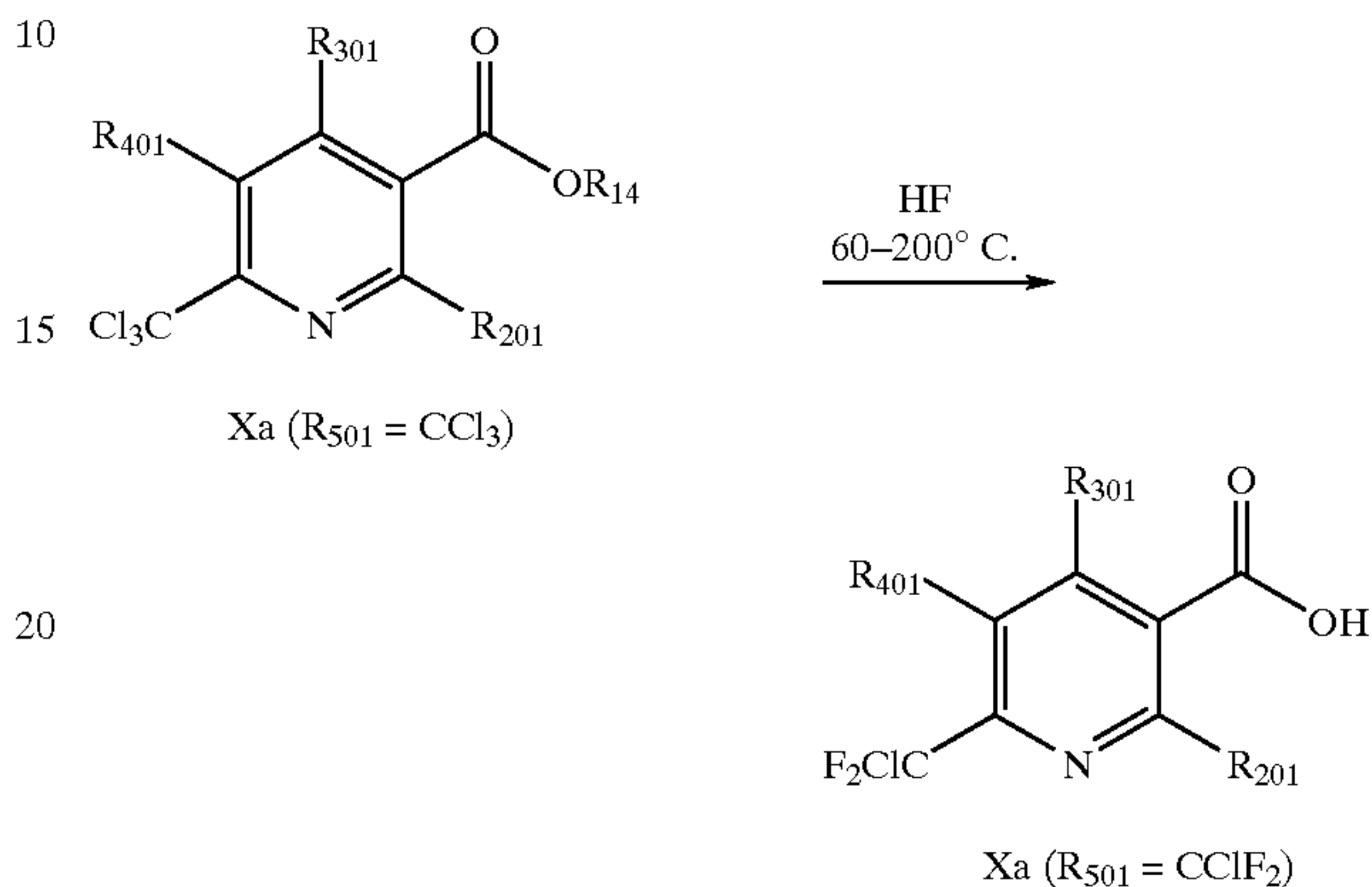
Reaction scheme 5
