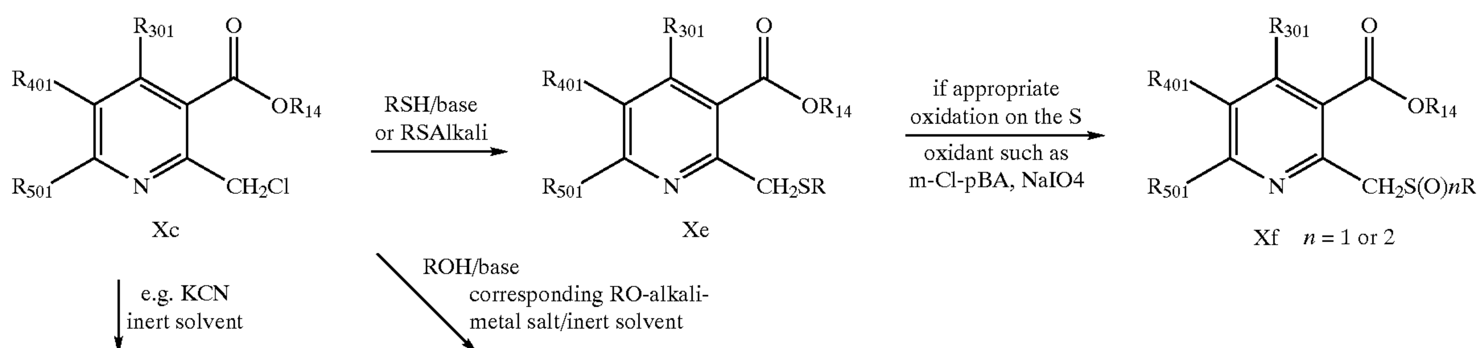
Reaction scheme 7
