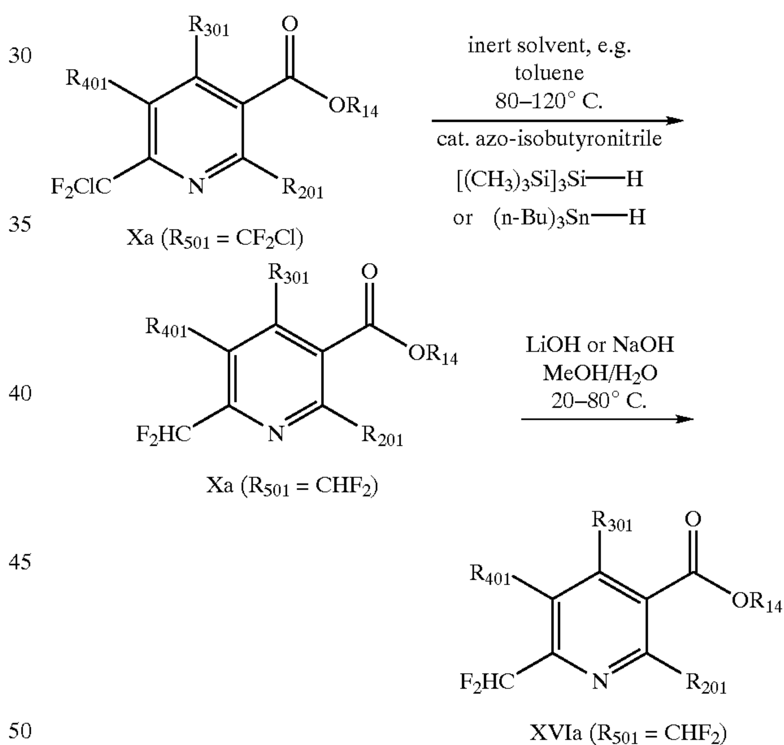
Reaction scheme 6
