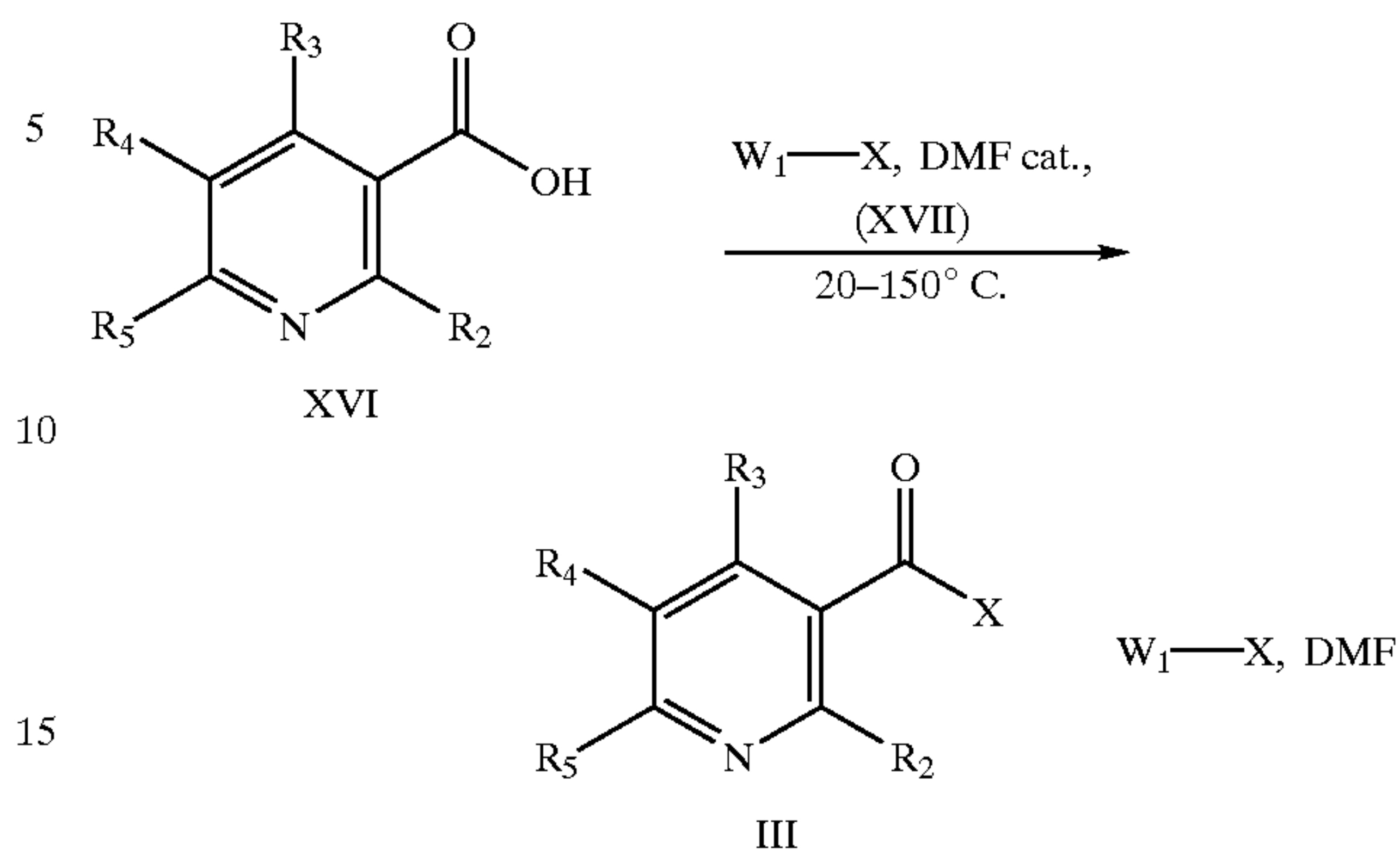
Reaction scheme 2
