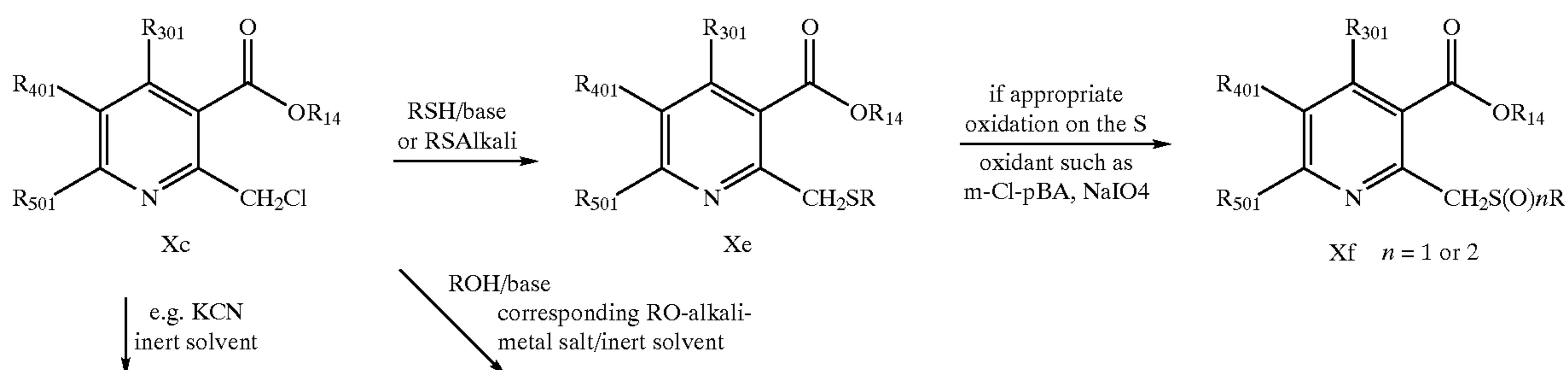
Reaction scheme 7
