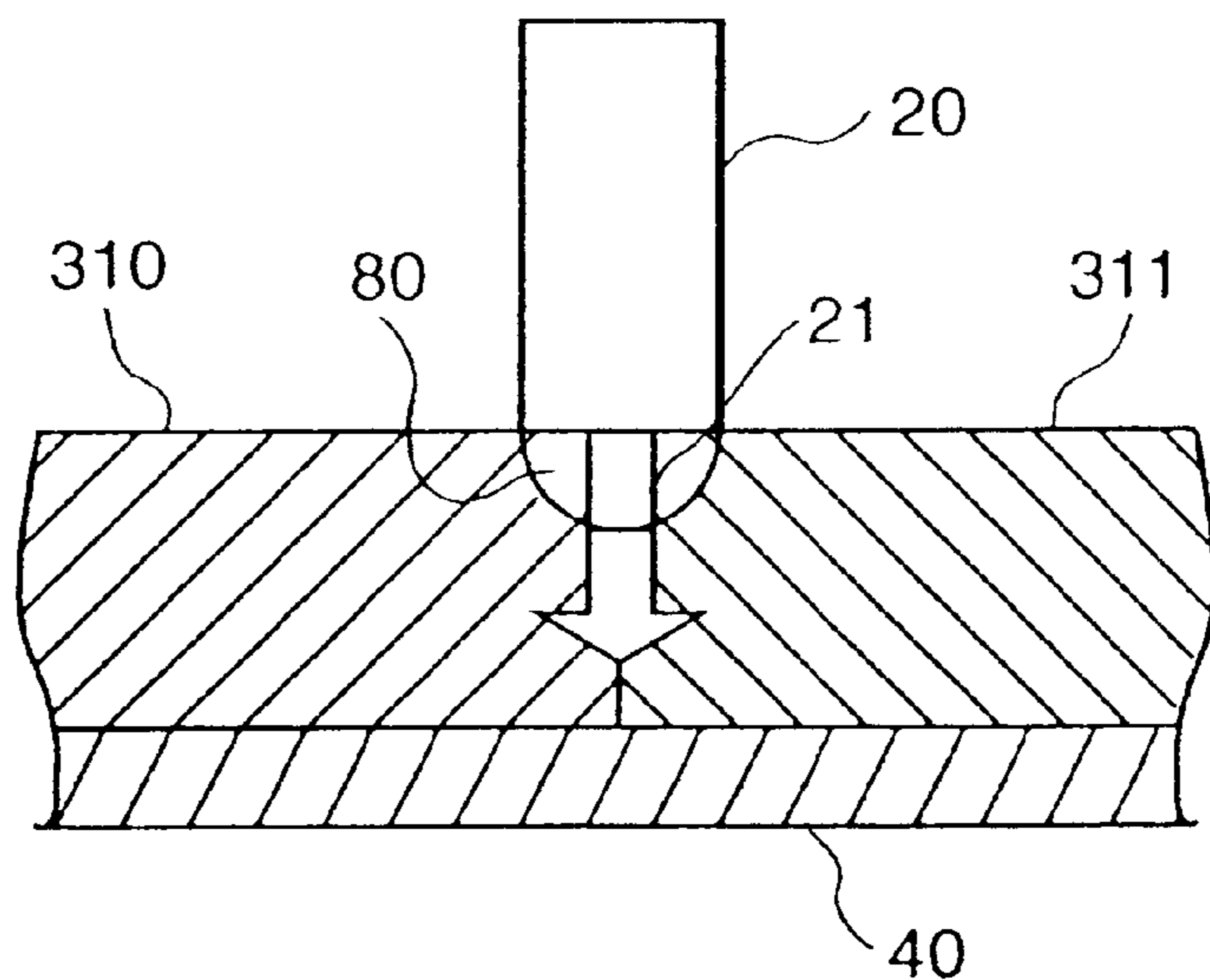
FIG. 19 (PRIOR ART)
