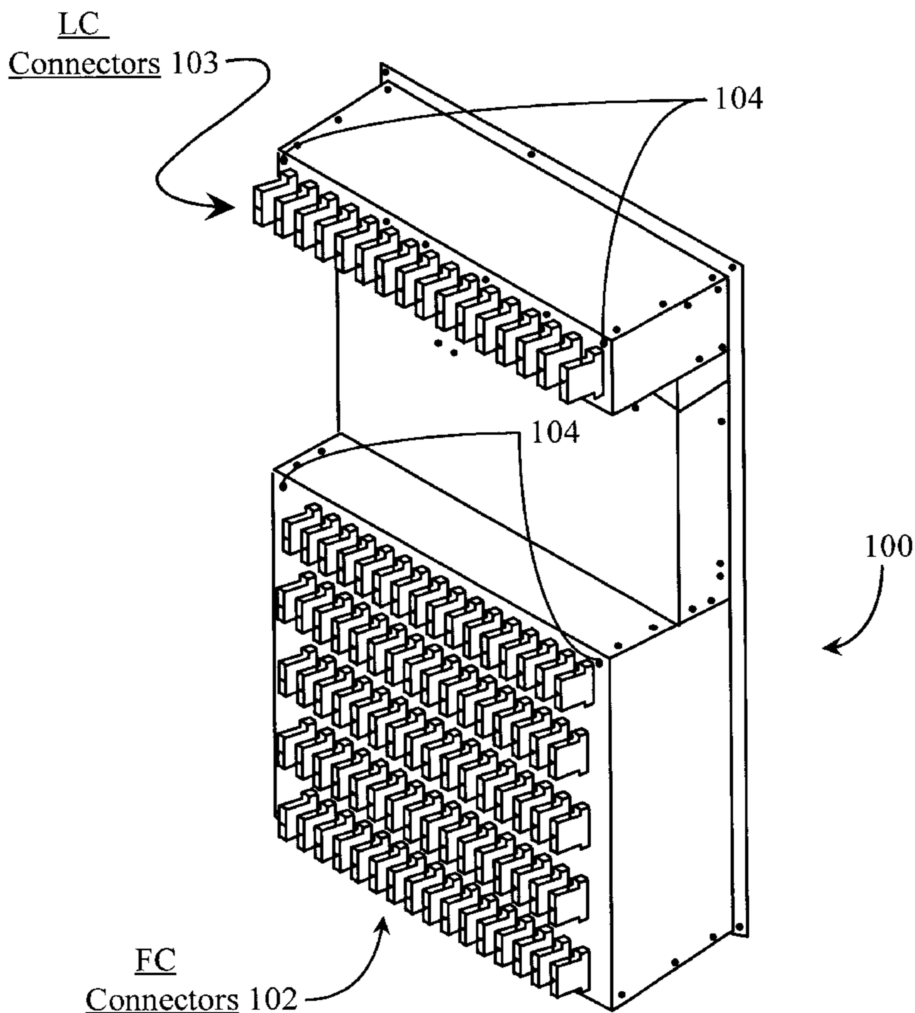
(Optical Backplane Assy.)
