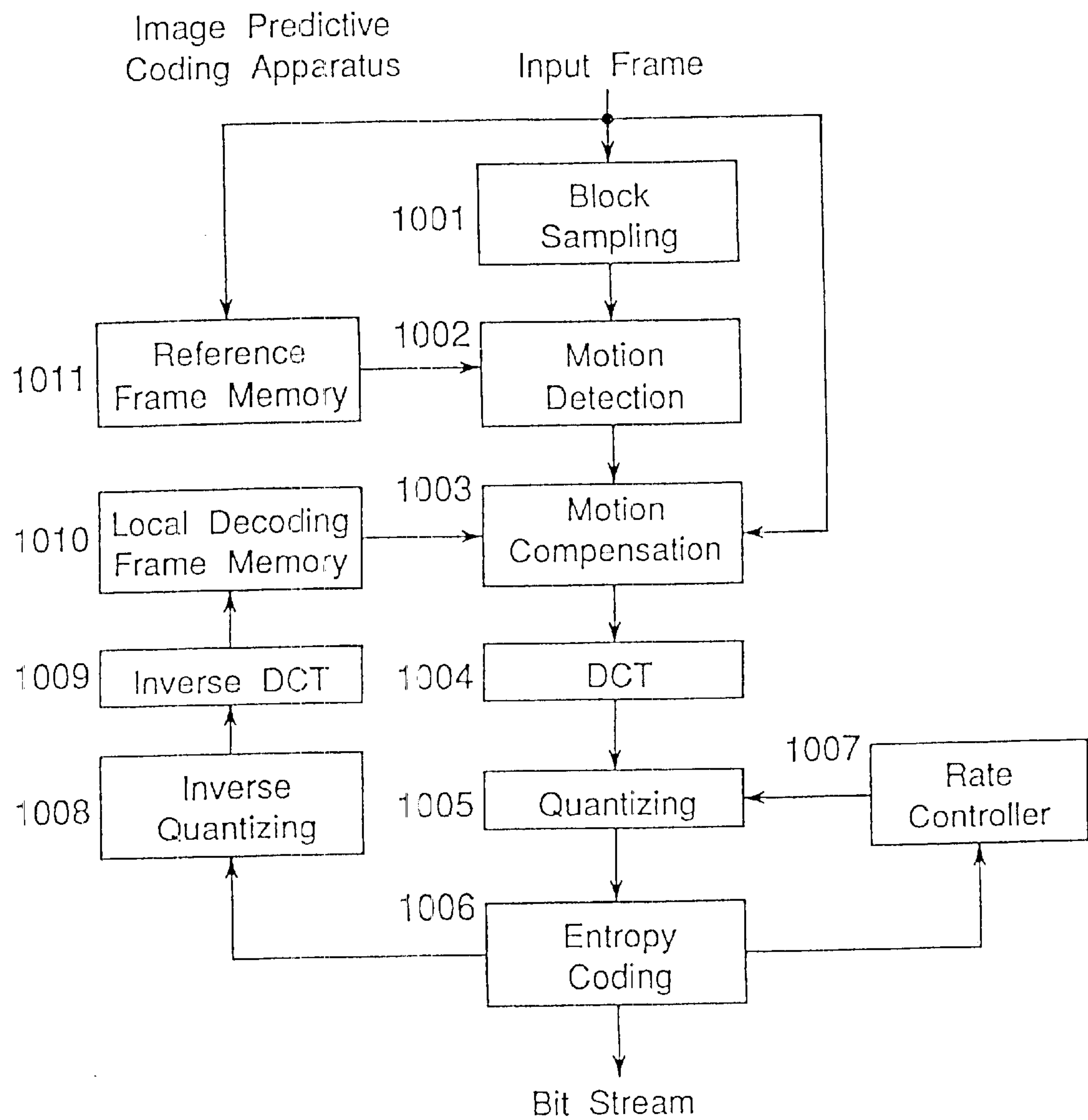
Fig.14 PRIOR ART
