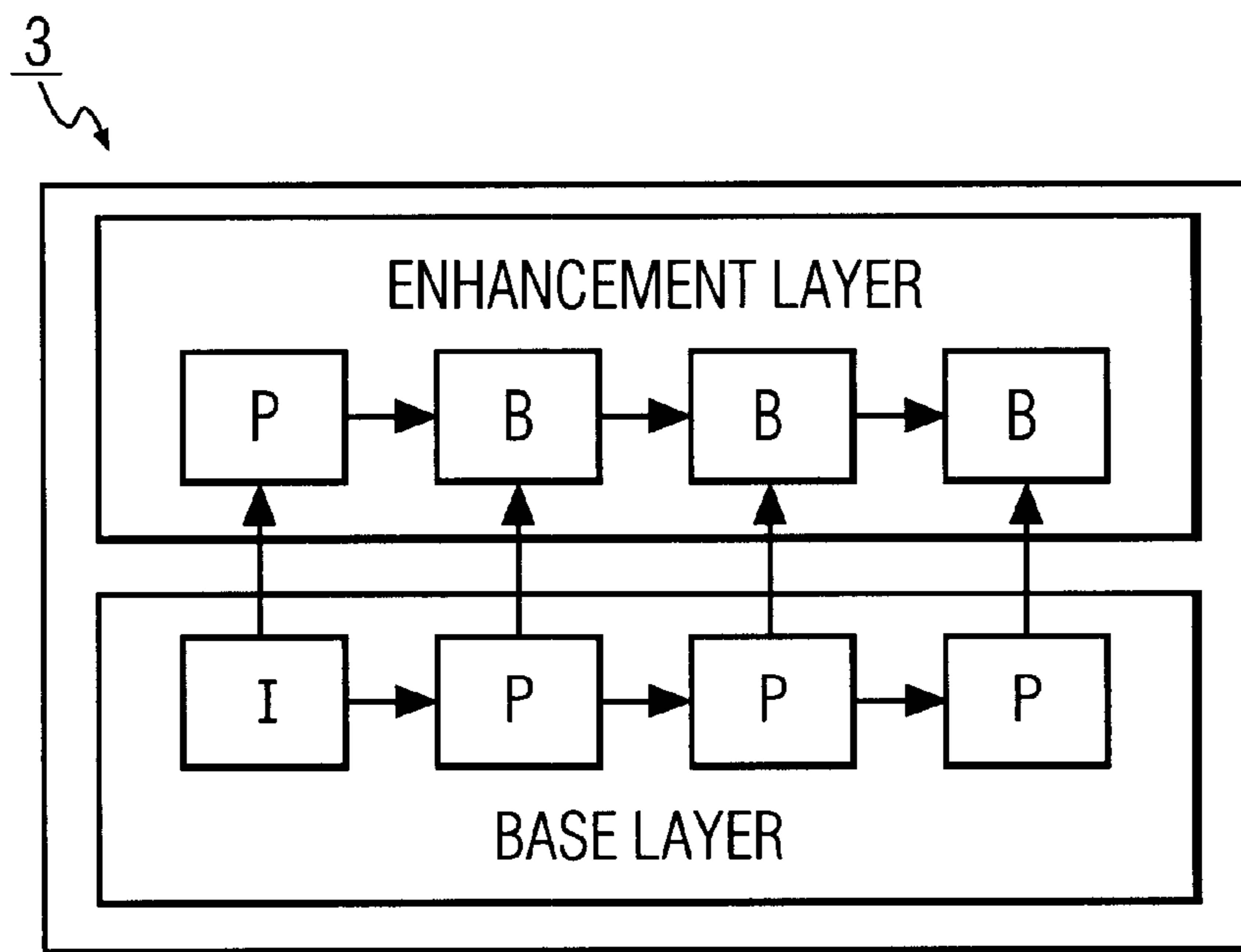
FIG. 2 (PRIOR ART)
