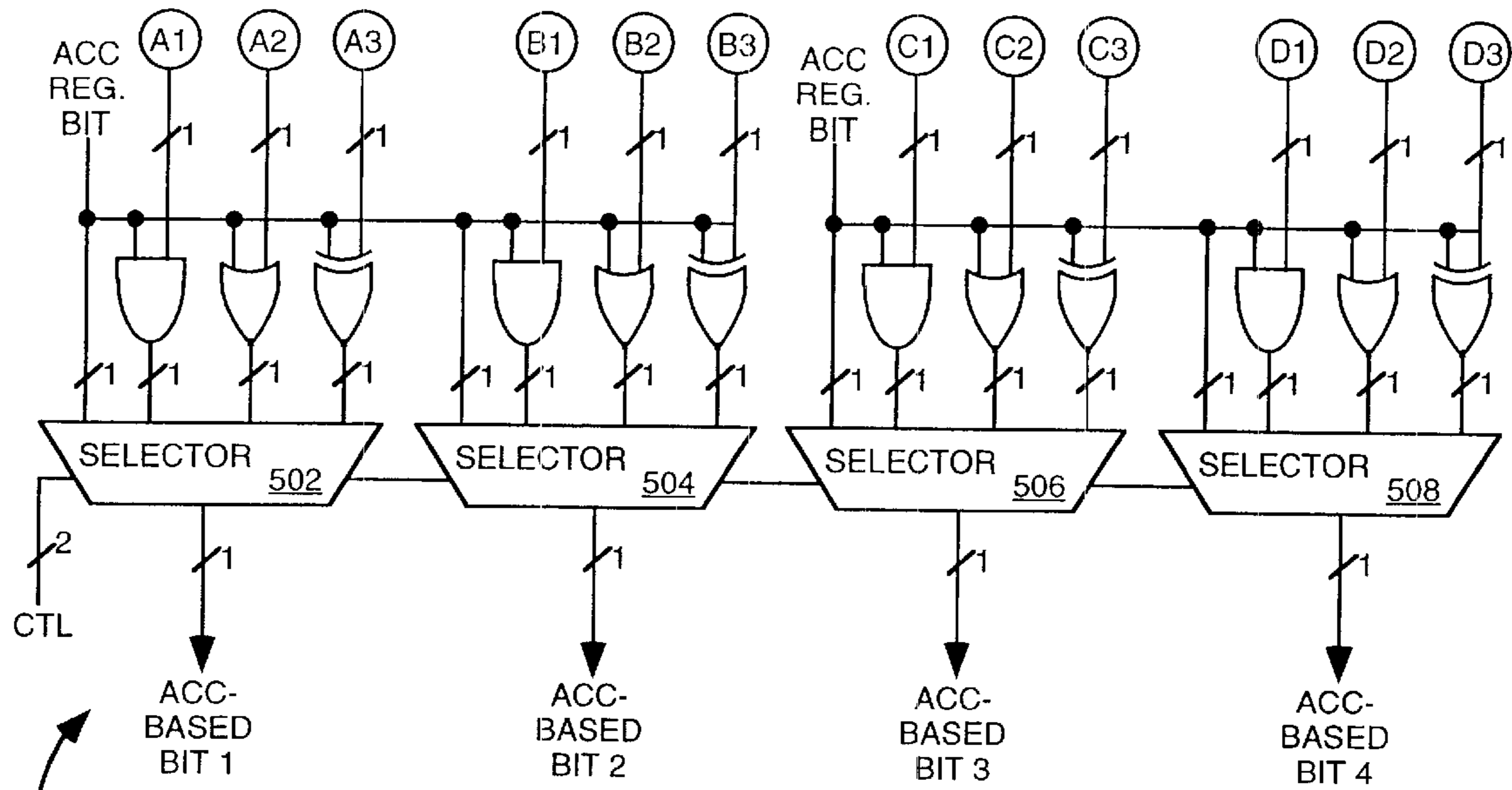
ACCUMULATOR BASED BIT GENERATION CIRCUIT 40
