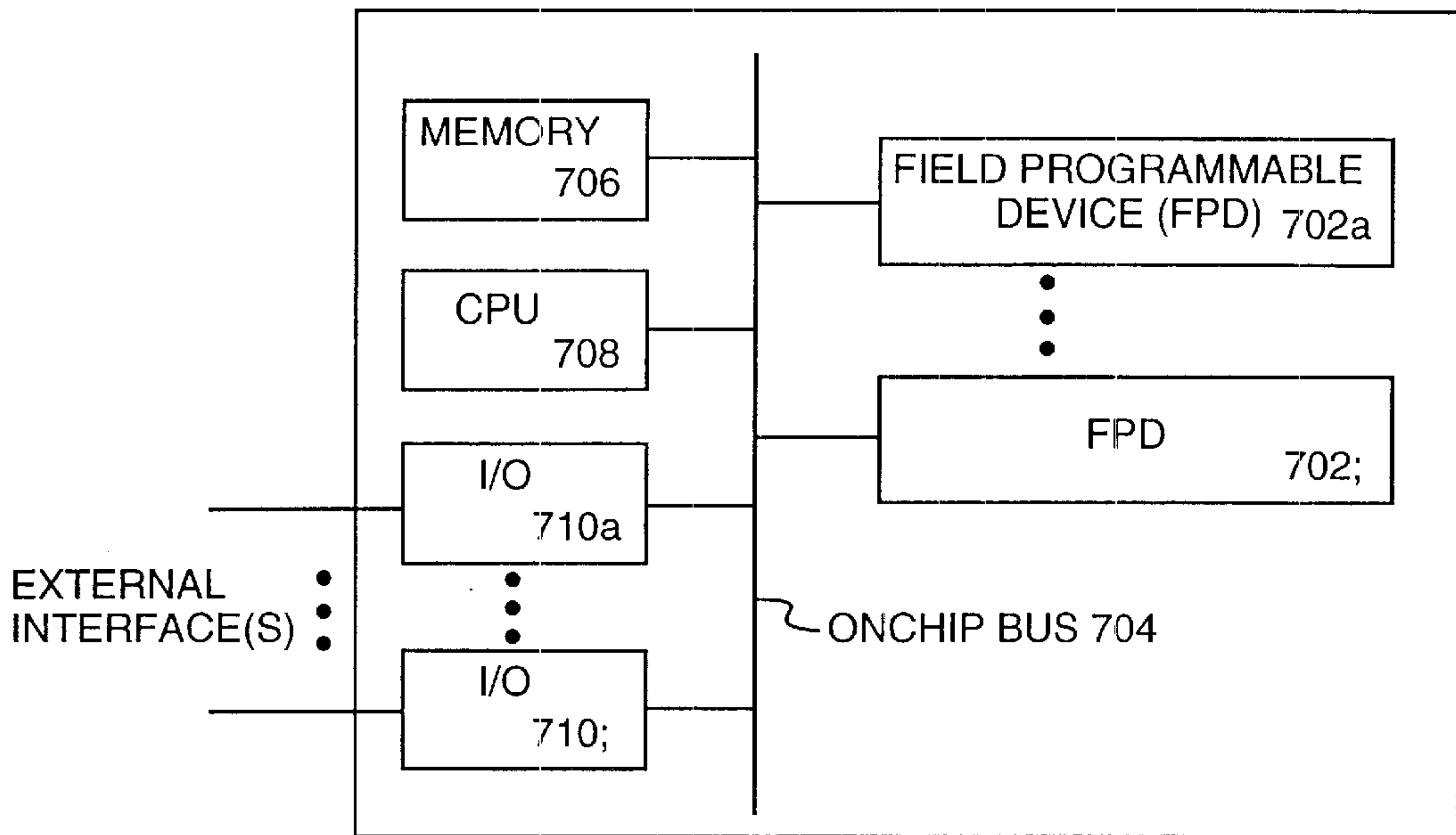
PROGRAMMABLE SYSTEM CHIP 700
