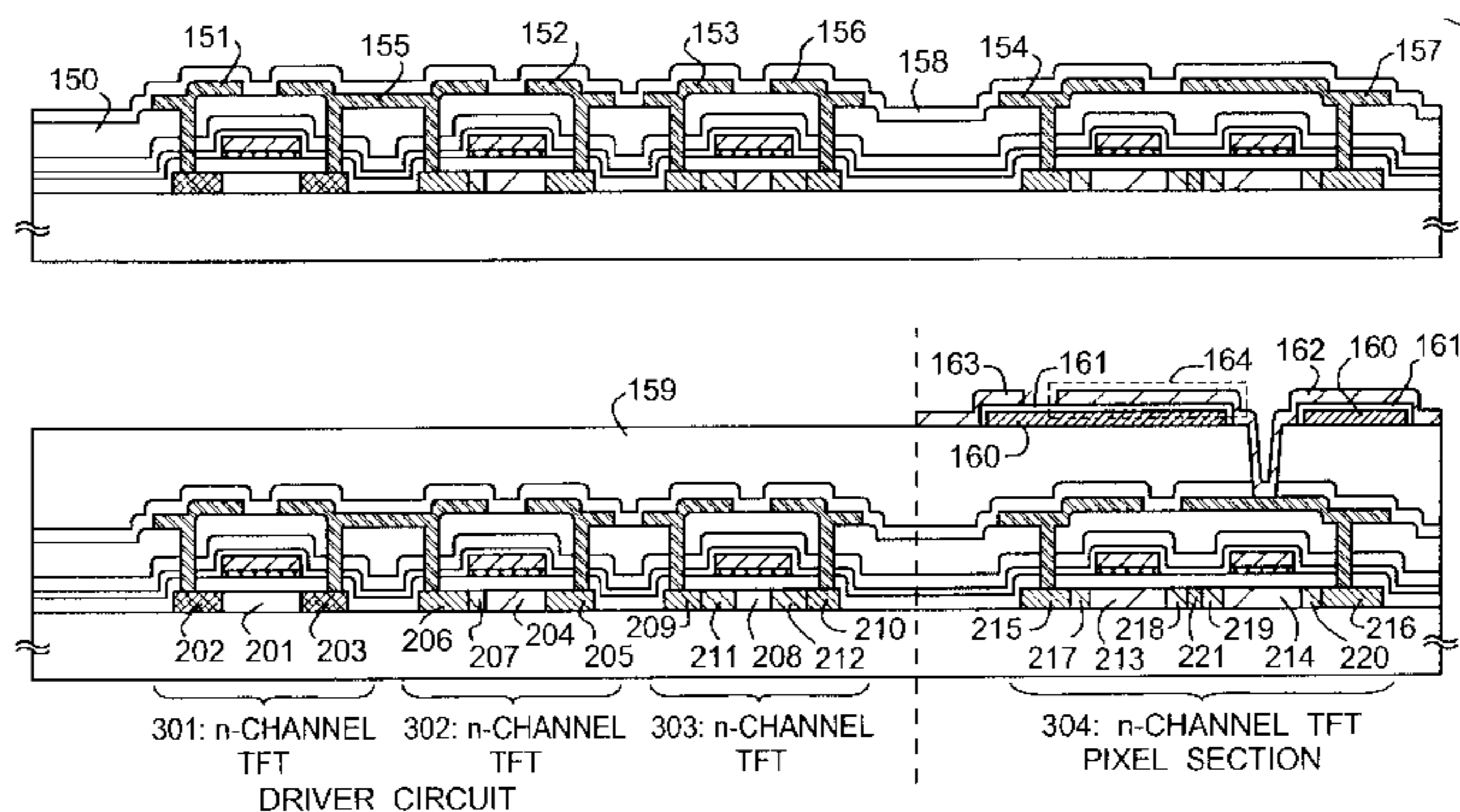
150: SECOND INTERLAYER INSULATING FILM 151-154: SOURCE WIRINGS 155-157: DRAIN WIRINGS 158: PASSIVATION FILM 159: THIRD INTERLAYER INSULATING FILM 160: SHIELDING FILM 161: ANODIC OXIDE 162,163: PIXEL ELECTRODES 164: STORAGE CAPACITOR 201,204,208,213,214: CHANNEL FORMING REGIONS 202,205,209,215: SOURCE REGIONS 203,206,210,216: DRAIN REGIONS 207,211,212: n-TYPE IMPURITY REGIONS (b) 217-120: n-TYPE IMPURITY REGIONS (c) 221: n-TYPE IMPURITY REGION (a)
