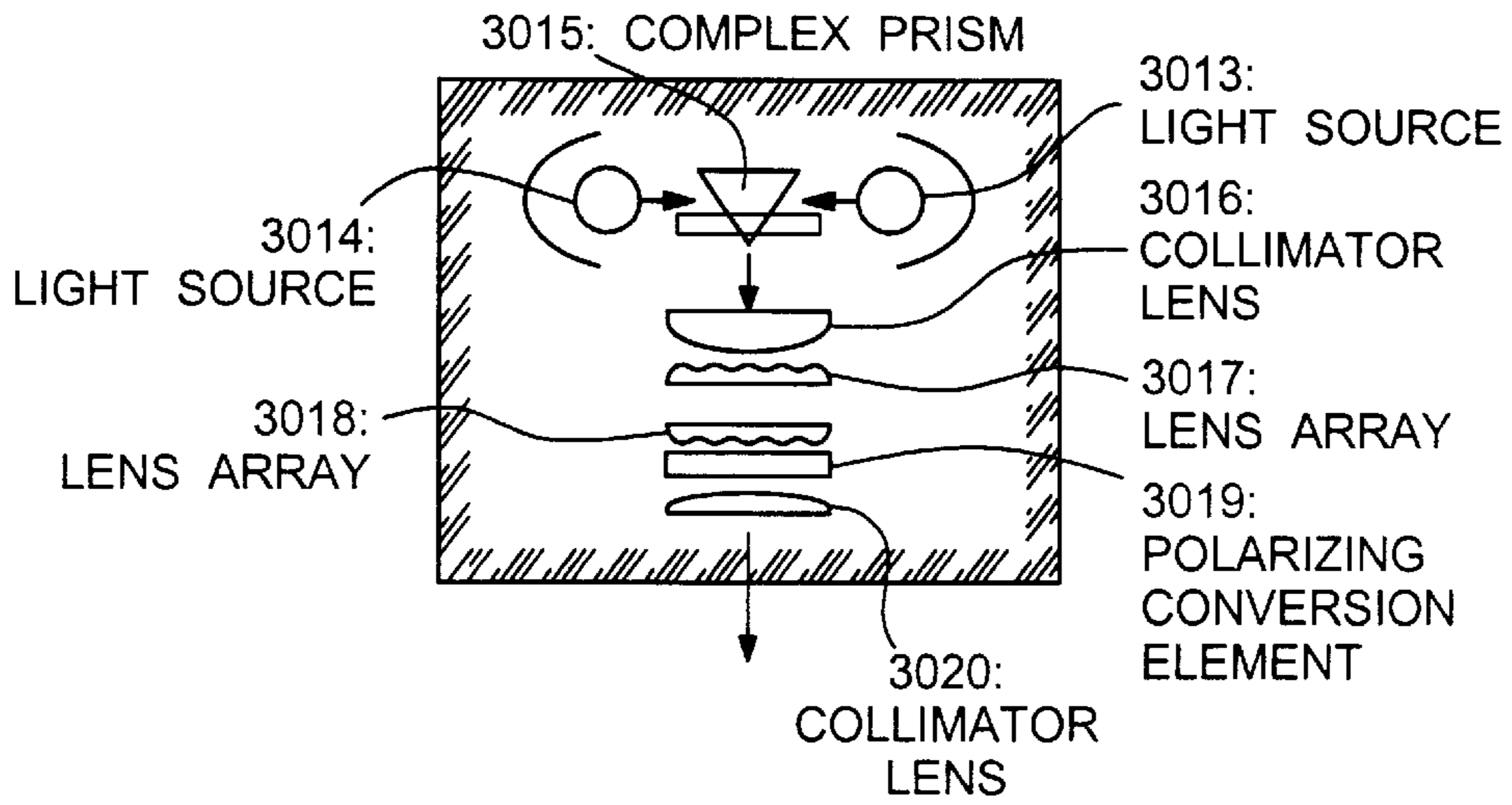
FIG. 25(B): OPTICAL LIGHT SOURCE SYSTEM (3-PLATE TYPE)
