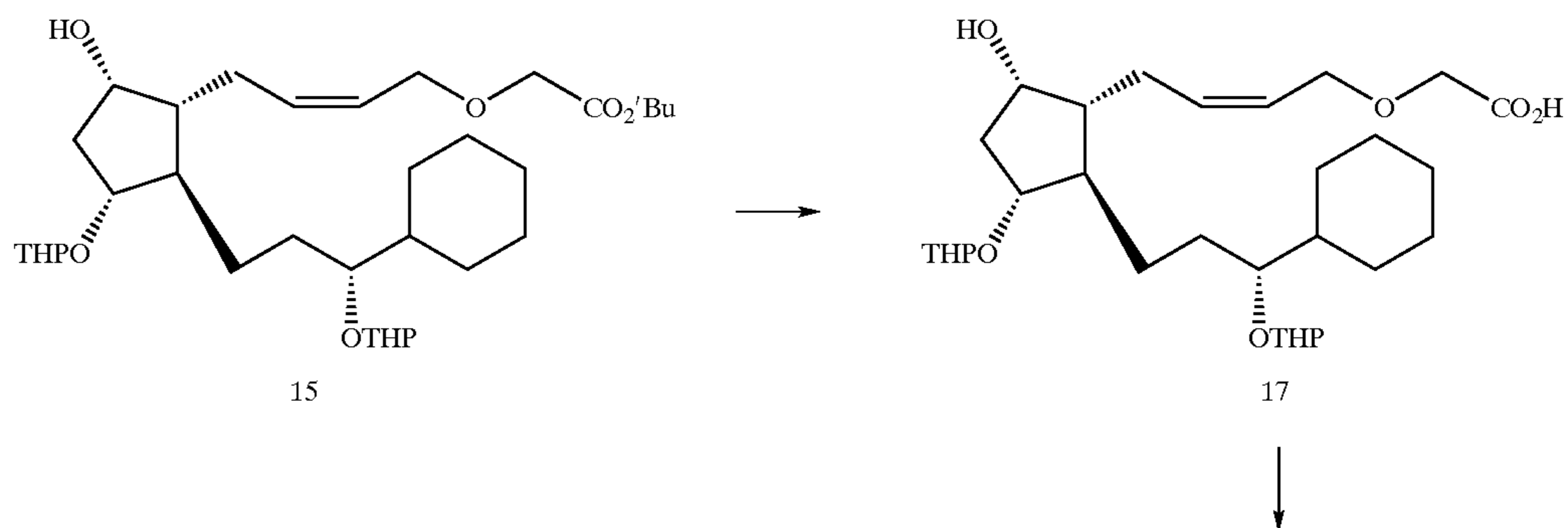
SCHEME II: SYNTHESIS OF COMPOUND (III)
