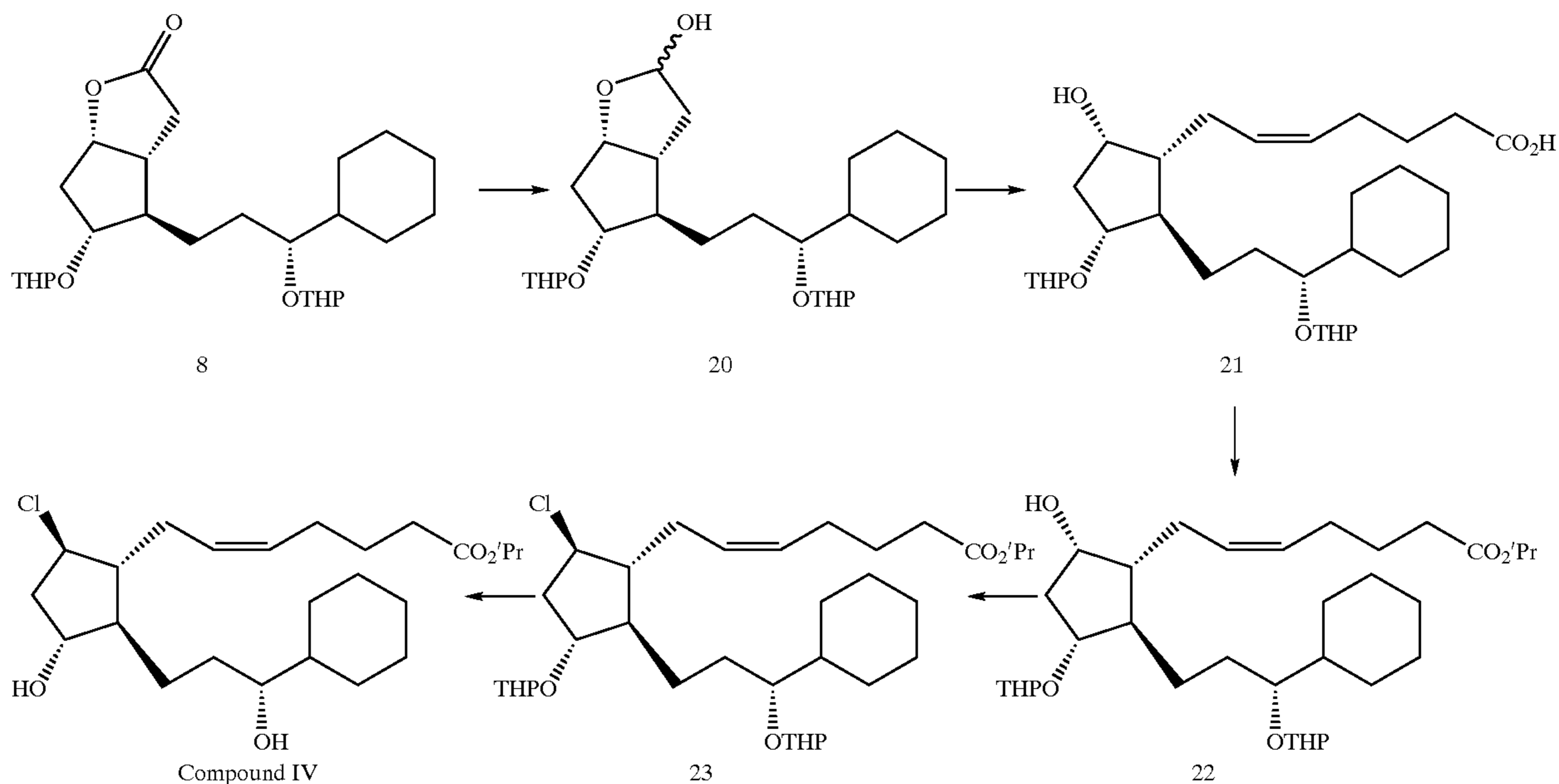
SCHEME III: SYNTHESIS OF COMPOUND (IV)
