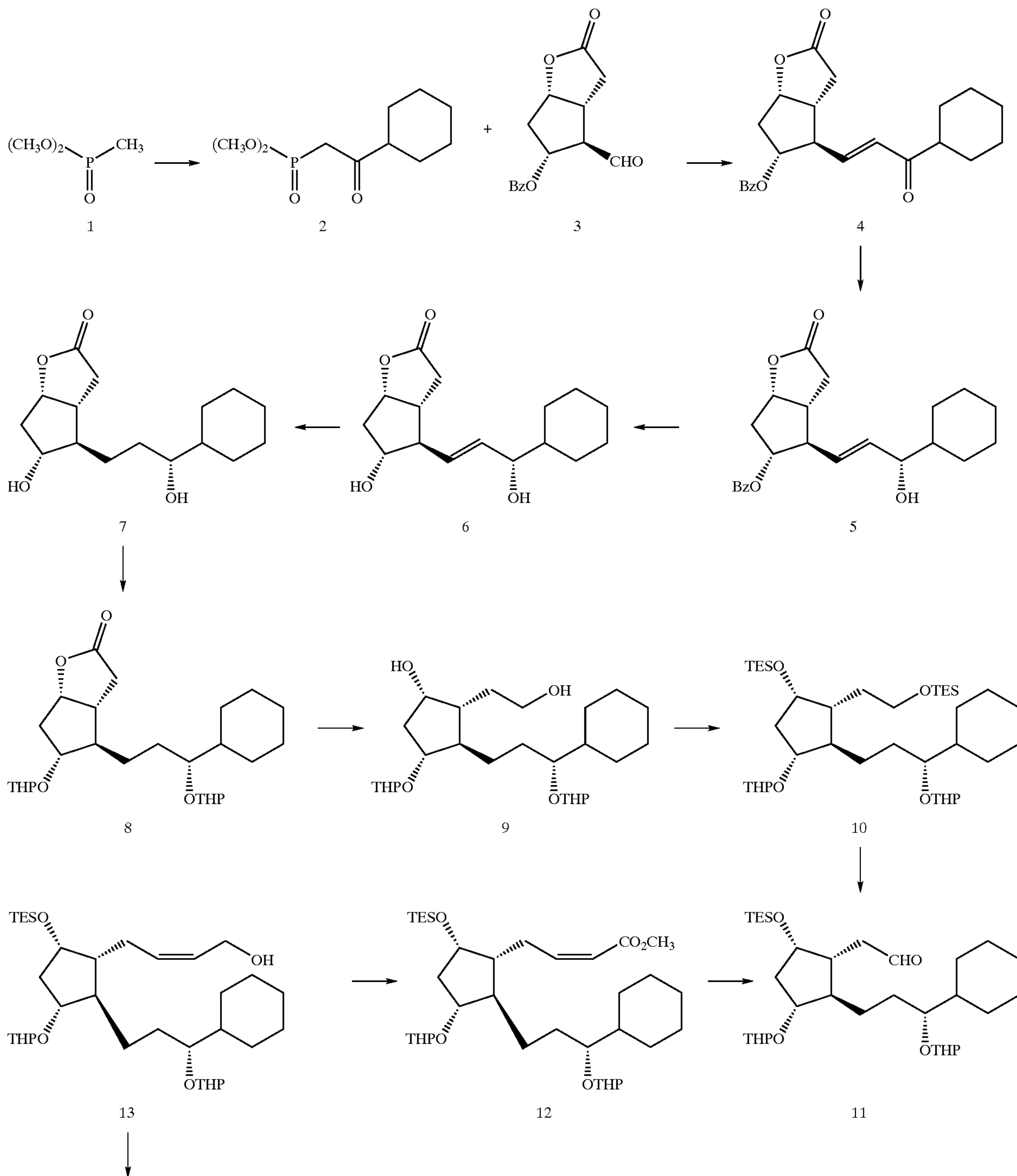
SCHEME I: SYNTHESIS OF COMPOUND (II)
