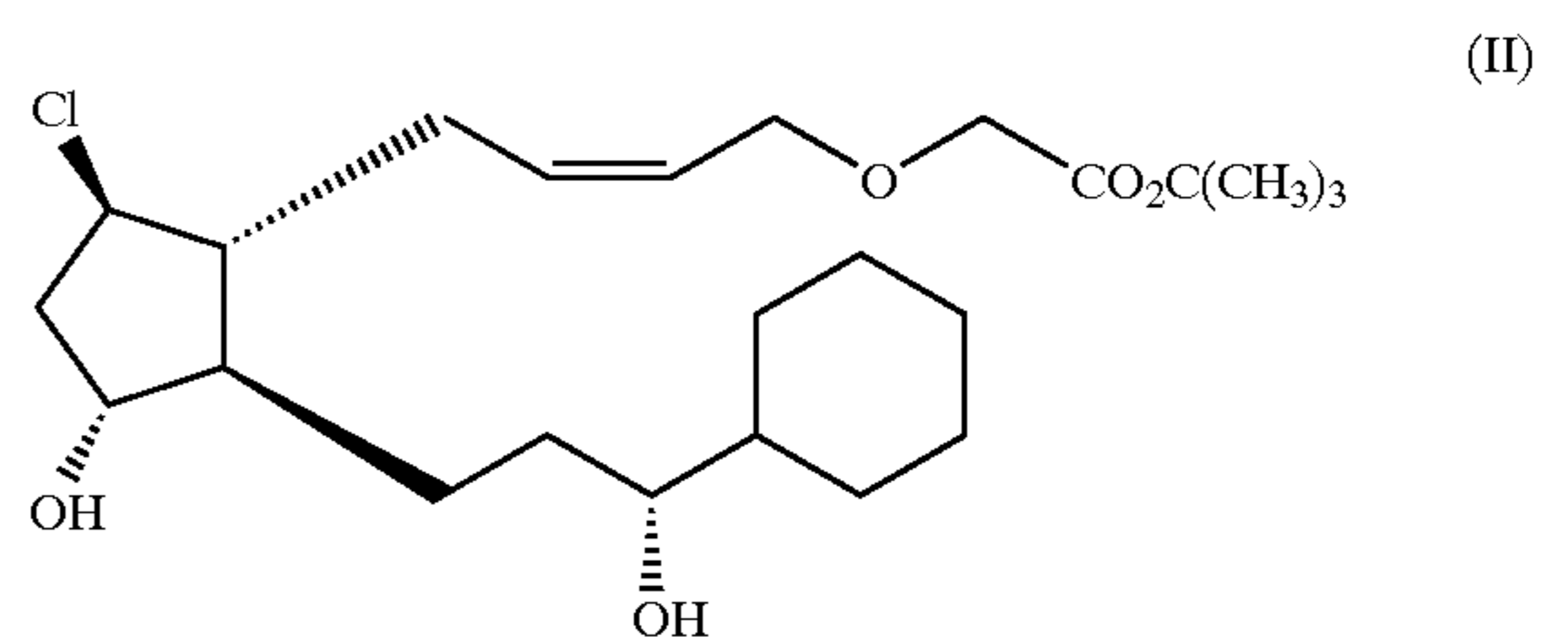
(5Z)-(9R, 11R, 15R)-9-Chloro-15-cyclohexyl-11,15-dihydroxy-3-oxa-16,17,18,19,20-pentanoic Acid t-Butyl Ester
