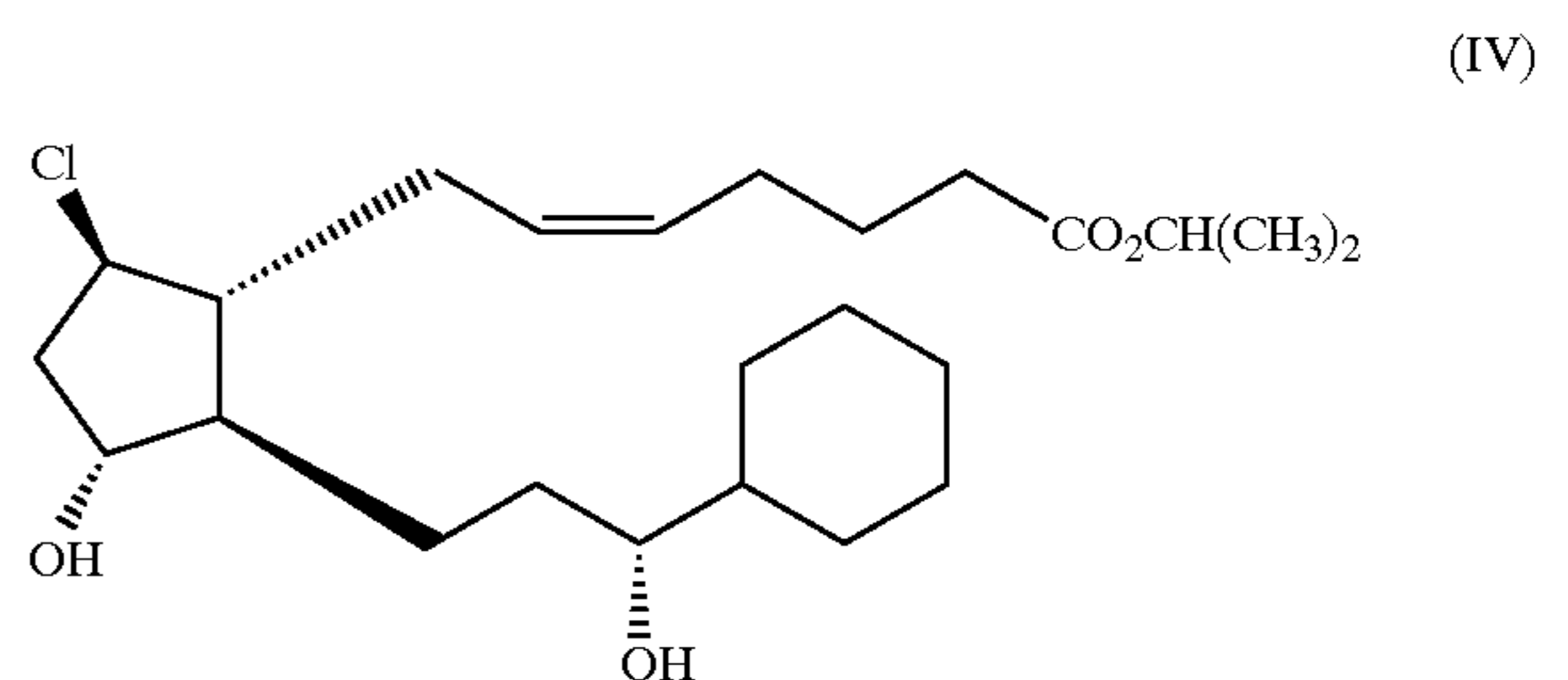
(5Z)-(9R, 11R, 15R)-9-Chloro-15-cyclohexyl-11,15-dihydroxy-3-oxa-16,17,18,19,20-pentanoic Acid Isopropyl Ester
