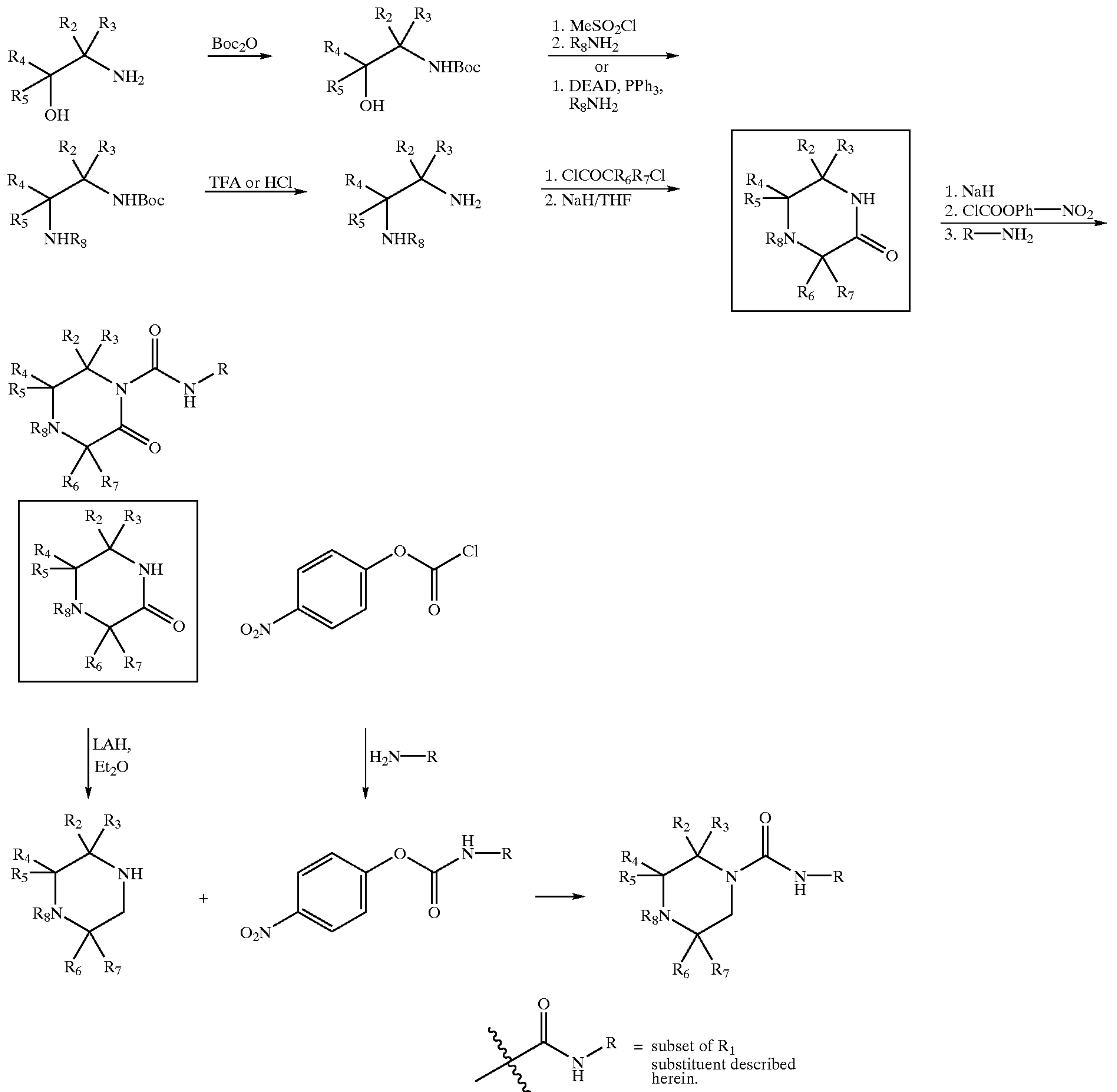
Scheme 13: General Synthesis of Piperizines and piperizinones
