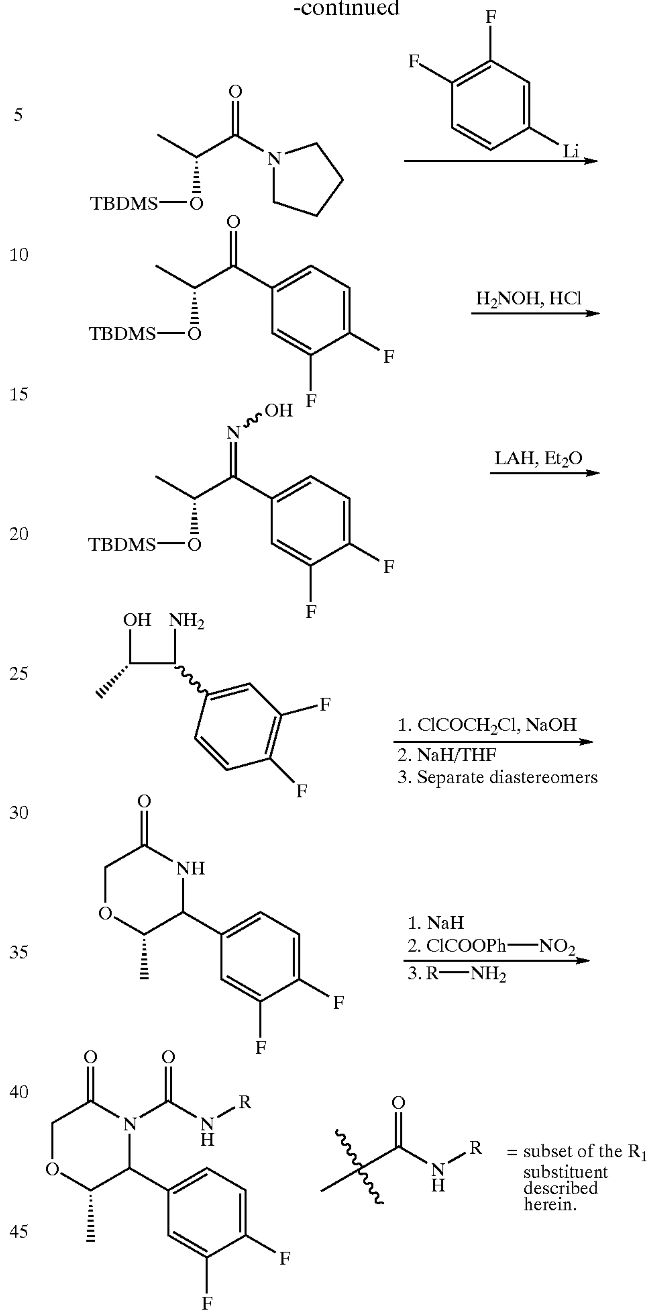
Scheme 4a: Synthesis of Substituted Morpholinone Examples.
