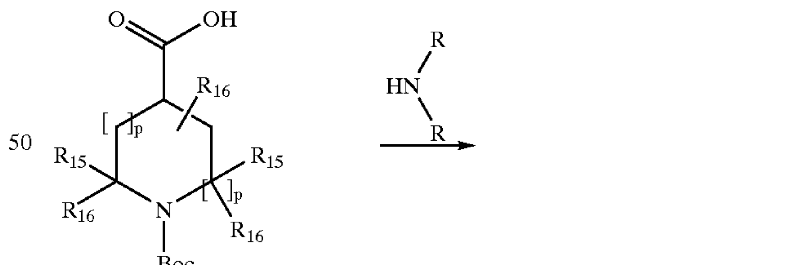
Scheme 21: General Synthesis of Compounds
