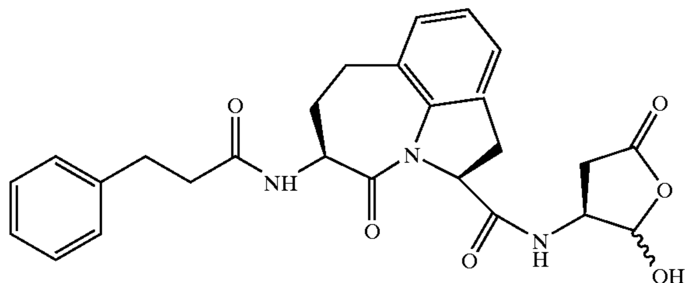
(2S-cis)-[5-Dihydrocinnamylamino-1,2,3,4,5,6,7-hexahydro-4-oxoazepino[3,2,1-hi]indole-2-carbonyl)-amino]-4-oxo-butanoic Acid
