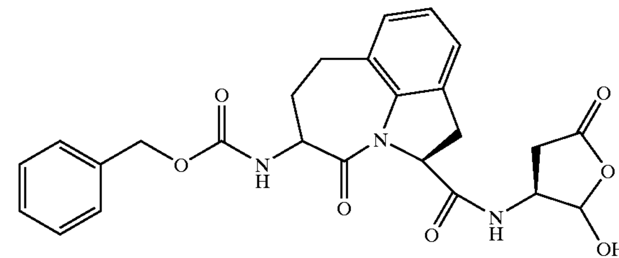
(2S-cis)-[5-Benzyloxycarbonylamino-1,2,4,5,6,7-hexahydro-4-oxoazepino[3,2,1-hi]indole-2-carbonyl)-amino]-4-oxo-butanoic Acid
