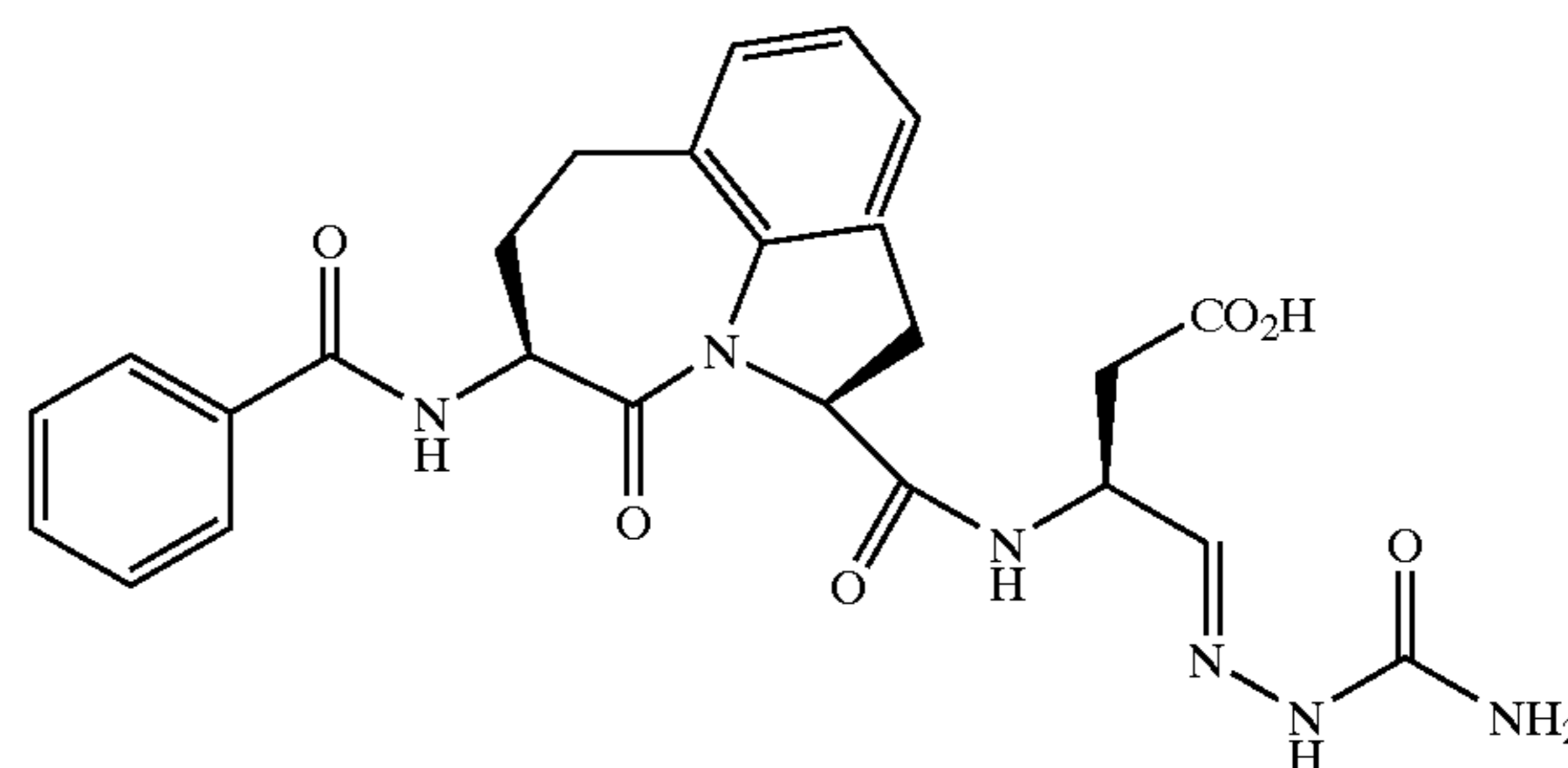
(2S-cis)-[5-Benzoylamino-1,2,3,4,5,6,7-hexahydro-4-oxoazepino[3,2,1-hi]indole-2-carbonyl)-amino]-4-oxo-butanoic Acid Semicarbazone
