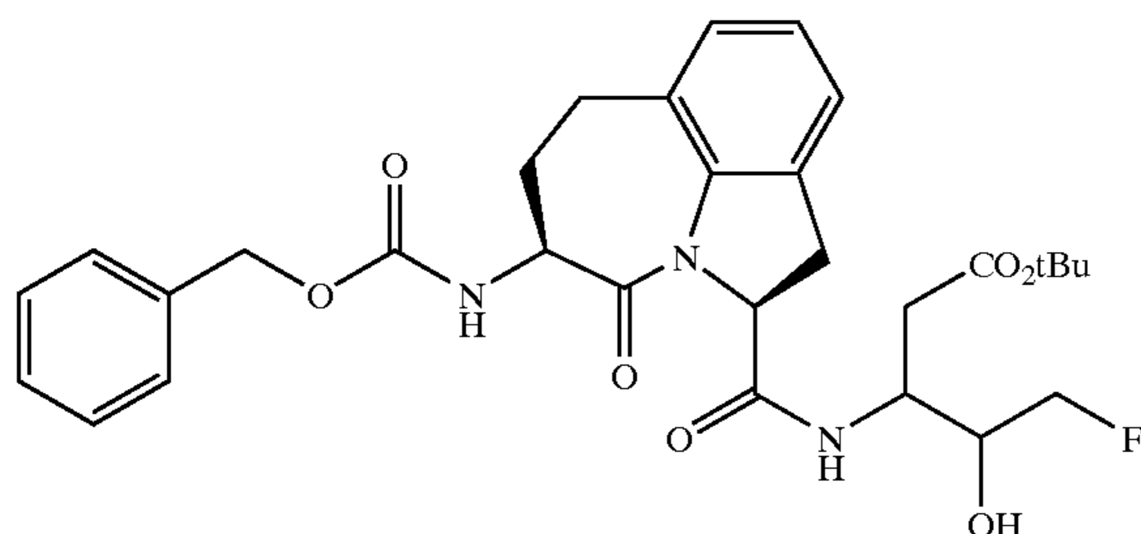
3{(2S-cis)-[5-Benzyloxycarbonylamino-1,2,3,4,5,6,7-hexahydro-4-oxoazepino[3,2,1-hi]indole-2-carbonyl)-amino]}-5-fluoro-4-hydroxy-pentanoic Acid tert-Butyl Ester
