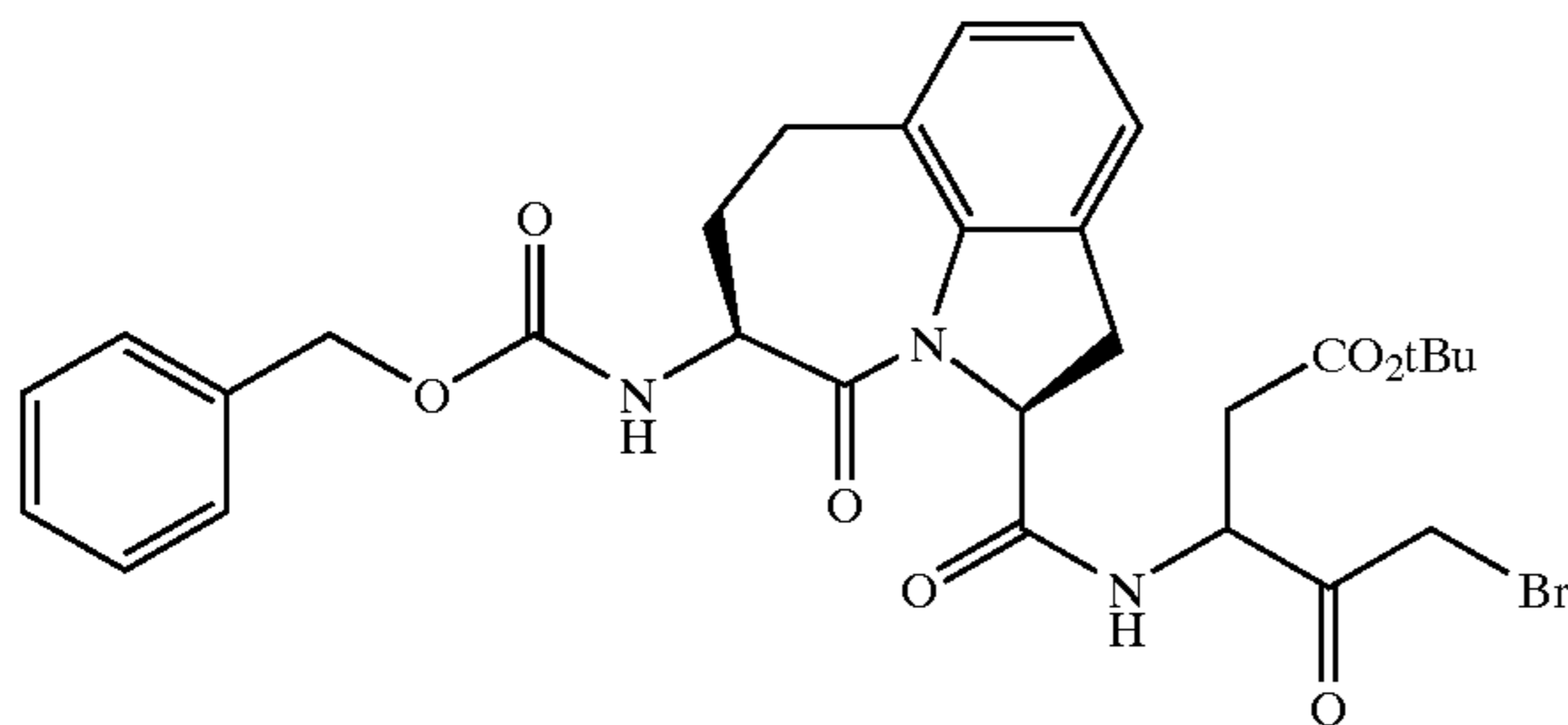
3-[(2S-cis)-[5-Benzyloxycarbonylamino-1,2,3,4,5,6,7-hexahydro-4-oxoazepino[3,2,1-hi]indole-2-carbonyl]amino]-5-bromo-4-oxo-pentanoic Acid, tert-Butyl Ester
