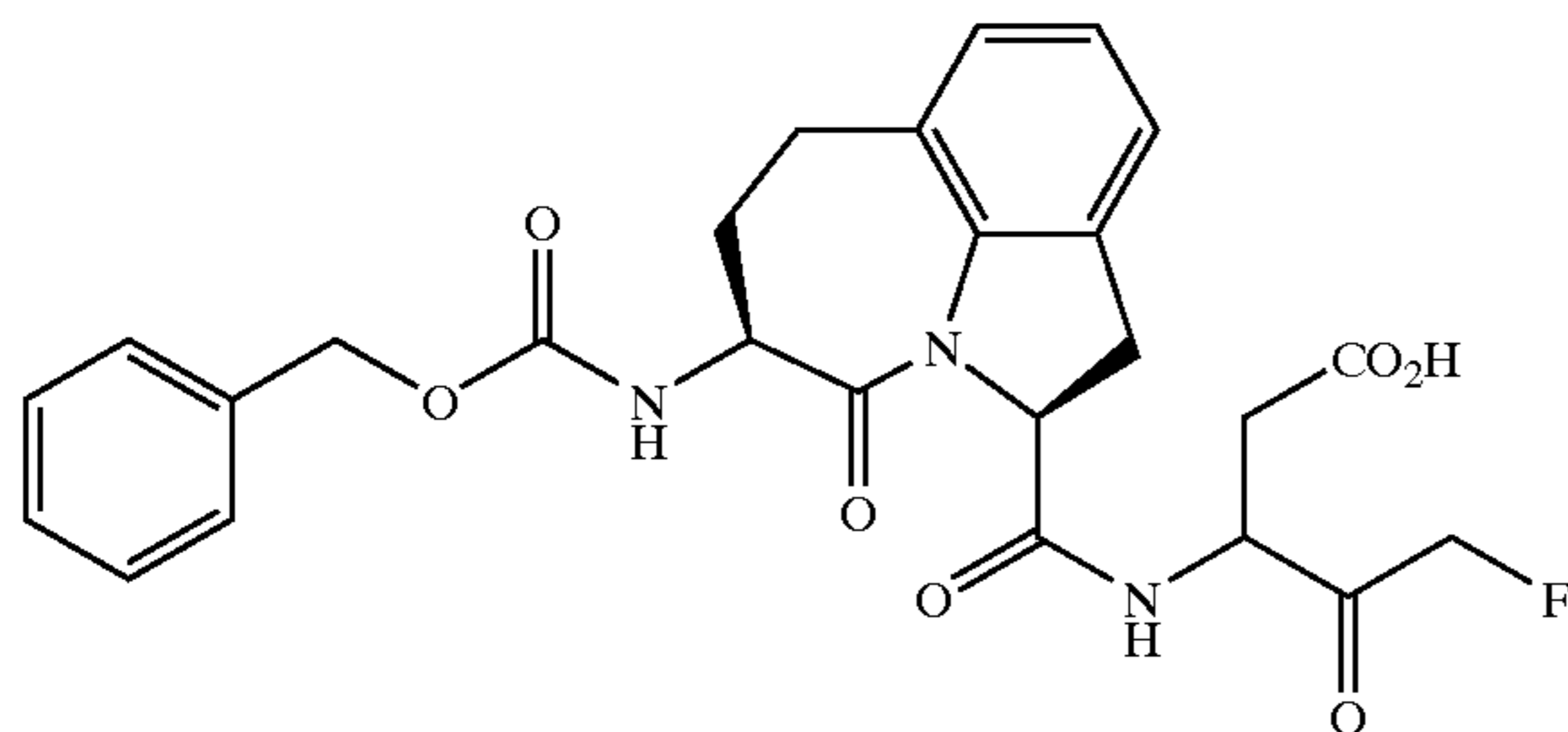
3{(2S-cis)-[5-Benzyloxycarbonylamino-1,2,3,4,5,6,7-hexahydro-4-oxoazepino[3,2,1-hi]indole-2-carbonyl]-amino}-5-fluoro-4-oxo-pentanoic Acid
