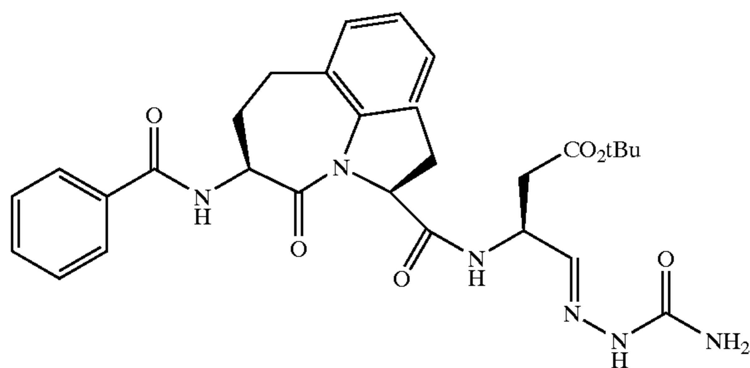
(2S-cis)-[5-Benzoylamino-1,2,3,4,5,6,7-hexahydro-4-oxoazepino[3,2,1-hi]indole-2-carbonyl)-amino]-4-oxo-butanoic Acid tert-Butyl Ester Semicarbazone
