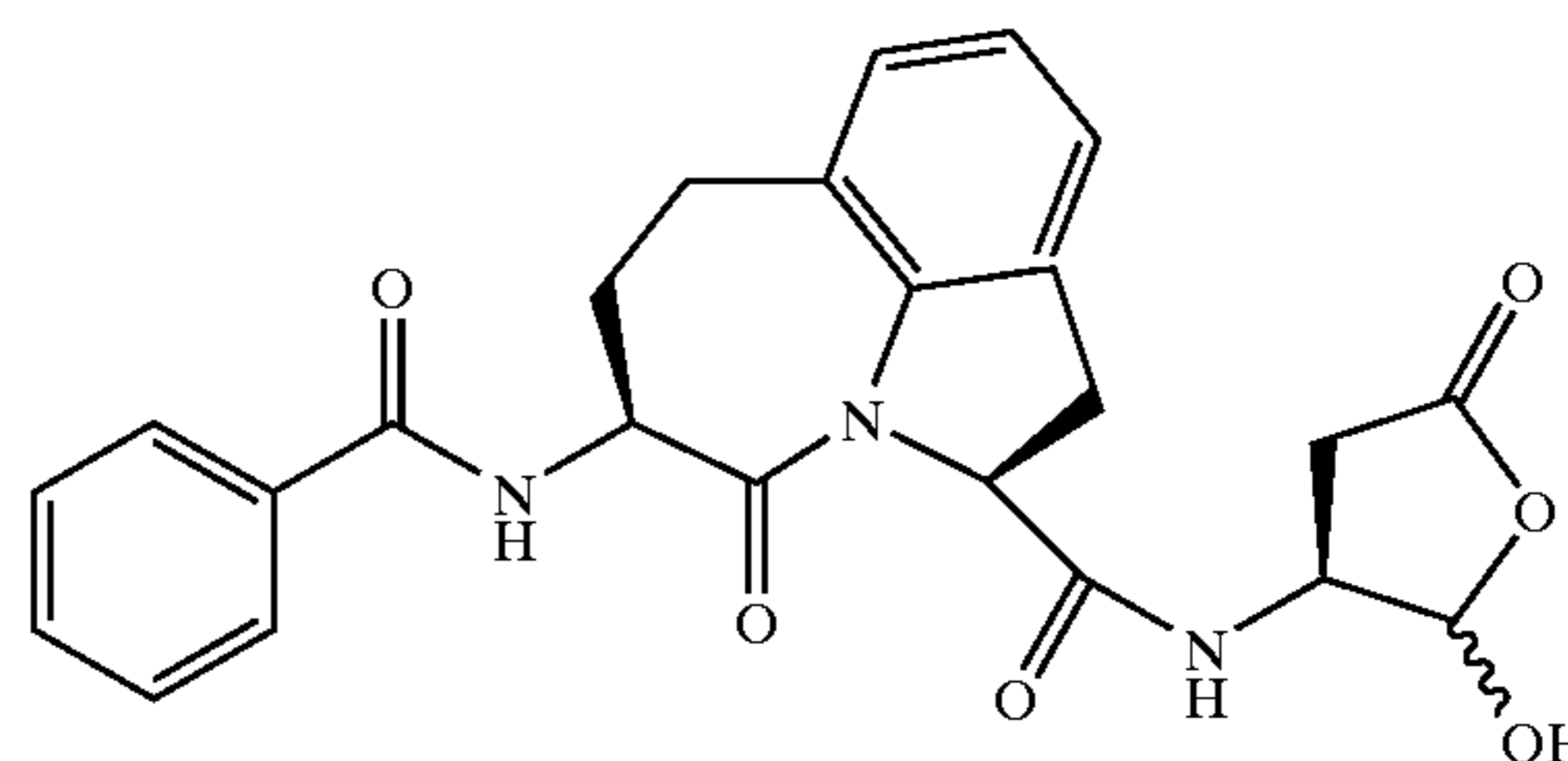
(2S-cis)-[5-Benzoylamino-1,2,3,4,5,6,7-hexahydro-4-oxoazepino[3,2,1-hi]indole-2-carbonyl)-amino]-4-oxo-butanoic Acid
