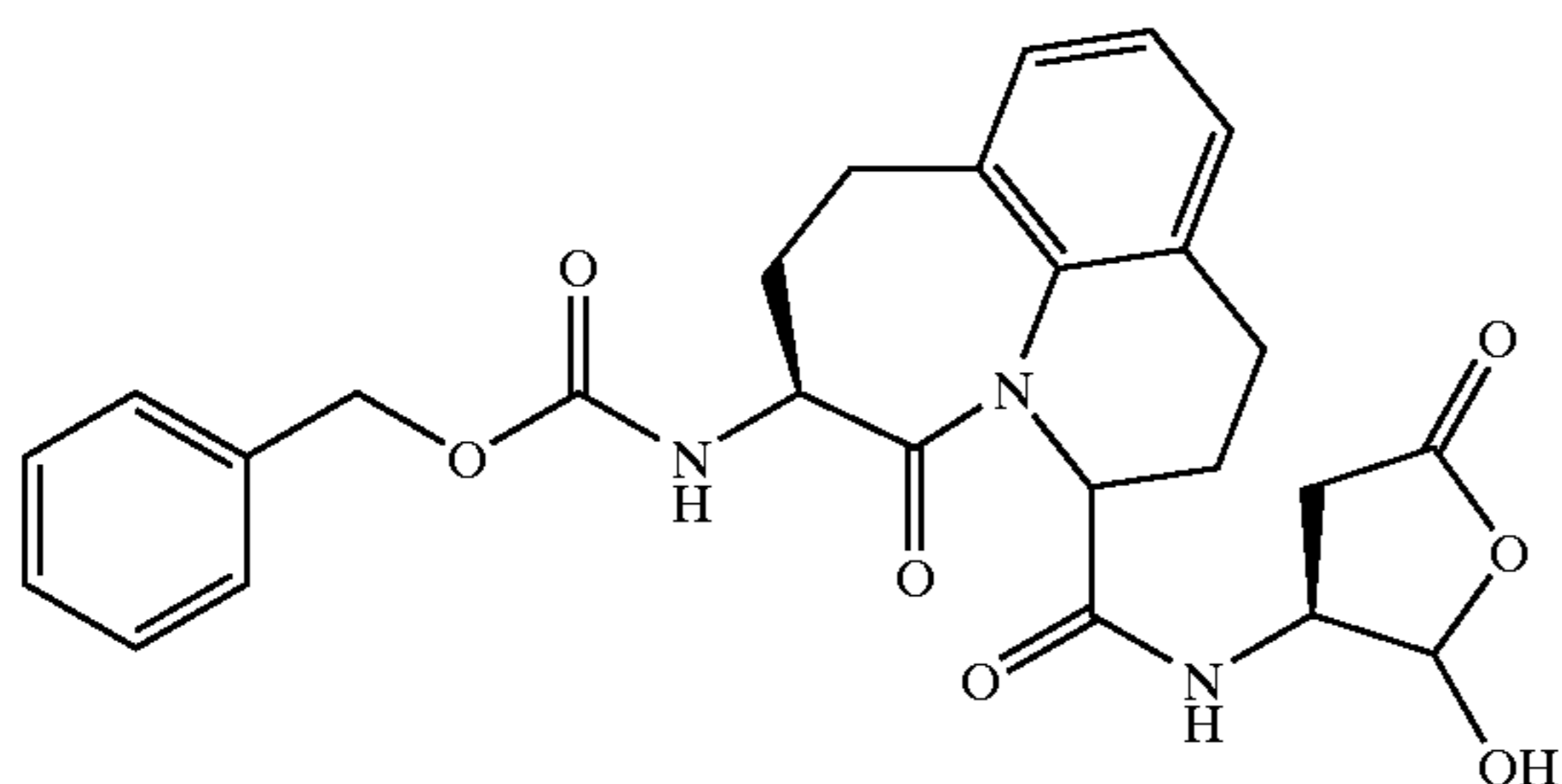
(3R,S-cis)-6-Benzyloxycarbonylamino-5-oxo-2,3,4,5,6,7,8-hexahydro-1H-azepino[3,2,1-hi]quinoline-3-carbonyl)-amino]-4-oxo-butanoic Acid
