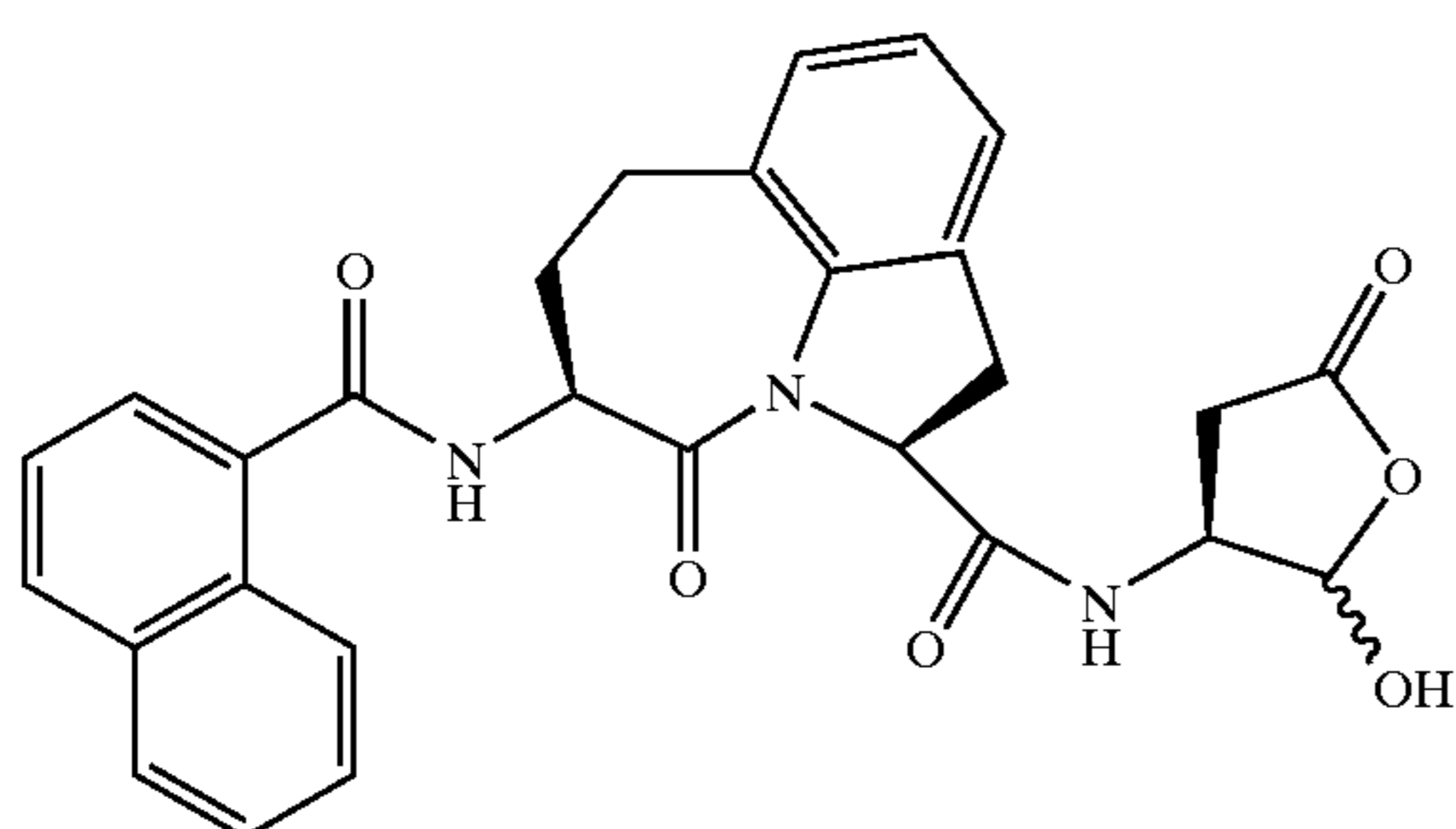
(2S-cis)-[5-(1-Naphthoyl)amino-1,2,3,4,5,6,7-hexahydro-4-oxoazepino[3,2,1-hi]indole-2-carbonyl)-amino]-4-oxo-butanoic Acid
