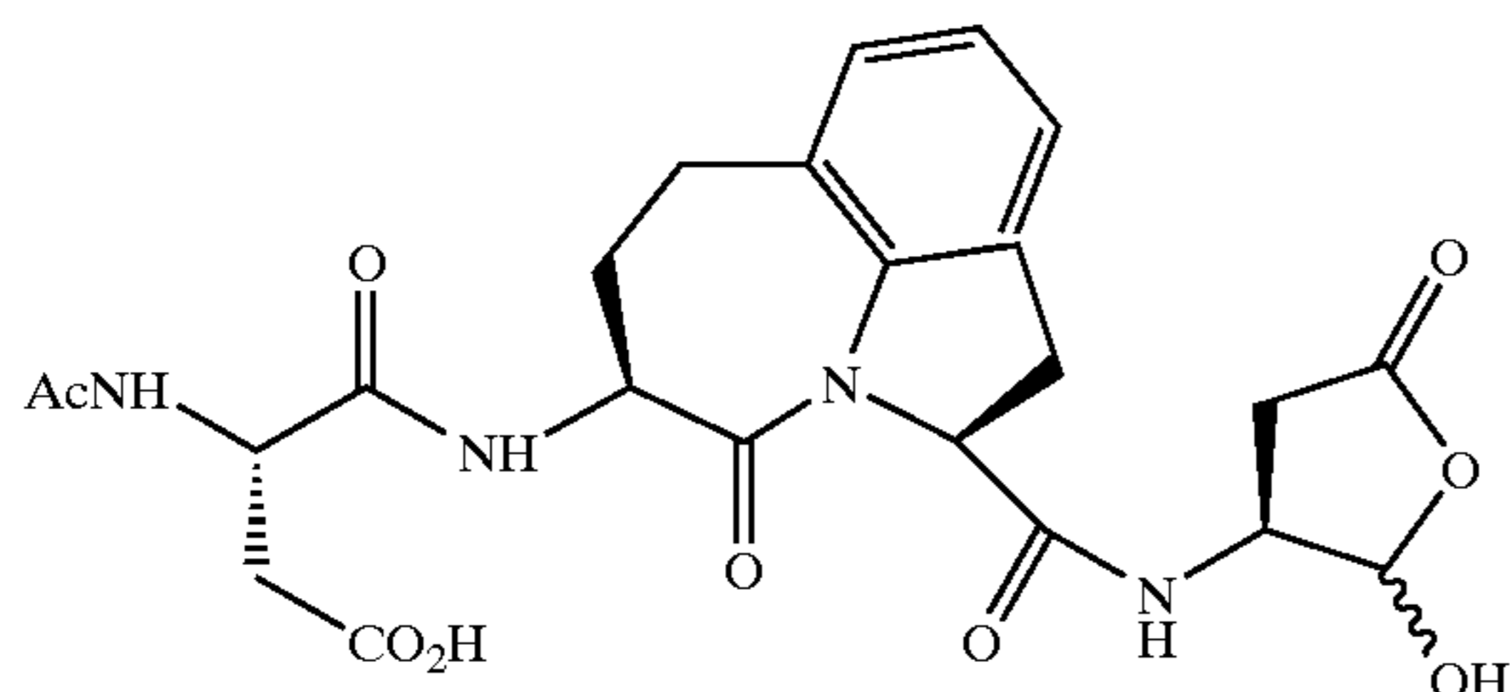
(2S-cis)-[5-(N-Acetyl-(S)-aspartyl)amino-1,2,3,4,5,6,7-hexahydro-4-oxoazepino[3,2,1-hi]indole-2-carbonyl)-amino]-4-oxo-butanoic Acid
