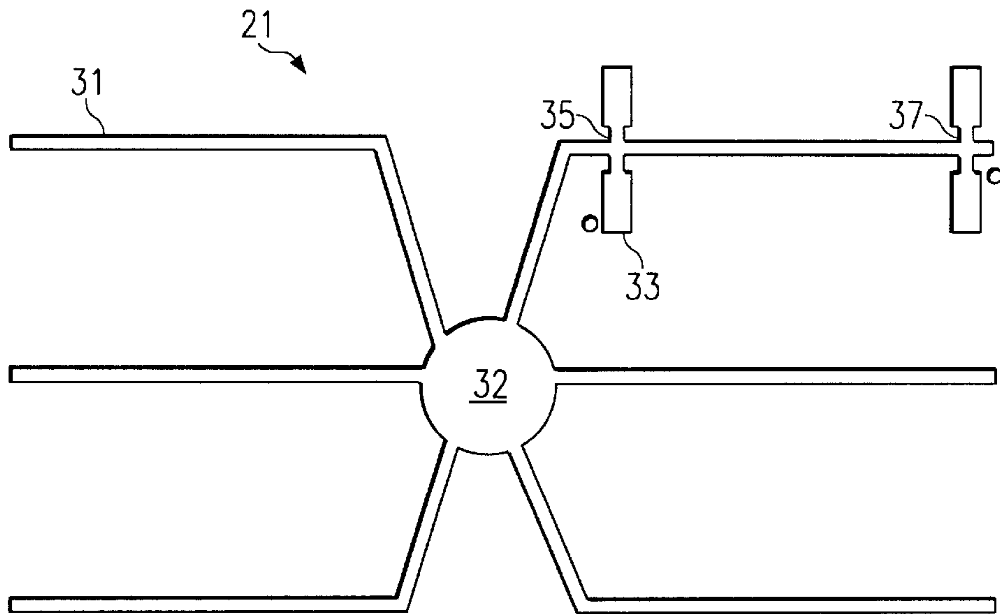
FIG. 3 (PRIOR ART)
