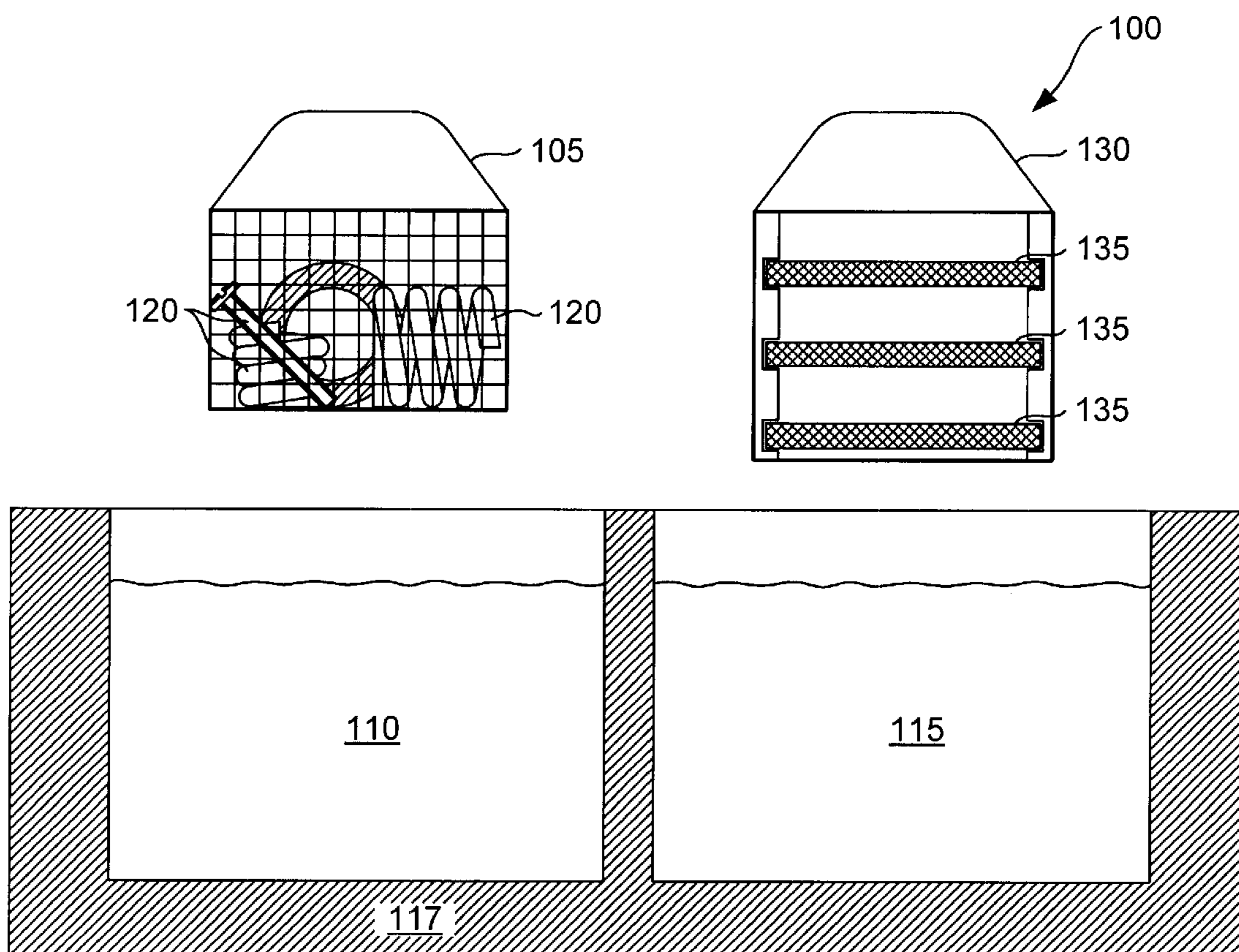
FIG. 1 (PRIOR ART)
