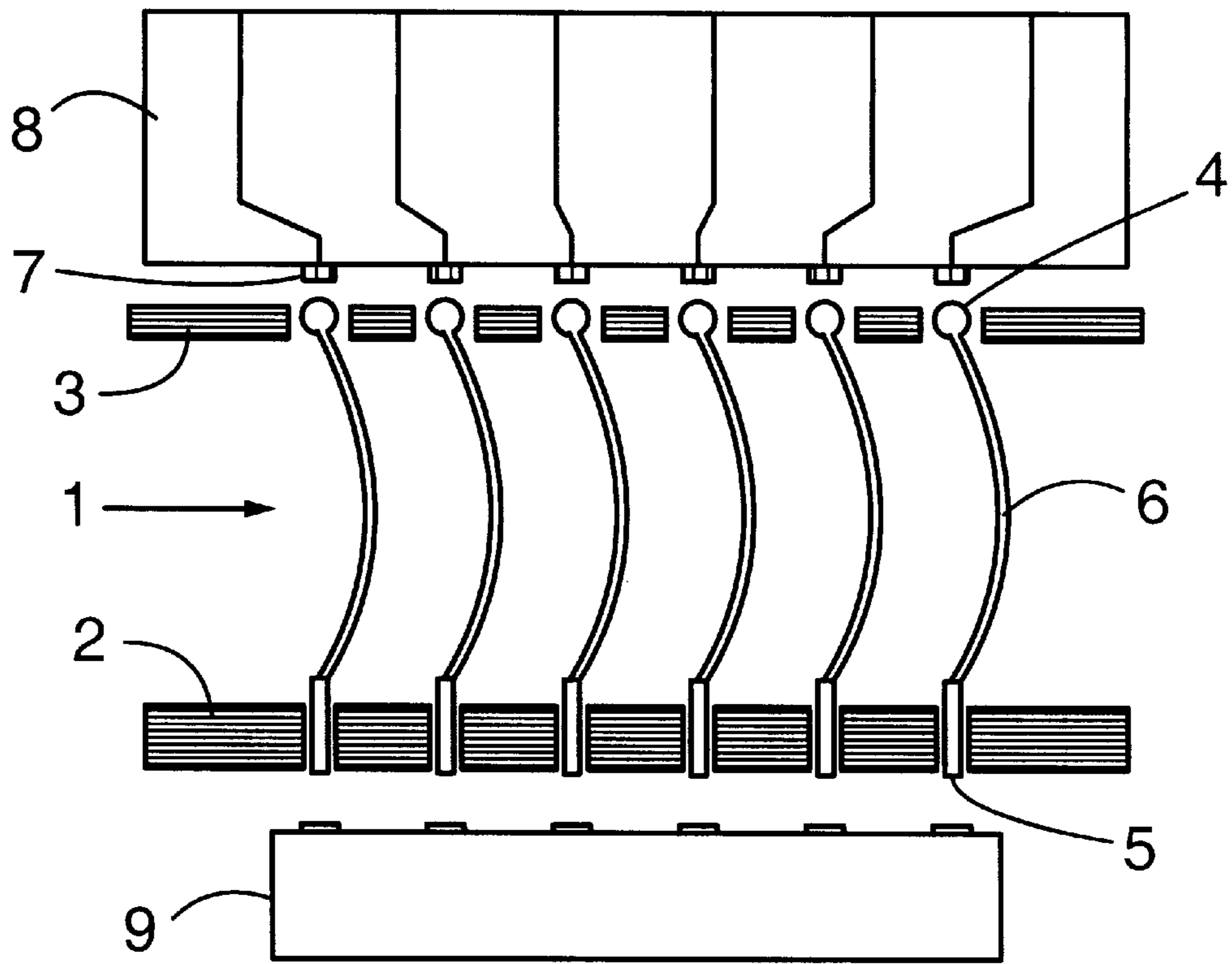
Fig. 1 (Prior Art)
