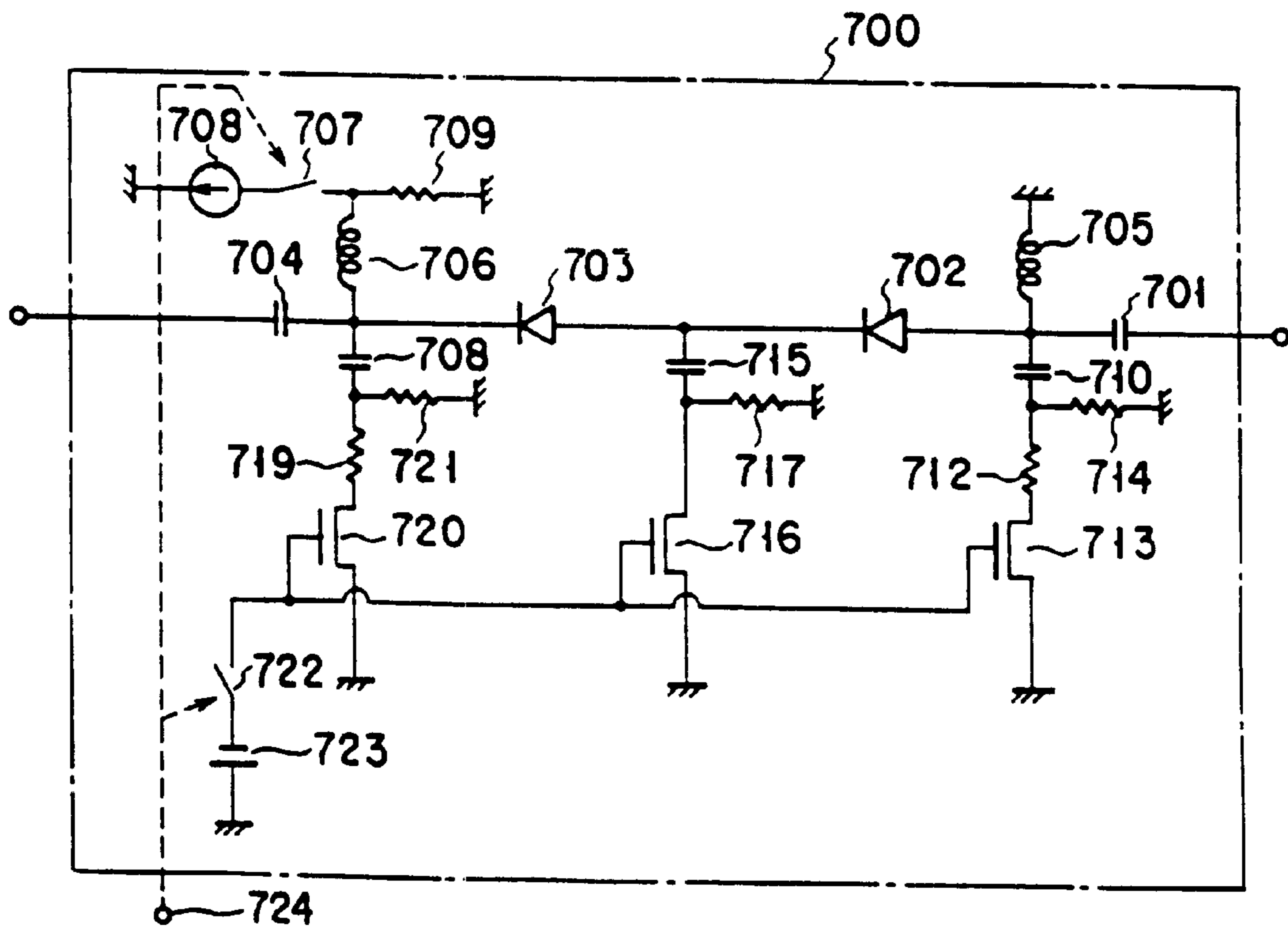
FROM TRANSMISSION DISPLAY SIGNAL DETECTION CIRCUIT
