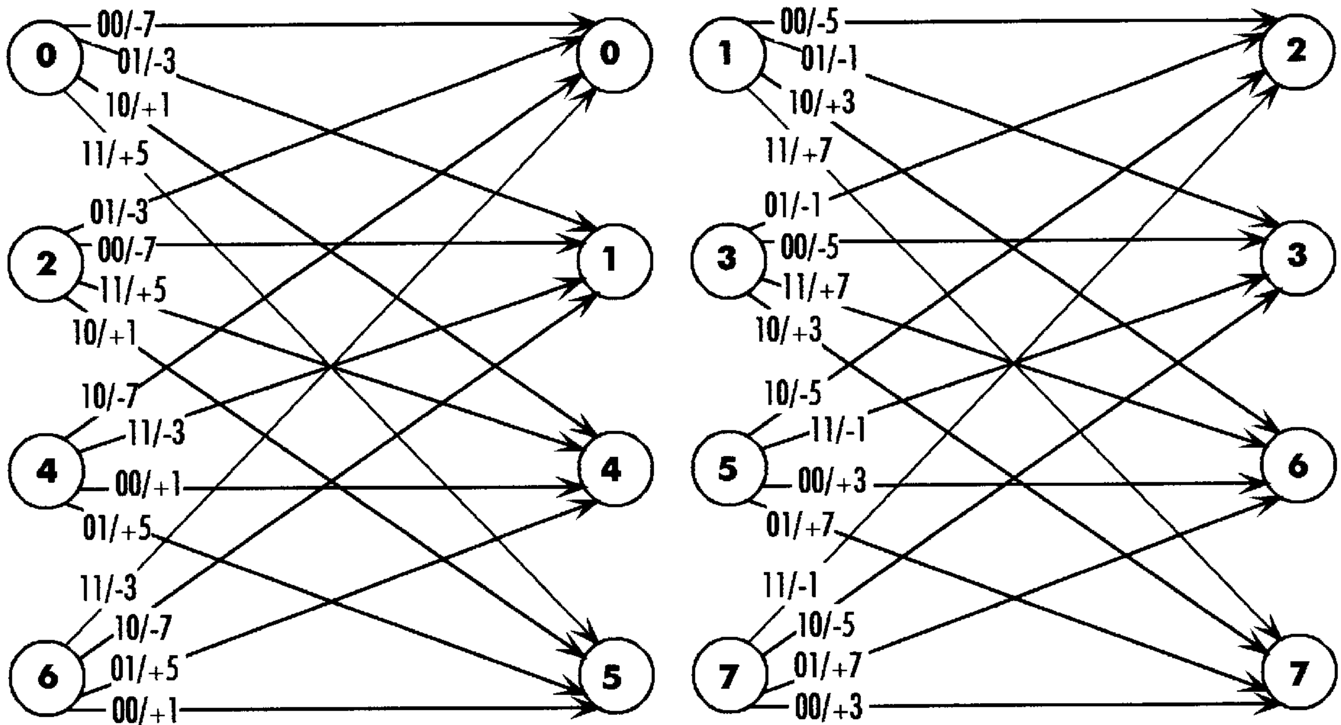
TCM Encoder State Diagram
