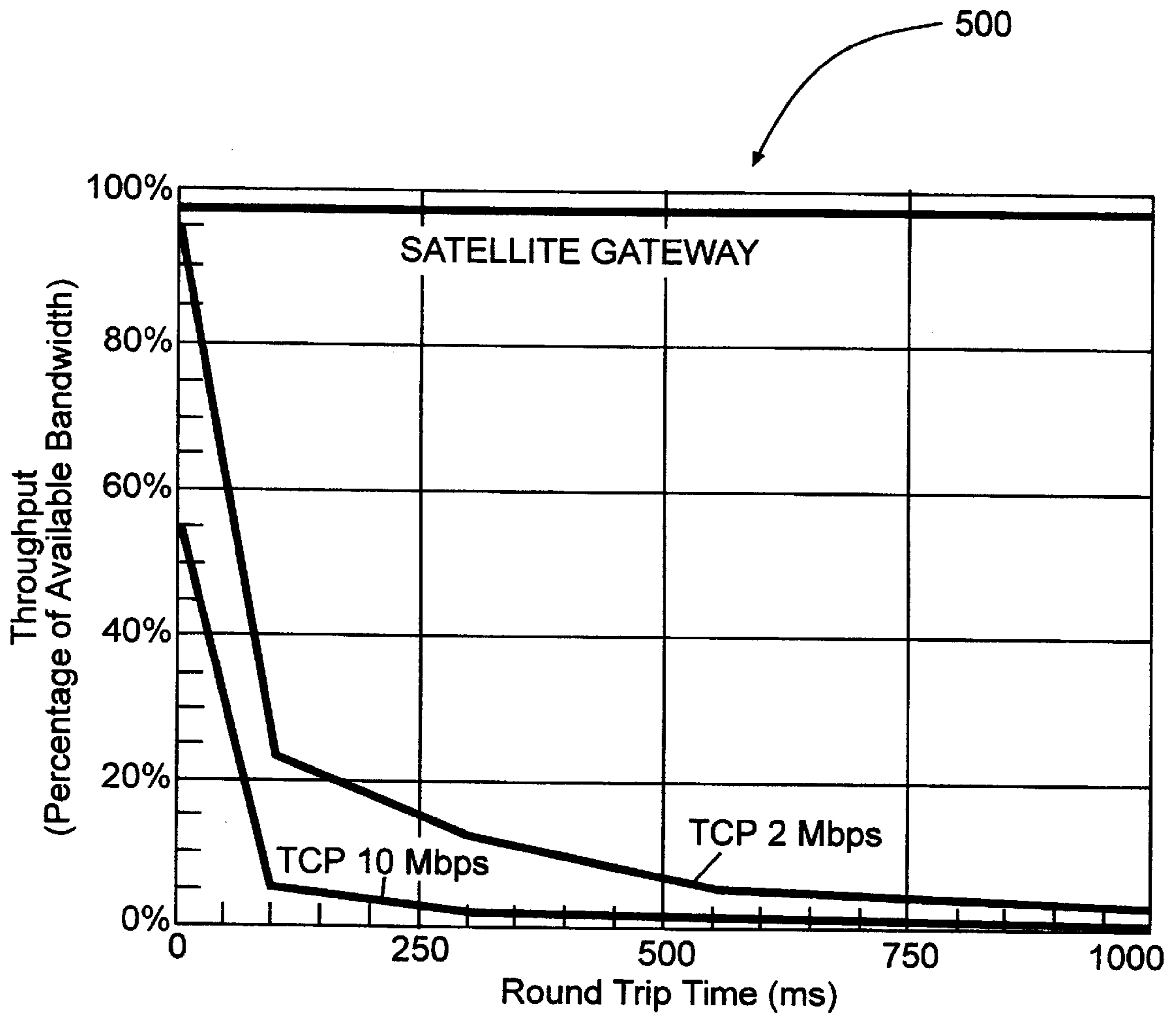
Delay vs. Throughput
