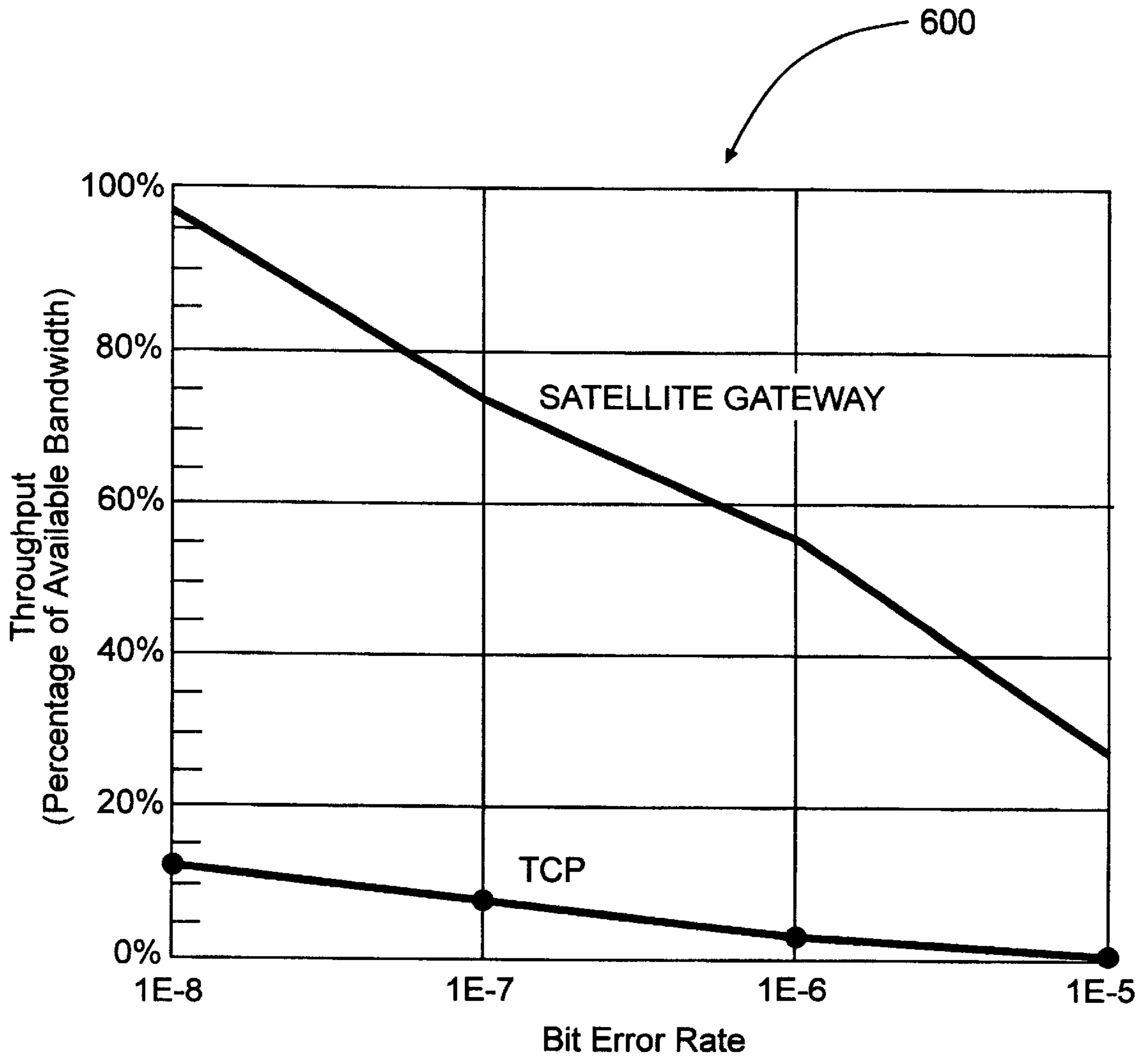
Bit Error Rate vs. Throughput (10Mbps Link)
